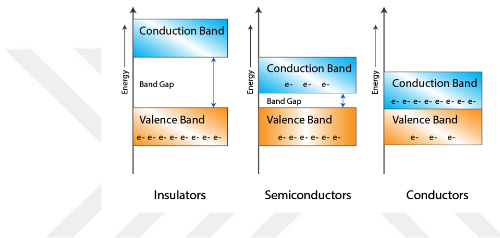
Figure 2.2. Band structures for insulators, semi-conductors and conductors.
