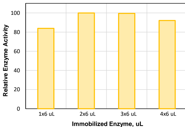
Figure 4.6. Effect of enzyme amount on activity.
