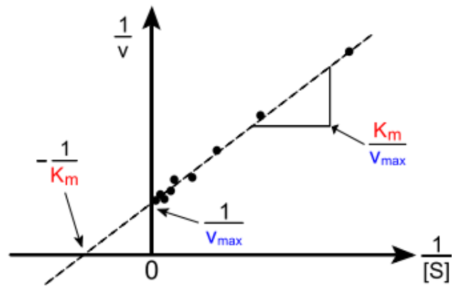
Figure 2.15. Lineweaver-Burk graph [13].
