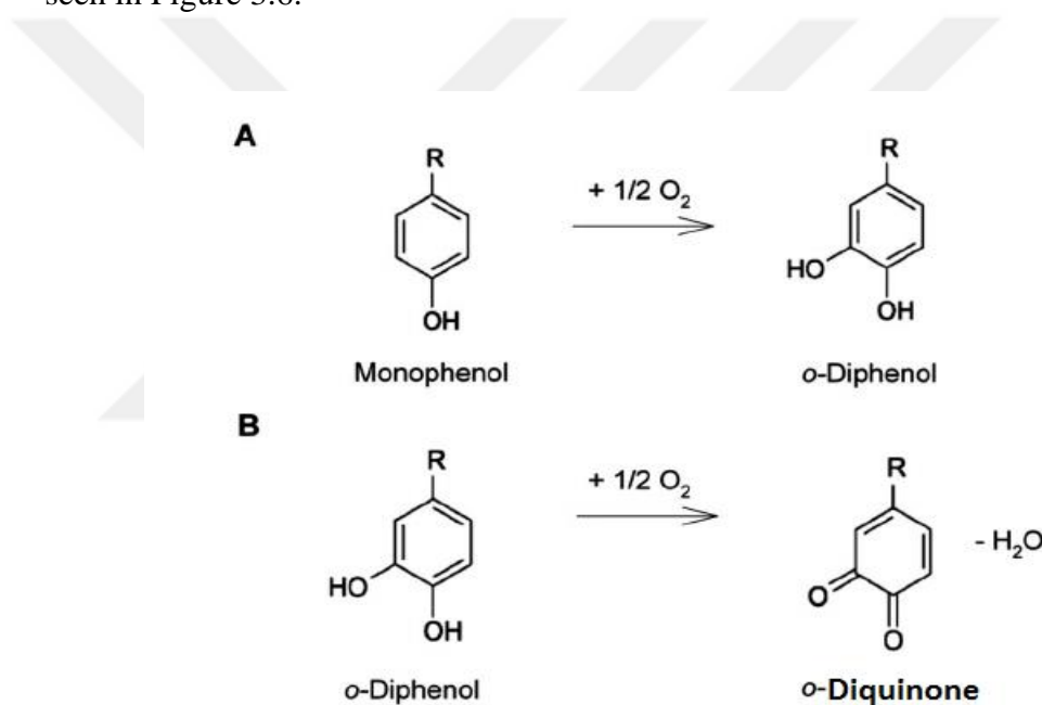
Figure 3.6. PPO's cresolase and catecholase activities: A) monophenol's o -hydroxylation, B) oxidation of o -diphenol to o -quinone.
