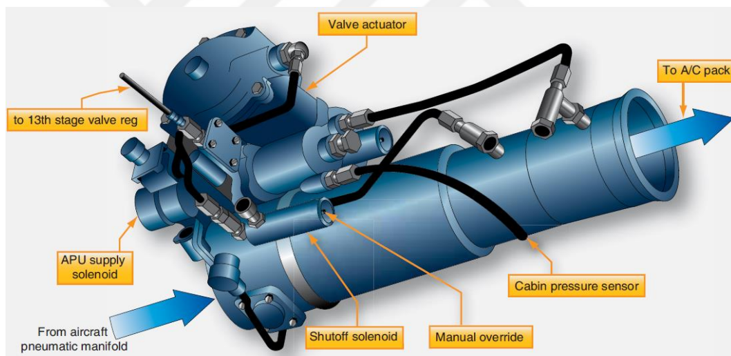
Figure 3.4. Pack valve [8].
