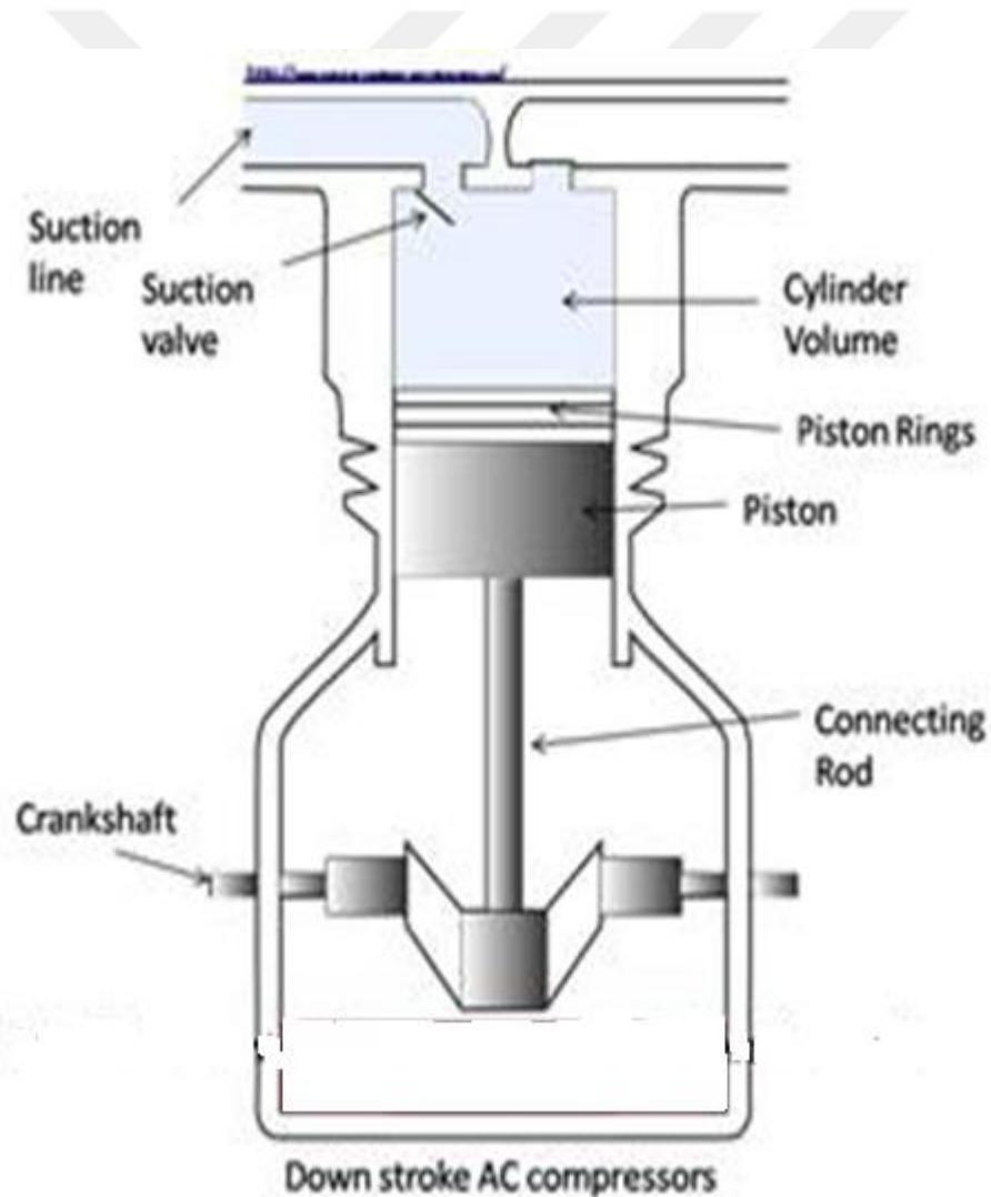
Figure 3.14. Compressor [10].
