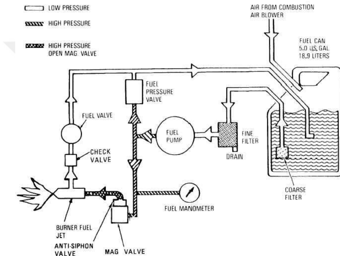
Figure 3.24. Heater fuel system [11].
