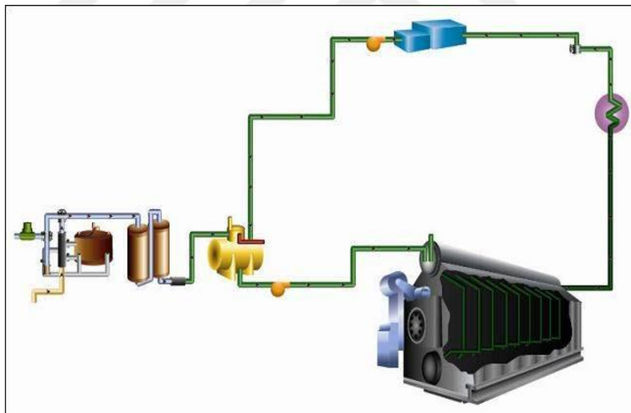
Figure 2.4. Boiler system [25].
