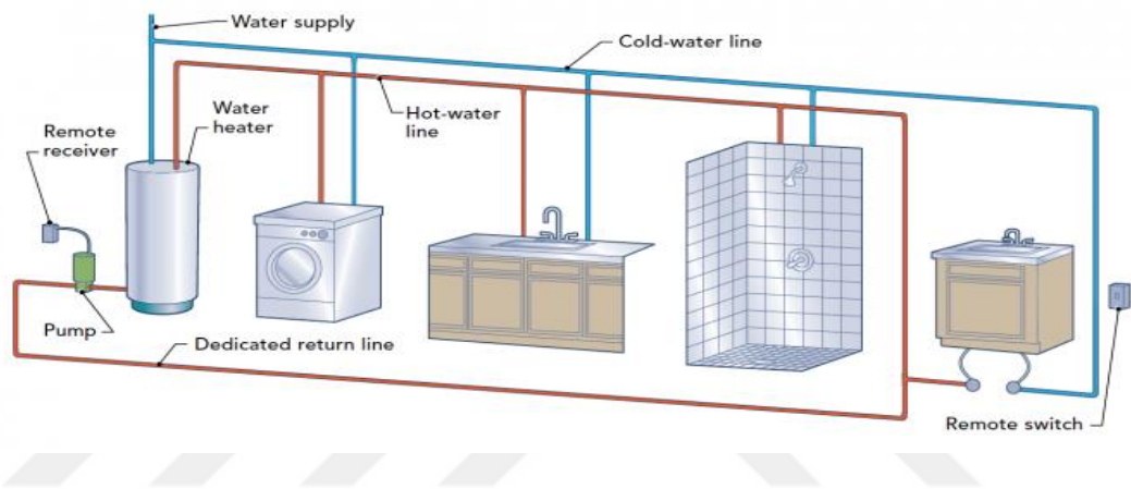
Figure 2.9. Hot water system [28].
