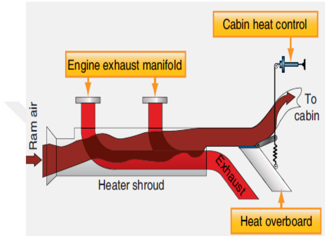
Figure 3.18. The simplest type of heating system [1].
