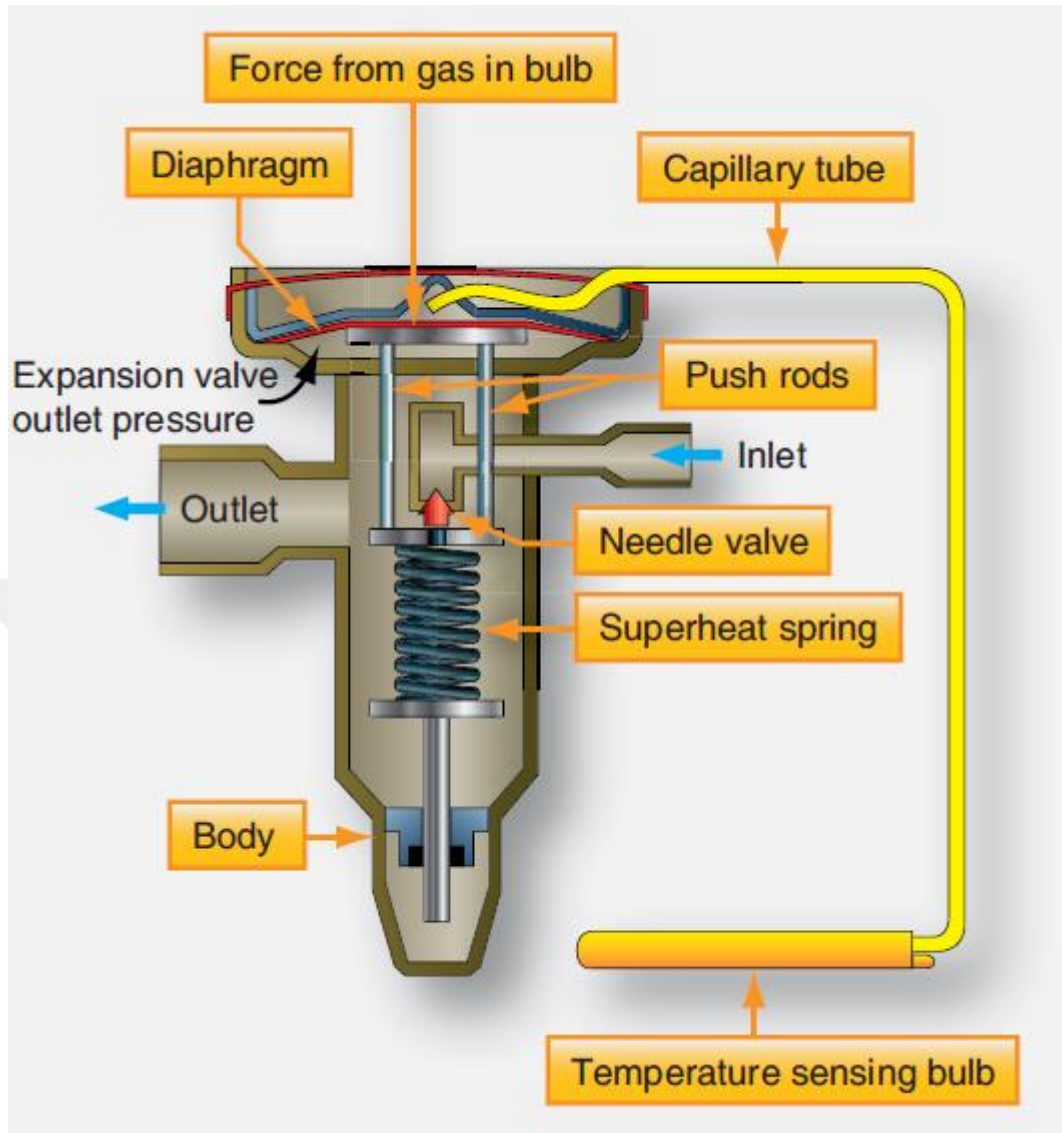
Figure 3.12. Expansion valve [10].
