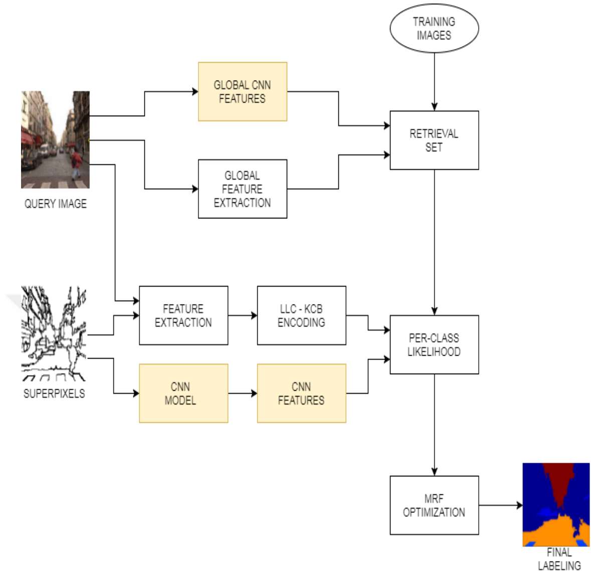
Figure 4.1: System Overview of CNN Models
