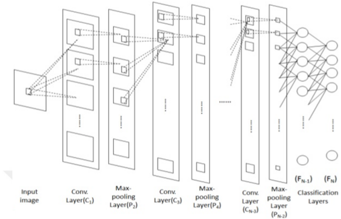
Figure 4.2: System Overview of Convolutional Neural Network Layers [27]
