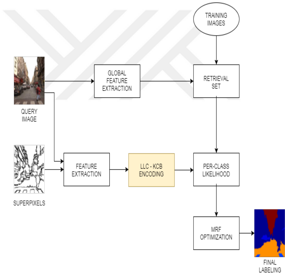
Figure 3.1: System Overview of Feature Encoding Methods
