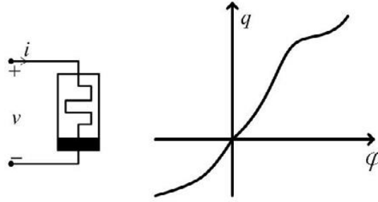
Figure 1.3: Symbol of memristor and its \varphi - q characteristic
