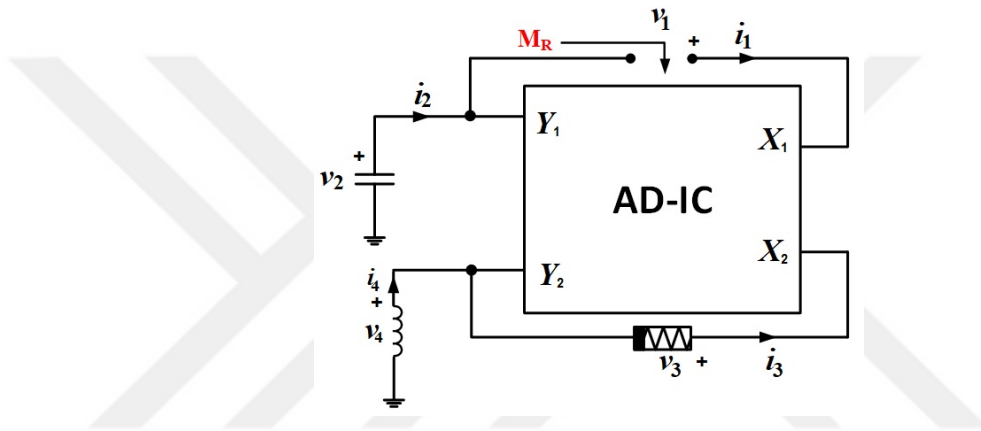
Figure 4.1: Memristor realization with AD-IC based metamutator
