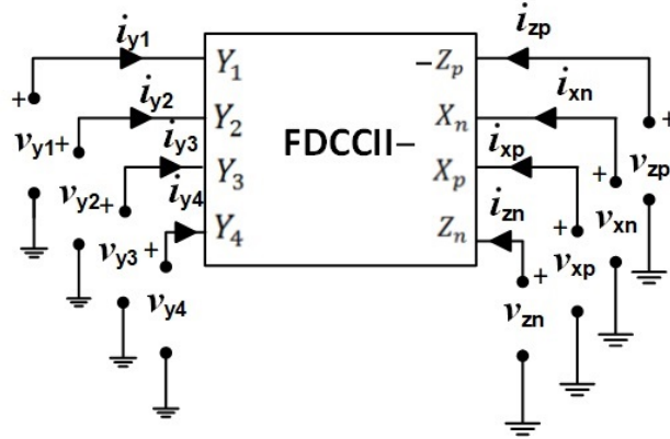
Figure 3.32: Block diagram of FDCCII-
