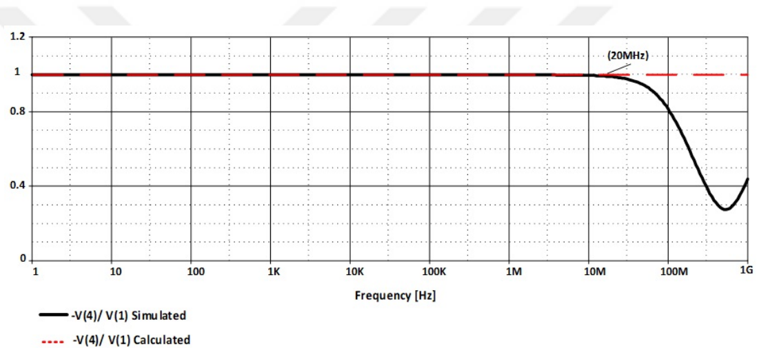
Figure 3.15: Theoretical and simulation characteristics of v_4 vs. v_1
