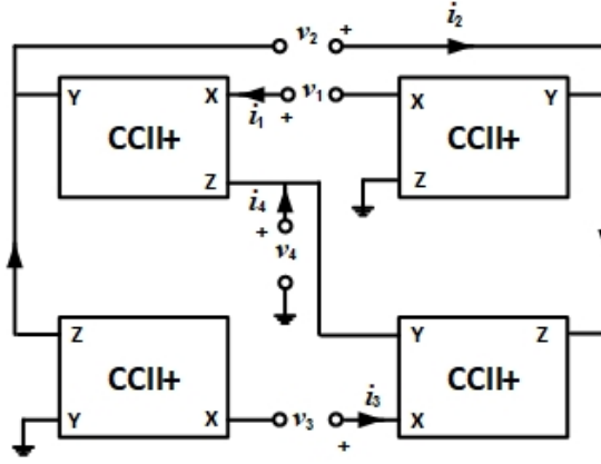
Figure 3.18: Diagram of metamutator extracted from [82]
