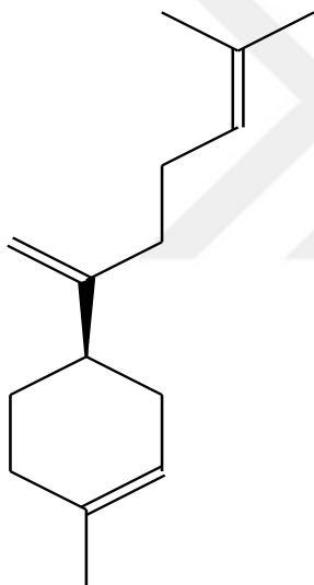
\beta -Bisabolen(PcÇ)
