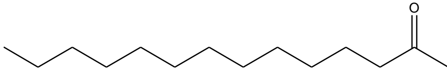
2-Tetradekanon(PcÇ)
