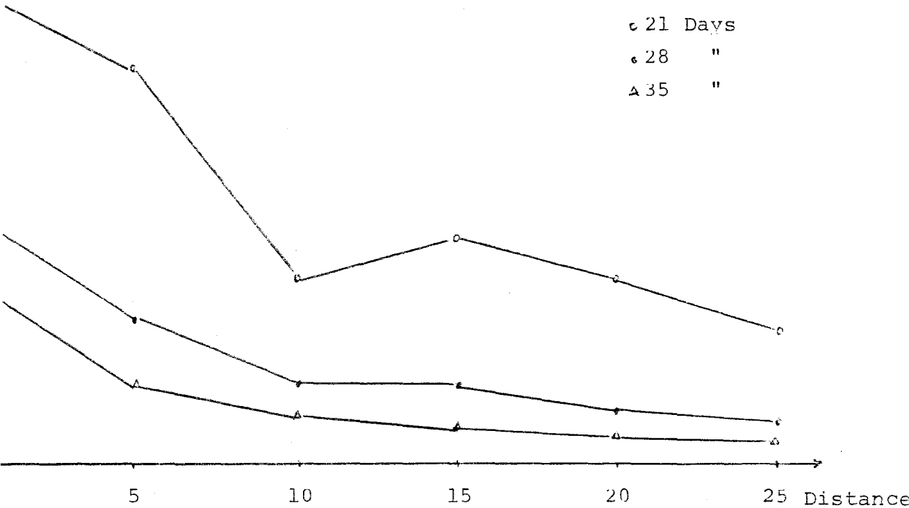
Figure 48 : Variation of Turbidity with Distance in the Channel Full with Sand
