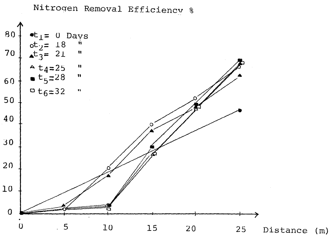
Figure 28 : The Removal Efficiency of Nitrogen with Distance in the Channel Full with Sand
