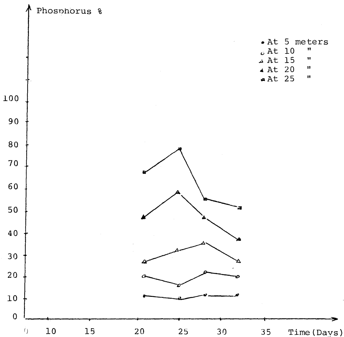
Figure 39 : Removal Efficiency of Phosphorus with Time in the Channel Full with Sandal
