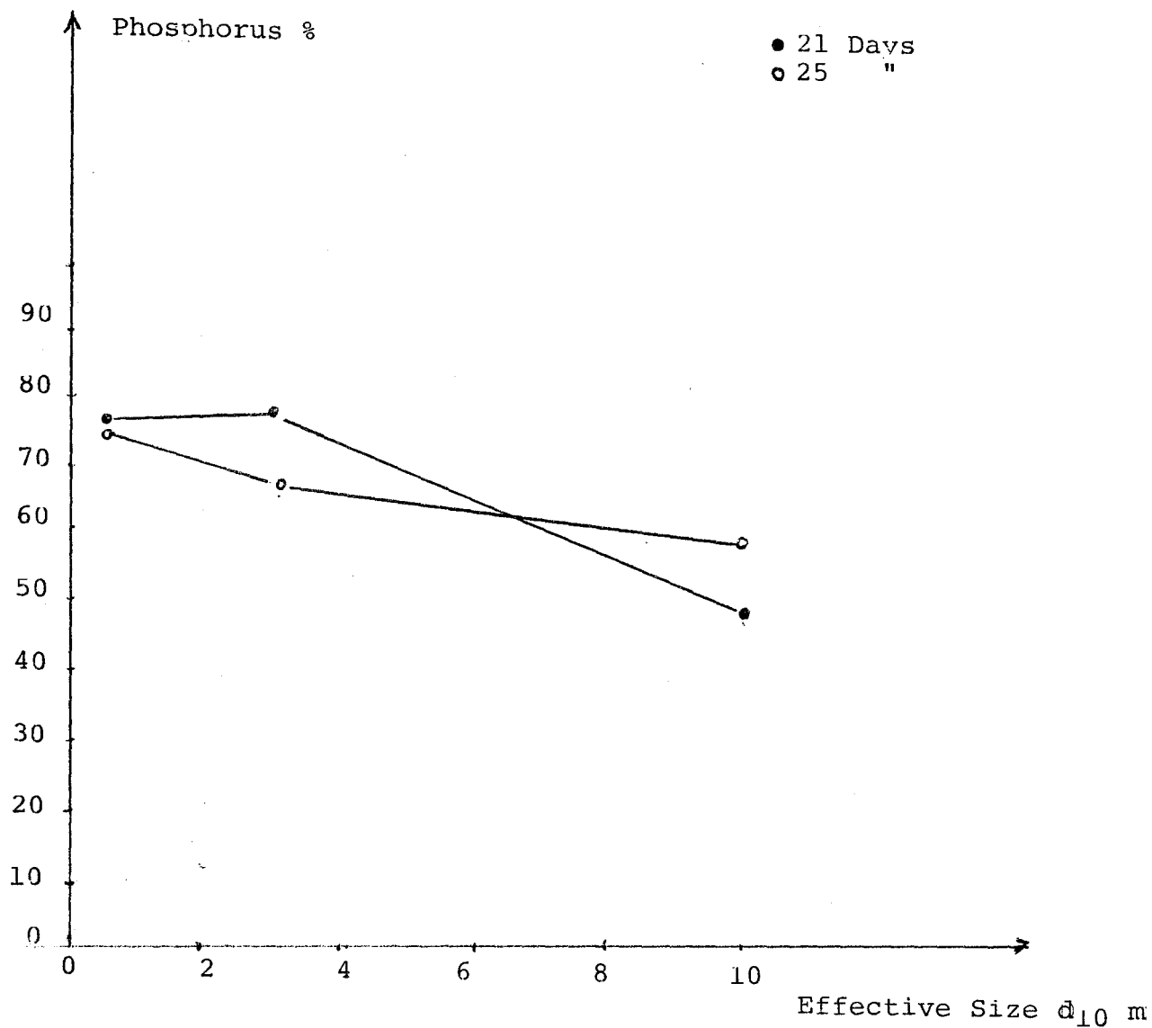
Figure 44 : Removal Efficiency of Phosphorus with Effective Size of Porous Media
