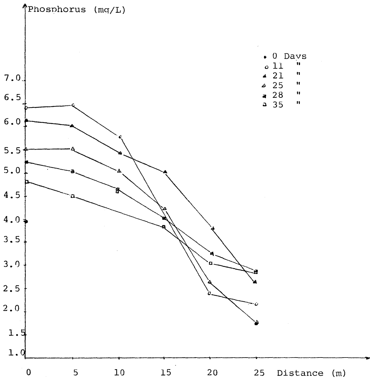
Figure 40 : Variation of Phosphorus with Distance in the Channel Full with Gravel
