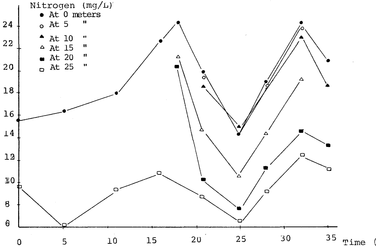
Figure 32 : Graphical Presentation Showing the Variation of Nitrogen with Time in the Channel Full with Gravel
