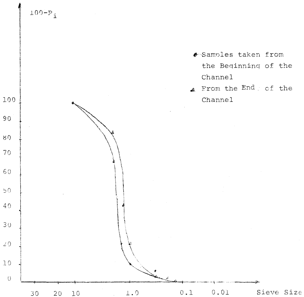
Figure 15 : The Granulometric Curves of Gravel Sample
