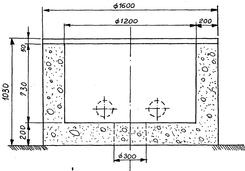
Section B-B
