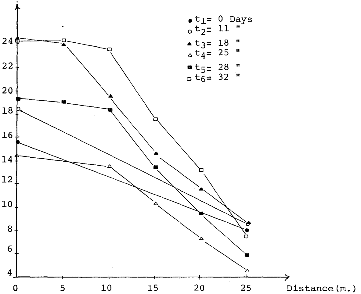
Figure 29 : Graphical Presentation Showing the Variation of Nitrogen with Distance in the Channel Full with Sand
