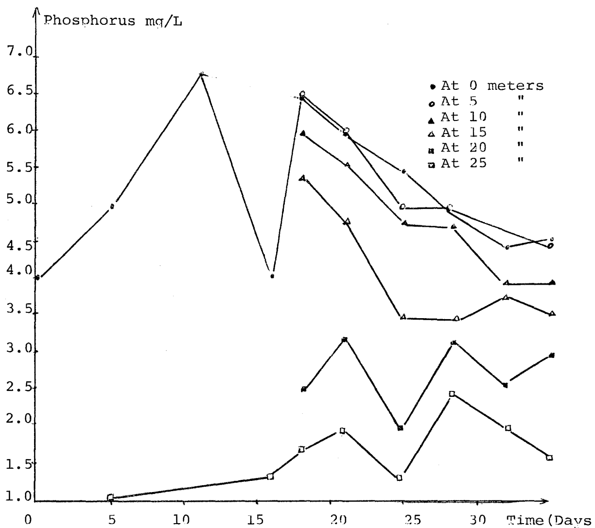
Figure 38 : Variation of Phosphorus with Time in the Channel Full with Sand
