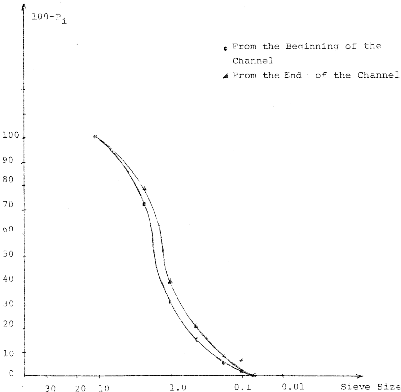
Figure 14 : The Granulometric Curves of Sand Samples
