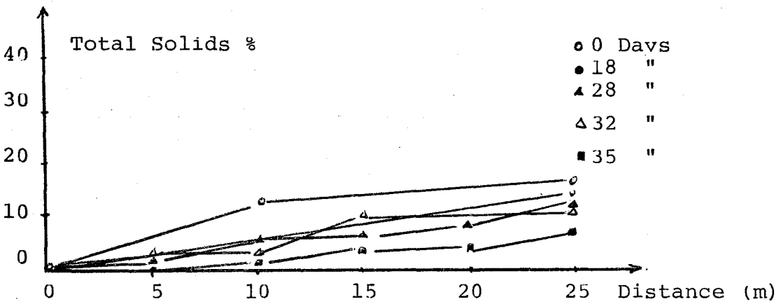
Figure 45 a :Removal Efficiency of Total Solids in the Channel Full with Gravel b :Removal Efficiency of Total Solids in the Channel Full with Sand
