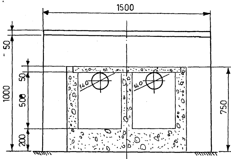
Section C-C'
