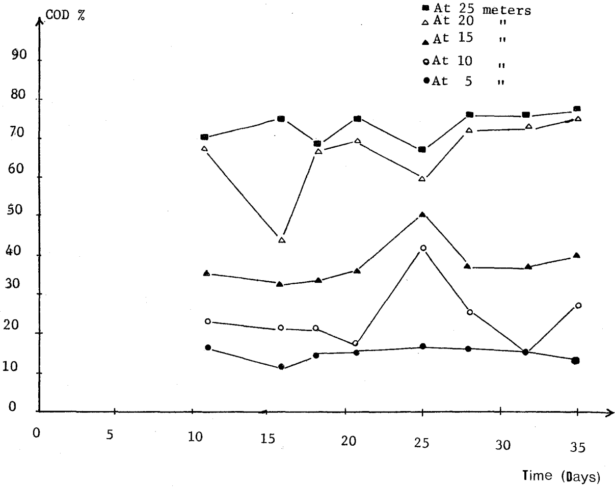
Figure 20 : Graphical Presentation Showing the Removal Efficiency of COD with Time in the Channel Full with Sand
