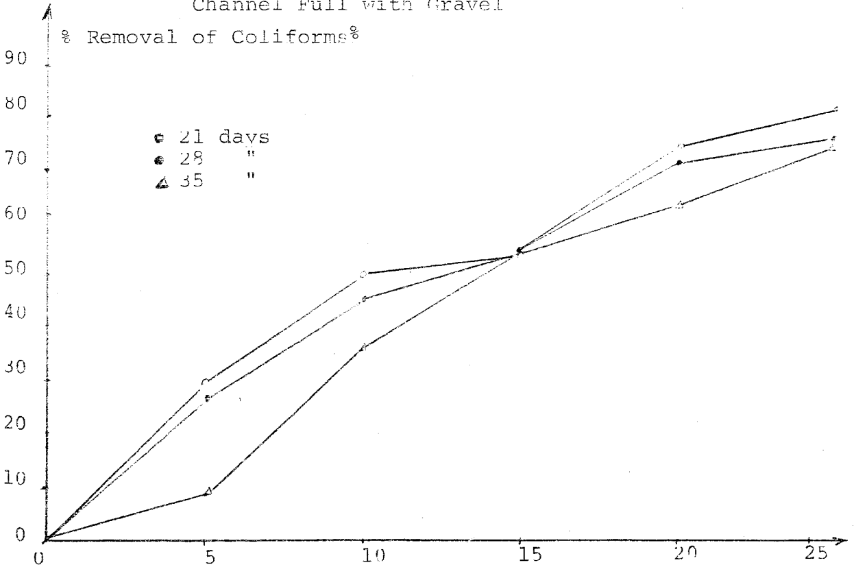
Figure 60 : The Removal Efficiency of Coliform with Distance in the Channel Full with Gravel
