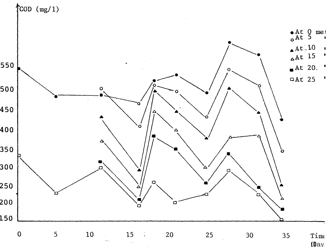
Figure 22 : Graphical Presentation Showing the Variation of COD w Time in the Channel Full with Gravel
