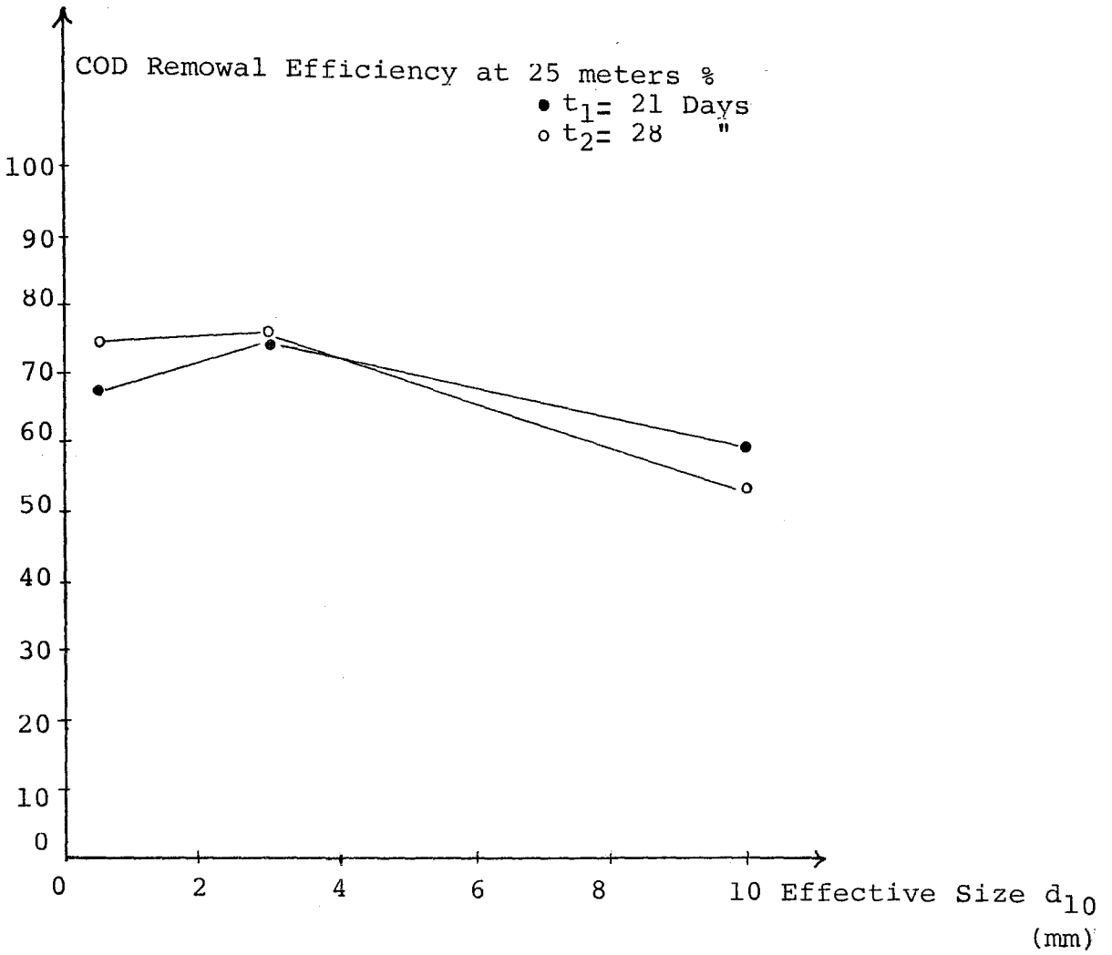
Figure 26 : Graphical Presentation Showing Variations of COD Removal Efficiency with Effective Size of Porous Media (at 25 meters)
