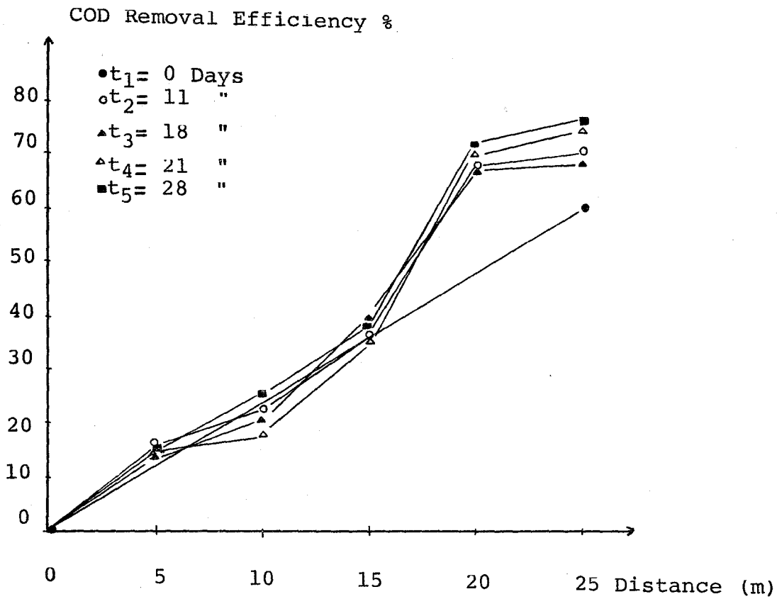
Figure 19 : The Removal Efficiency of COD with Distance in the Channel Full with Sand
