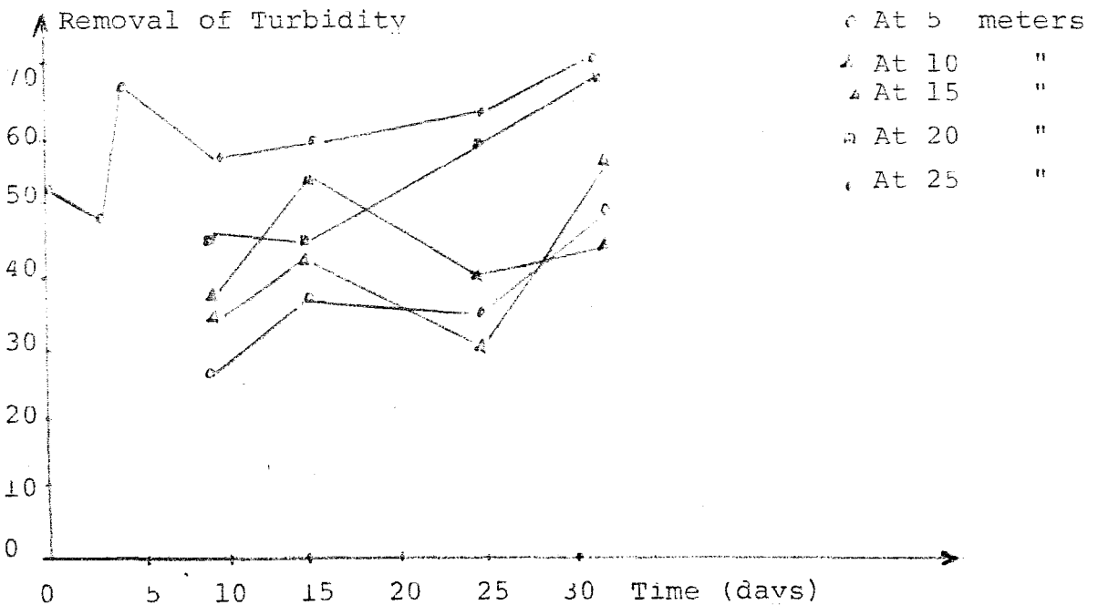
Figure 51 : Removal Efficiency of Turbidity with Time in the Channel Full with Gravel
