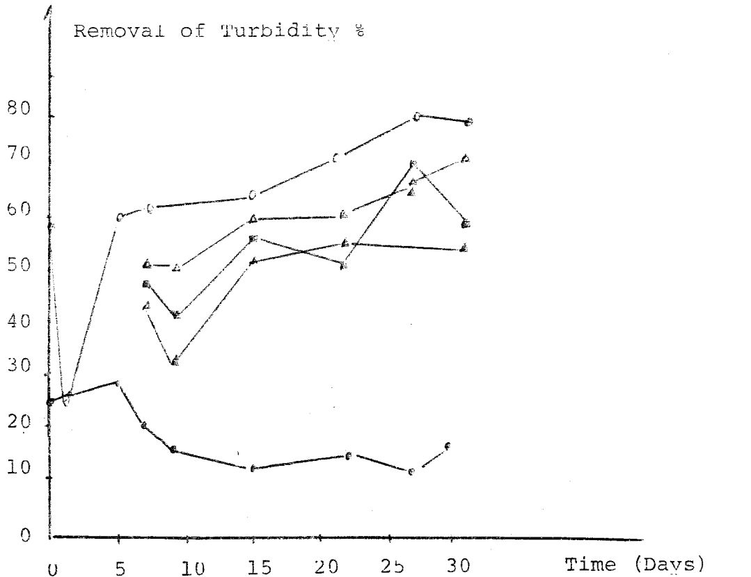
Figure 47 : Removal of Turbidity with Time in the Channel Full with Sand
