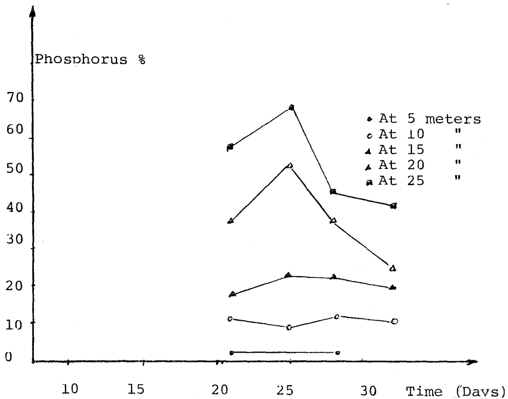
Figure 41 : Removal Efficiency of Phosphorus with Time in the Channel Full with Gravel
