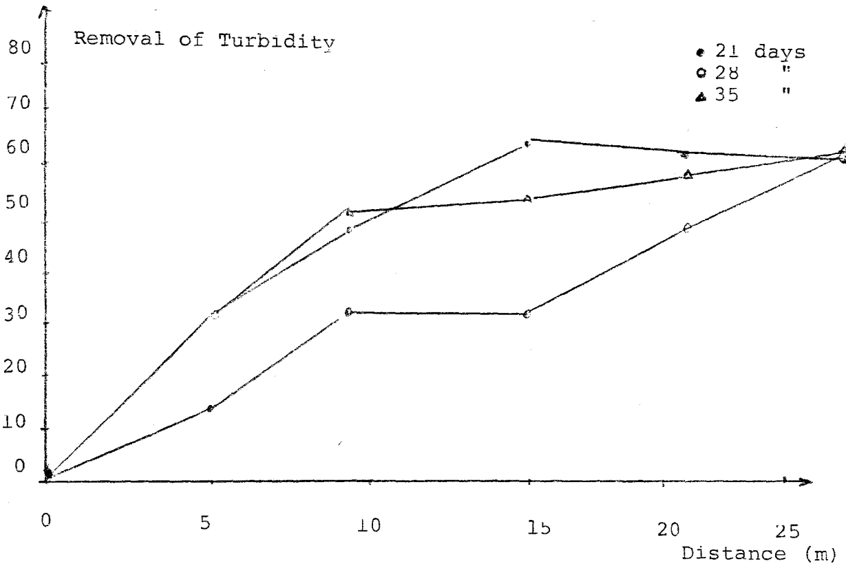
Figure 53 : Removal Efficiency of Turbidity with Distance in the Channel Full with Gravel
