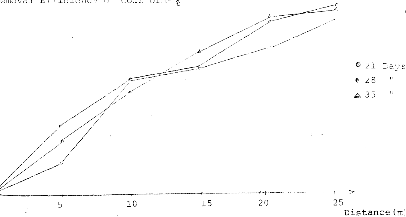
Figure 58 : Removal Efficiency of Coliform with Distance in Sand Bed
