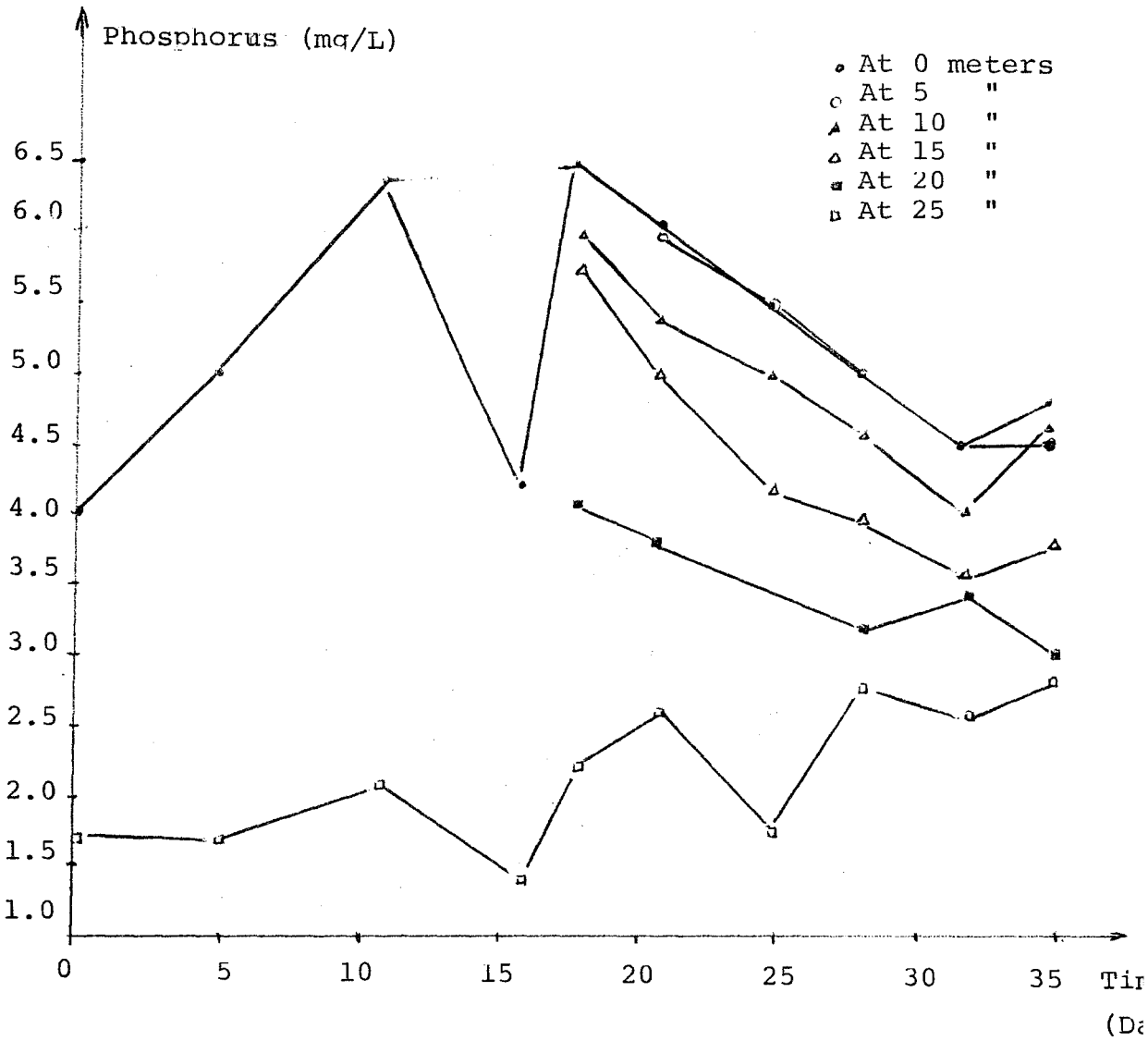
Figure 43 : Variation of Phosphorus with Time in the Channel Full with Gravel
