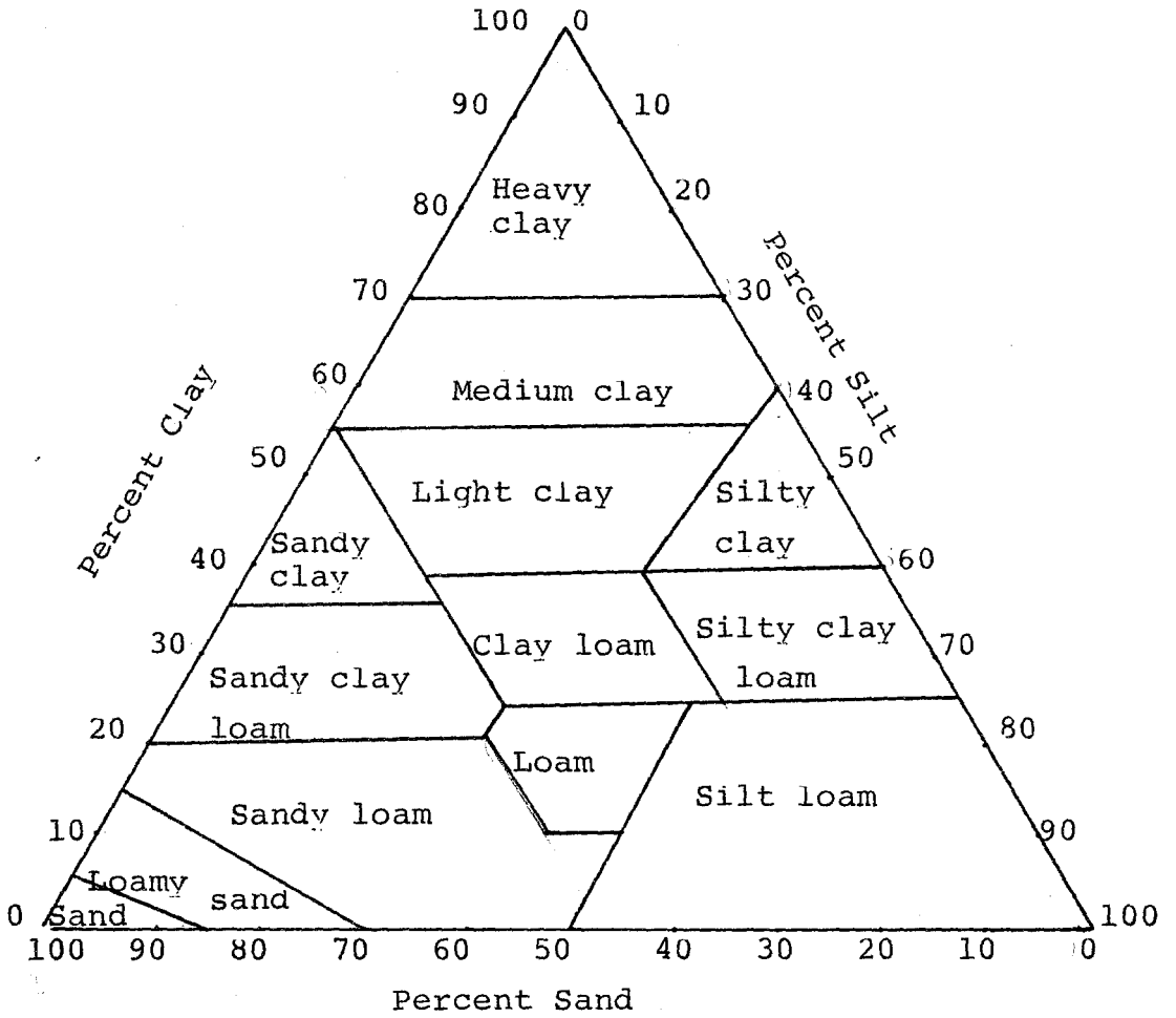
Figure 3 : Textural Classes (Crites,1984)
