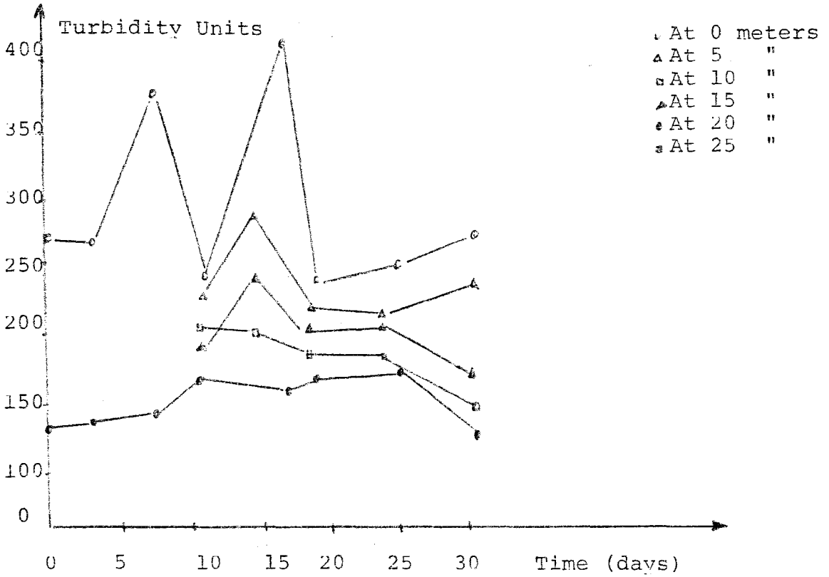
Figure 50 : Variation of Turbidity with Time in the Channel Full with Gravel
