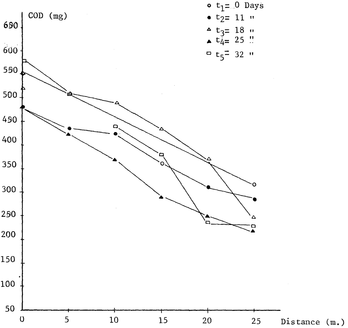
Figure 25 : Graphical presentation Showing the Variation of COD with Distance in the Channel Full with Gravel
