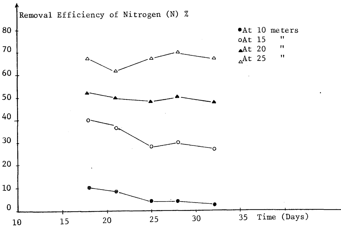
Figure 30 : Graphical Presentation of the Removal Efficiency of Nitrogen with Time in the Channel Full with Sand
