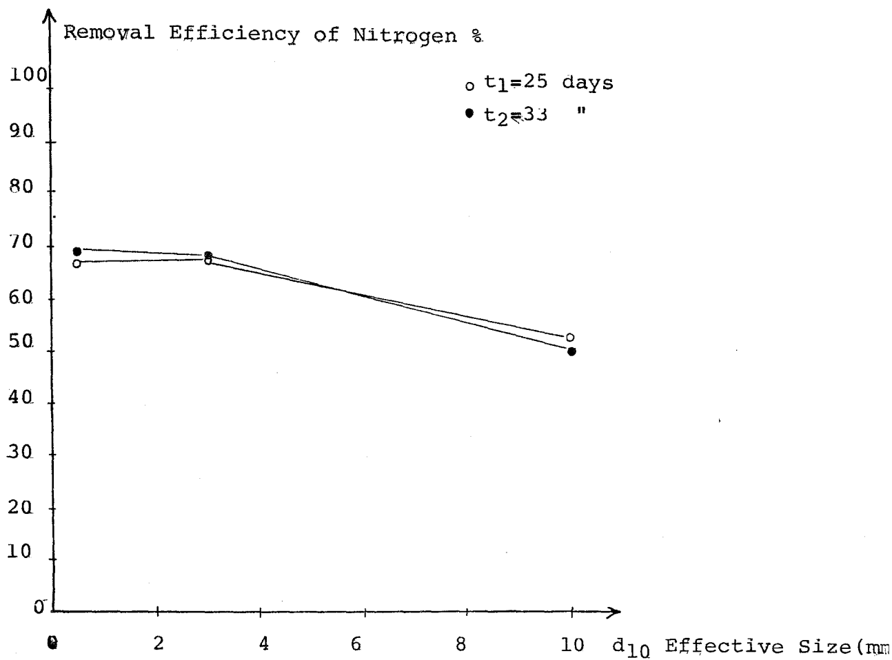
Figure 35 : Graphical Presentation Showing th Removal Efficiency of Nitrogen with the Effective Size
