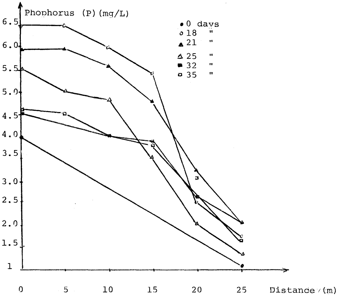
Figure 36 : Variation of Phosphorus with Distance in the Channel Full with Sand
