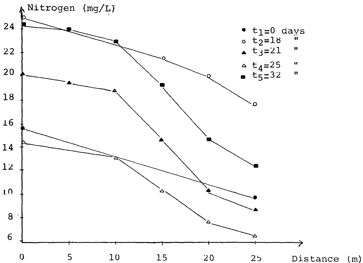
Figure 34 : Graphical Presentation Showing the Variation of Nitrogen with Distance in the Channel Full with Gravel
