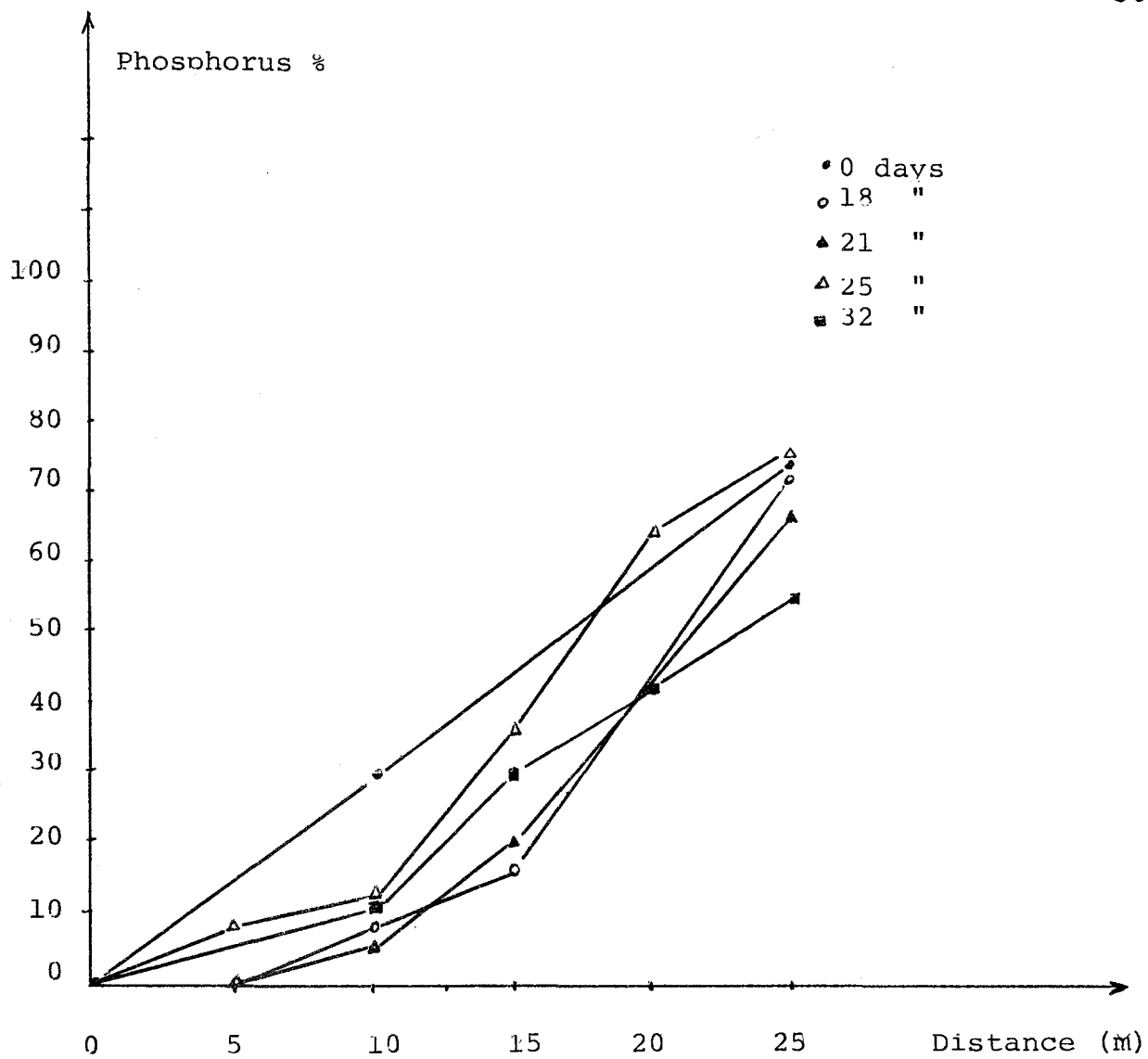
Figure 37 : Removal Efficiency of Phosphorus with Distance in the Channel Full with Sand
