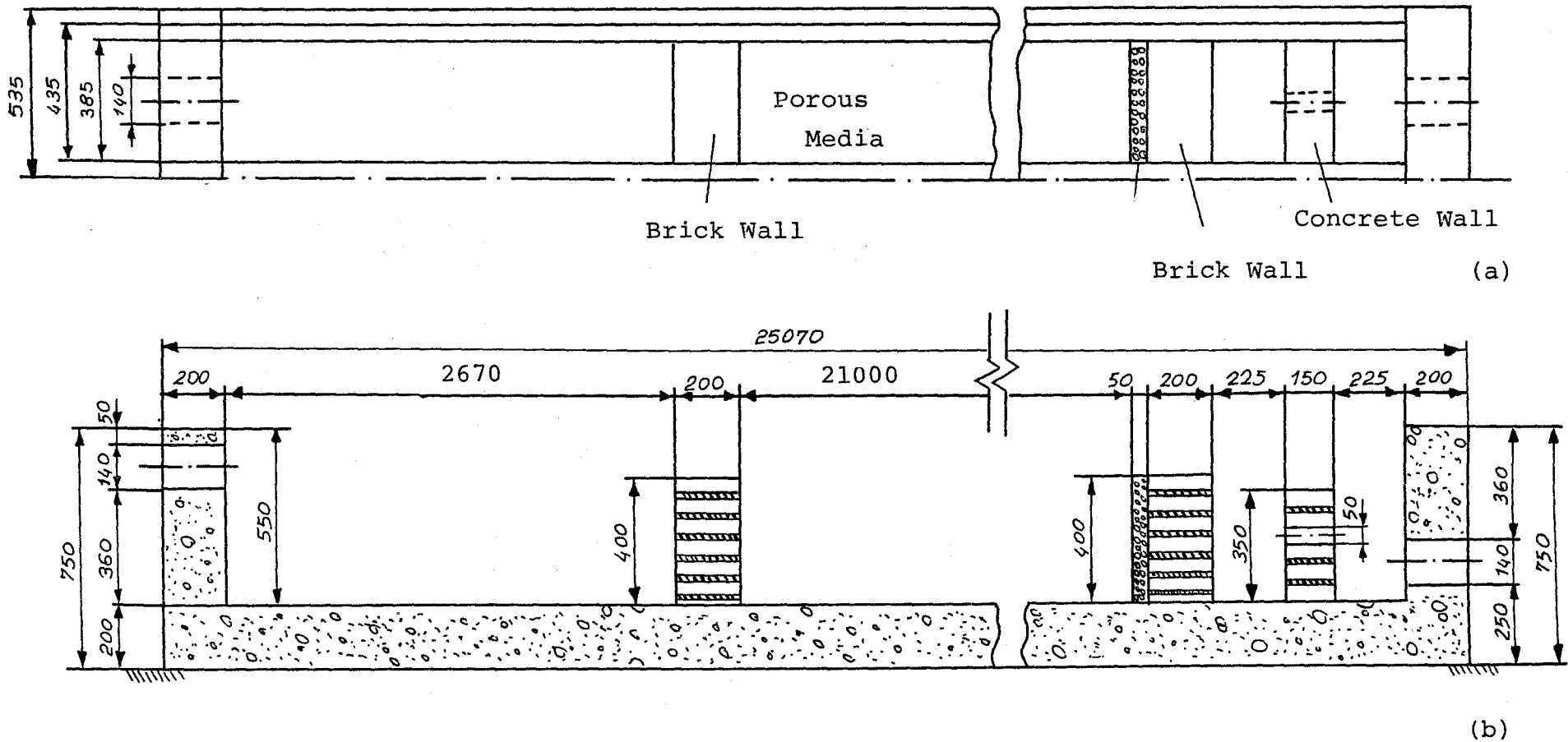
Figure 10a : Top View of the Channel b : Longitudinal Cross- Section of the Channel (A.Baysal, 1984)
