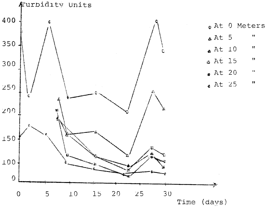
Figure 46 : Variation of Turbidity with Time in the Channel Full with Sand
