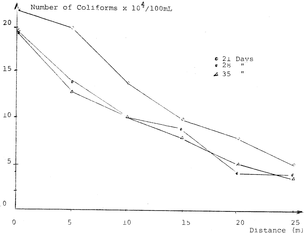
Figure 59 : The variation of Number of Coliform with Distance in the Channel Full with Gravel
