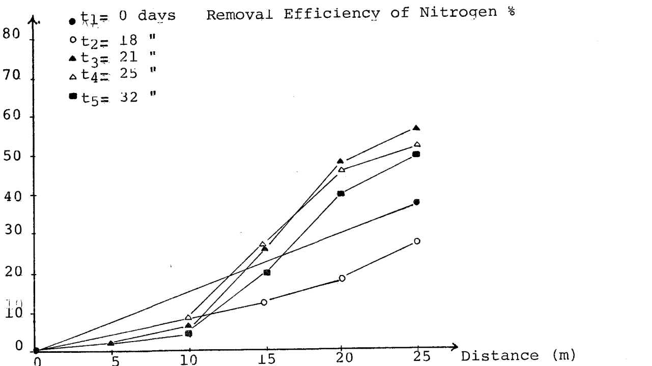
Figure 33 : Graphical Presentation Showing the Removal Efficiency of Nitrogen with Distance in the Channel Full with Gravel
