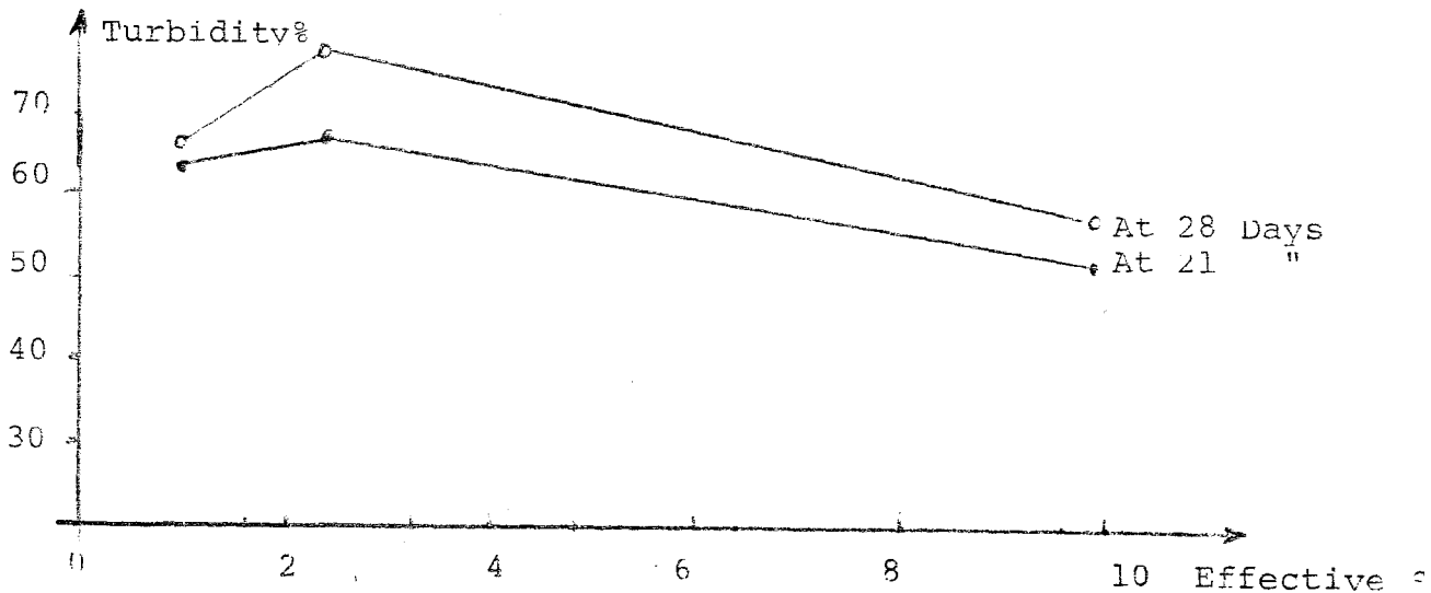
Figure 54 : Removal Efficiency of Turbidity with Effective size of Porous Media
