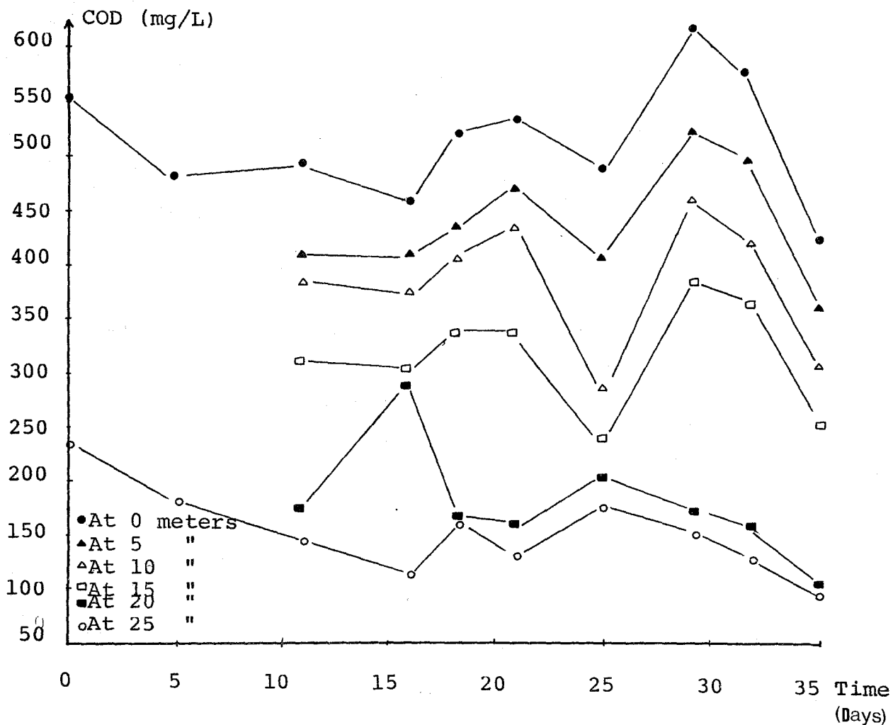
Figure 18 : Graphical Presentation Showing the Variation of COD with Time in the Channel Full with Sand
