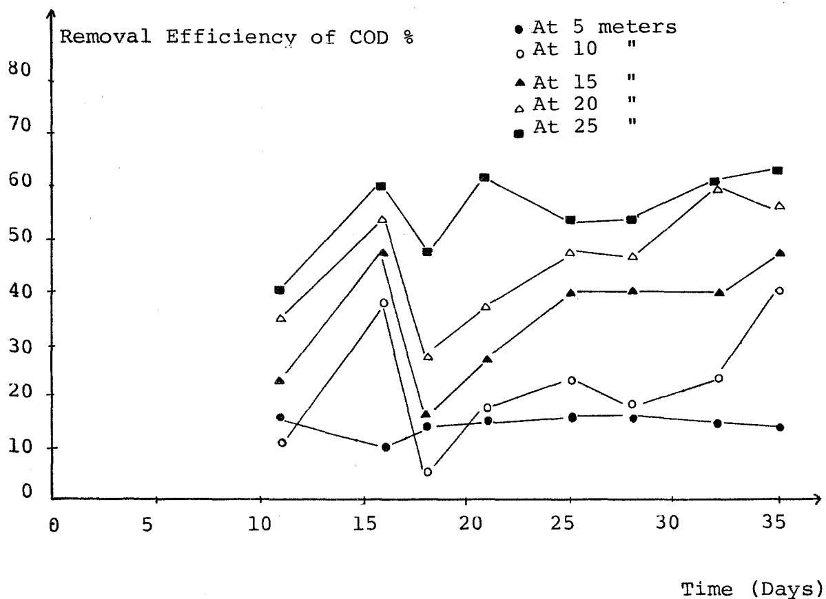
Figure 23 : Graphical Presentation Showing the Removal Efficiency of COD with Time in the Channel Full with Gravel
