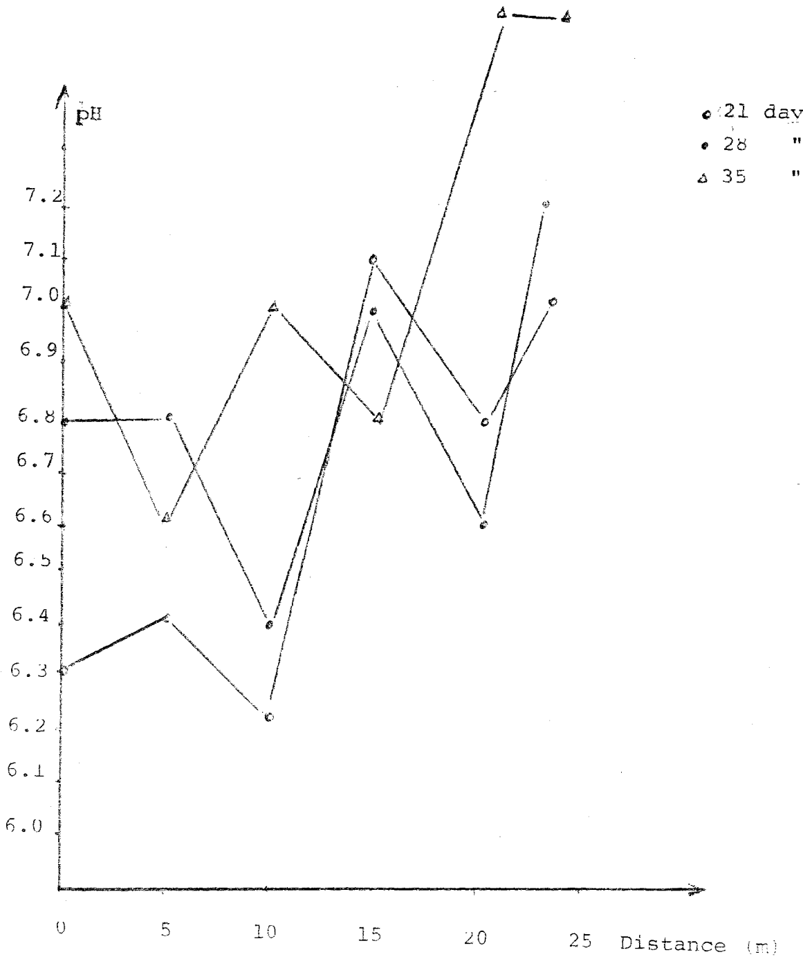
Figure 56 : Variation of pH with Distance in the Channel Full with Gravel
