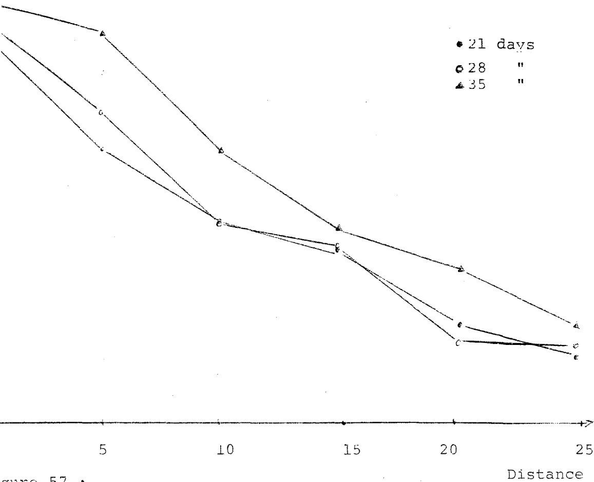
Figure 57 : Variation of Total Coliform with Distance in the Channel Full with Sand
