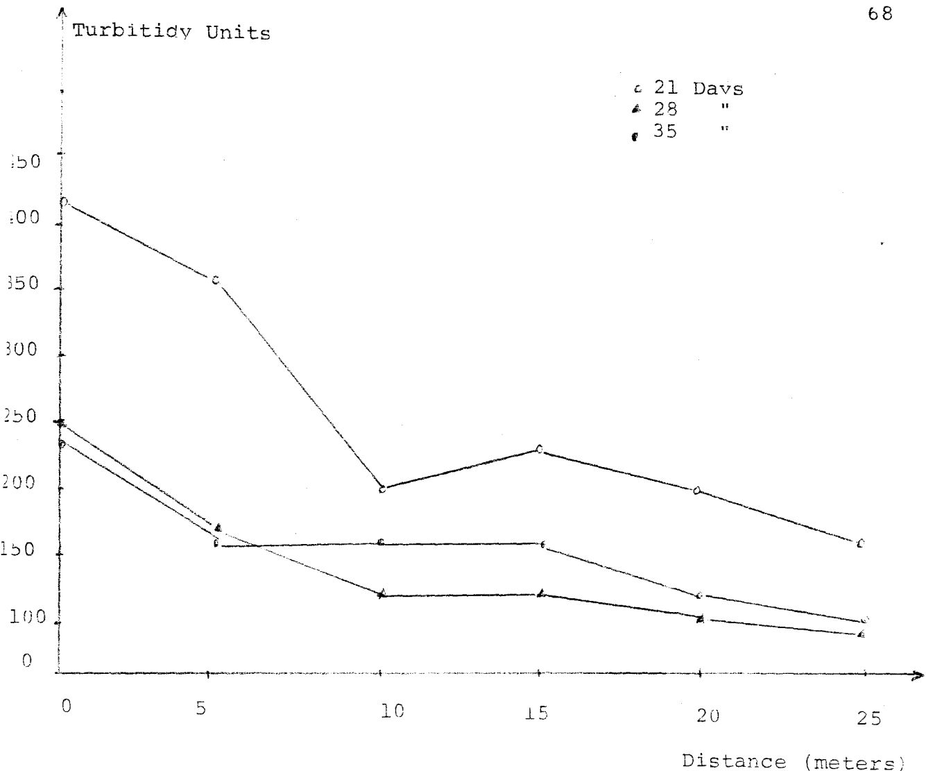
Figure 52 : Variation of Turbidity with Distance in the Channel Full with Gravel
