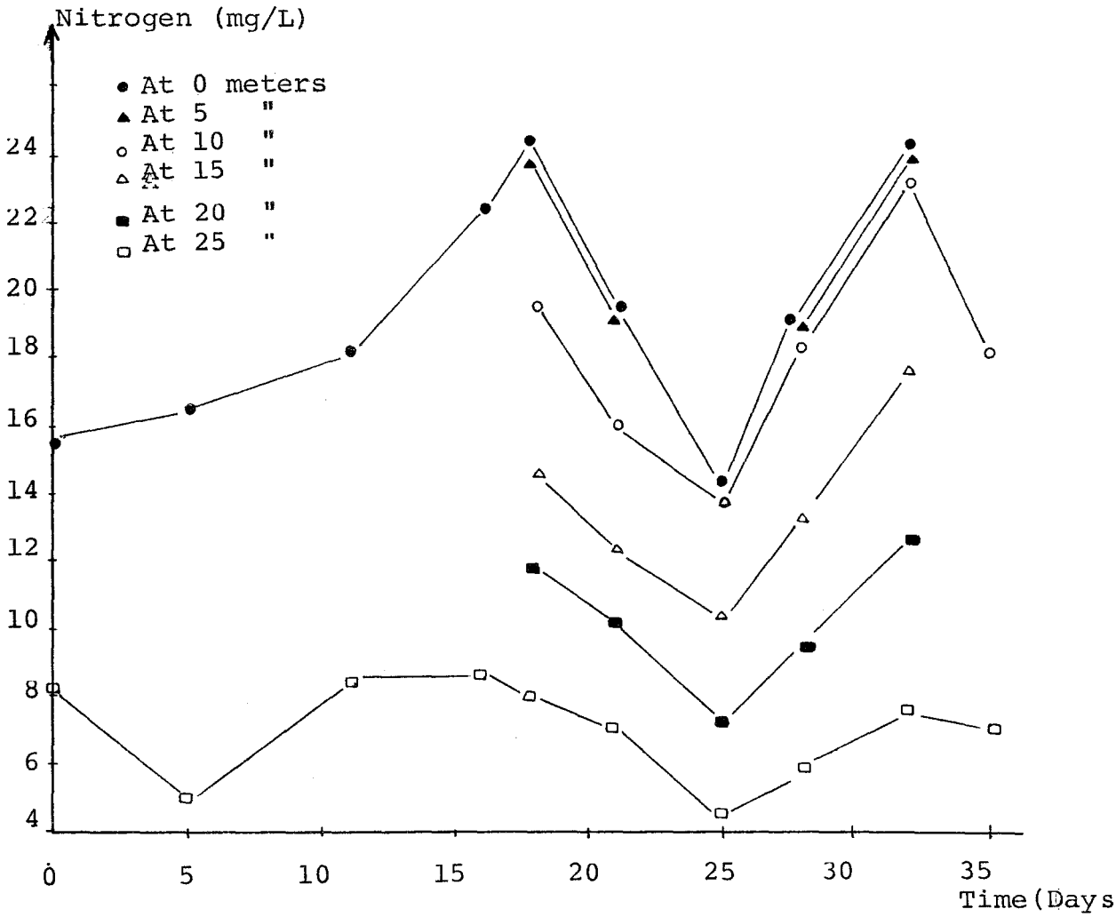
Figure 27 : Graphical Presentation Showing the Variation of Nitrogen with Time in the Channels Full with Sand
