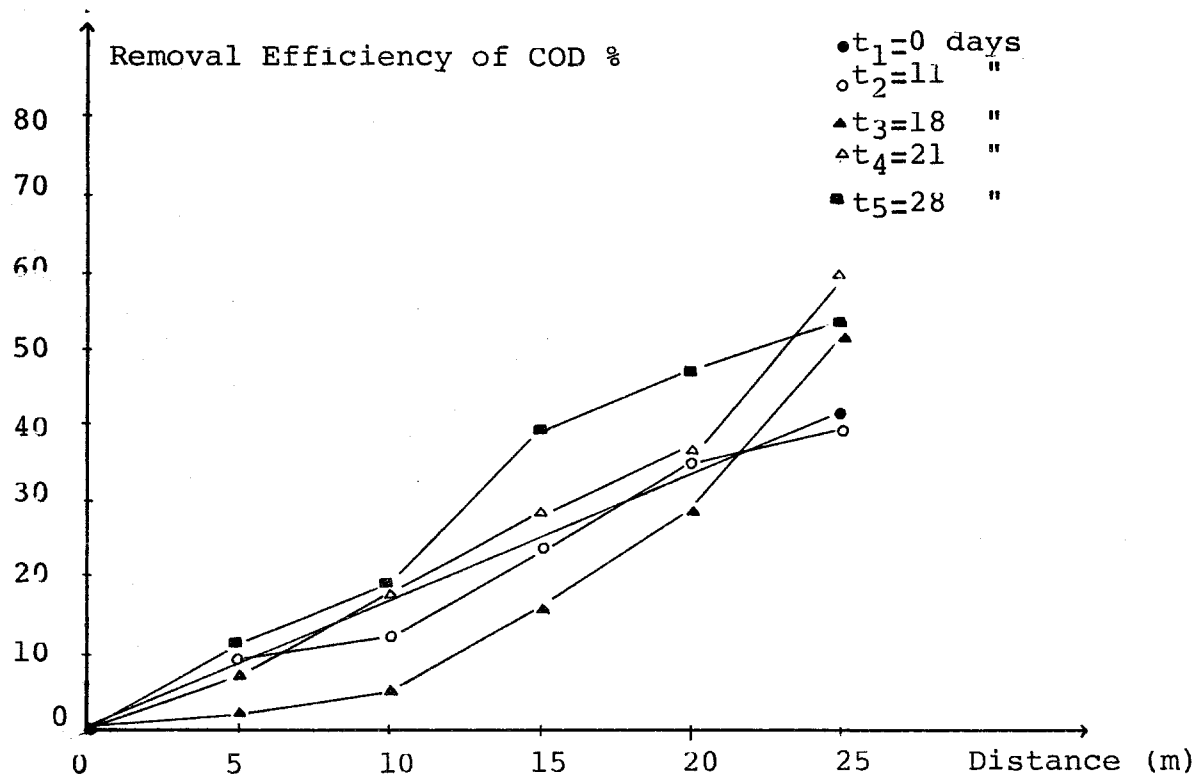
Figure 24 : Graphical Presentation Showing the Removal Efficiency of COD with Distance in the Channel Full with Gravel
