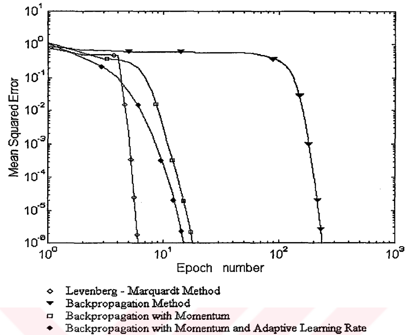
Figure 3.1 Mean squared error graph for XOR problem
