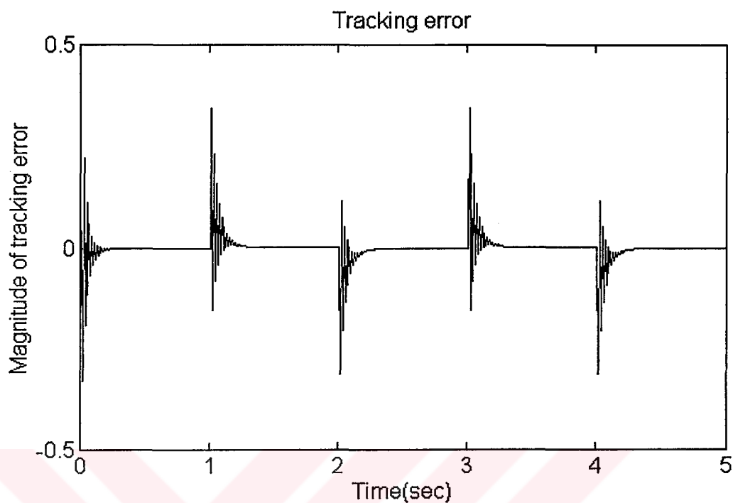
Figure 5.14(b) Tracking error when the PI controller is active. Reference input is r(t) = \text{sgn}[\sin(\pi t)]
