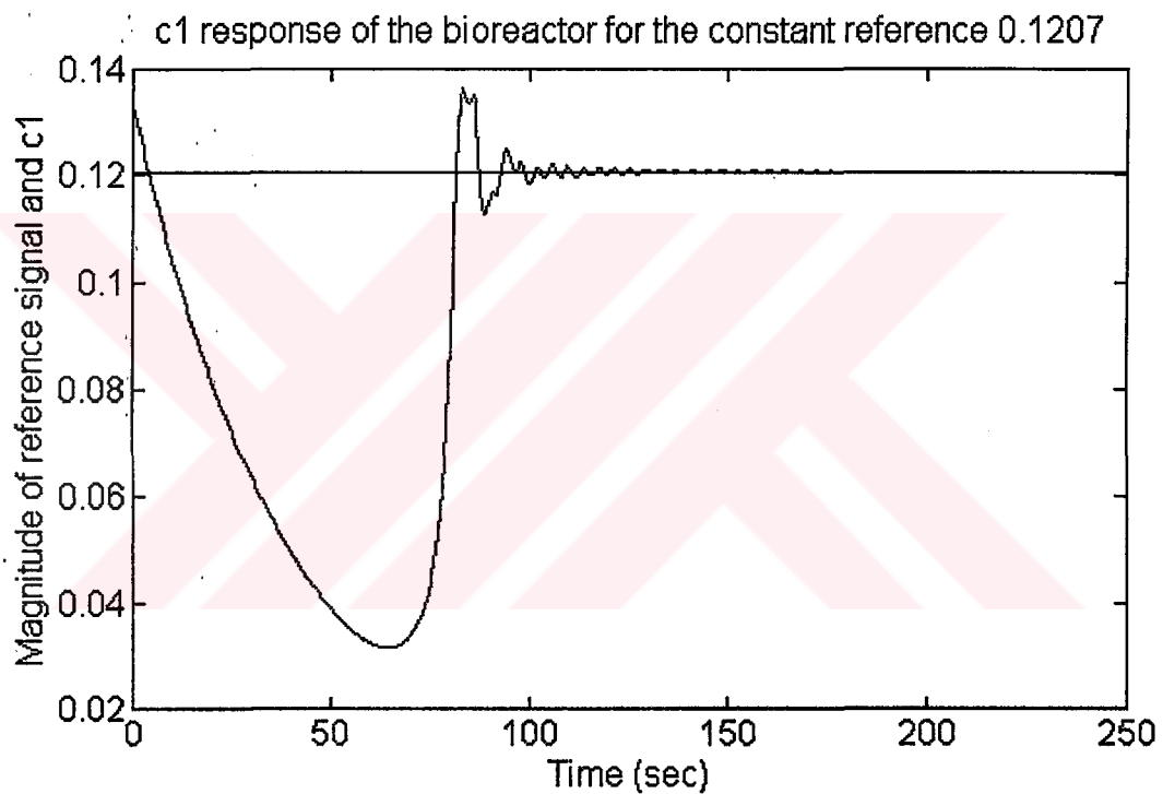
Figure 9.11(a) c_1(t) Output of the bioreactor plant defined by Equations (9.27) and (9.28) in response to the constant input 0.1207
