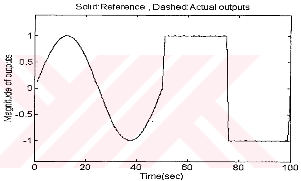
Figure 6.3(a) Output graph for the first plant
