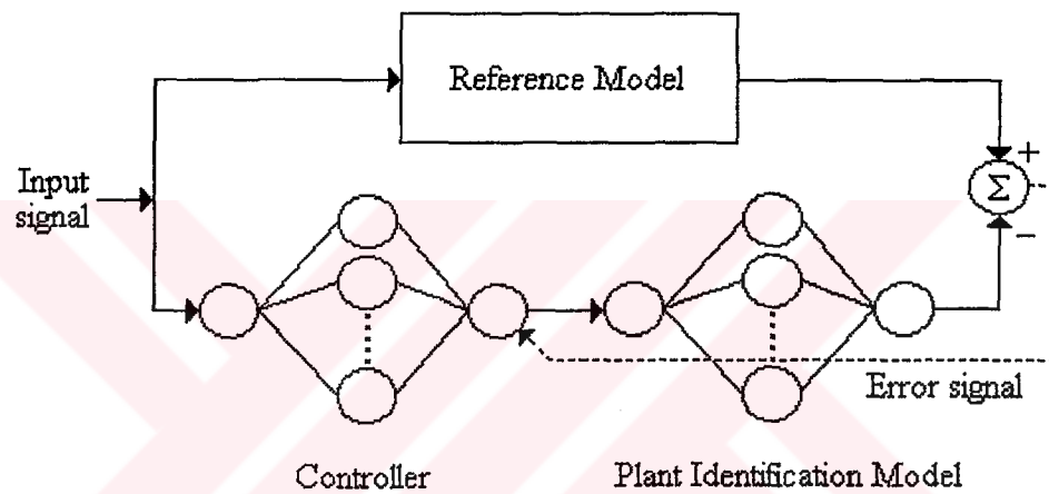
Figure 5.4 Controller training architecture for the first simulation
