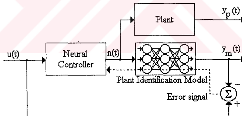
Figure 5.3 Controller training architecture by the use of plant identification model
