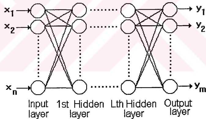
Figure 2.4 Multilayer feedforward neural network
