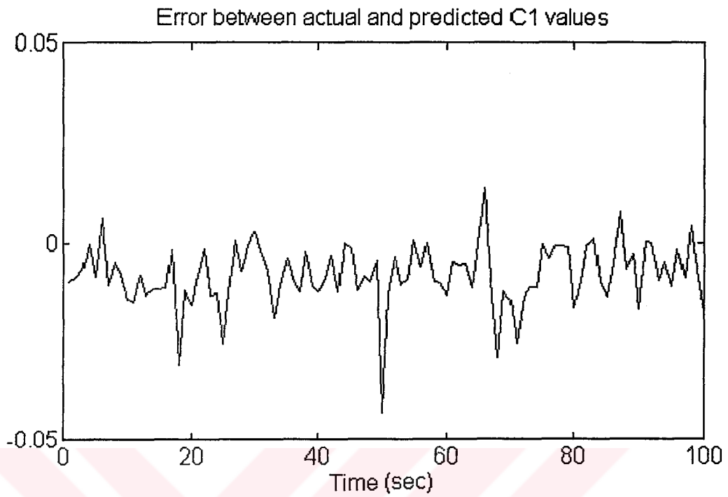
Figure 4.7(b) Error between actual and predicted c_1 values
