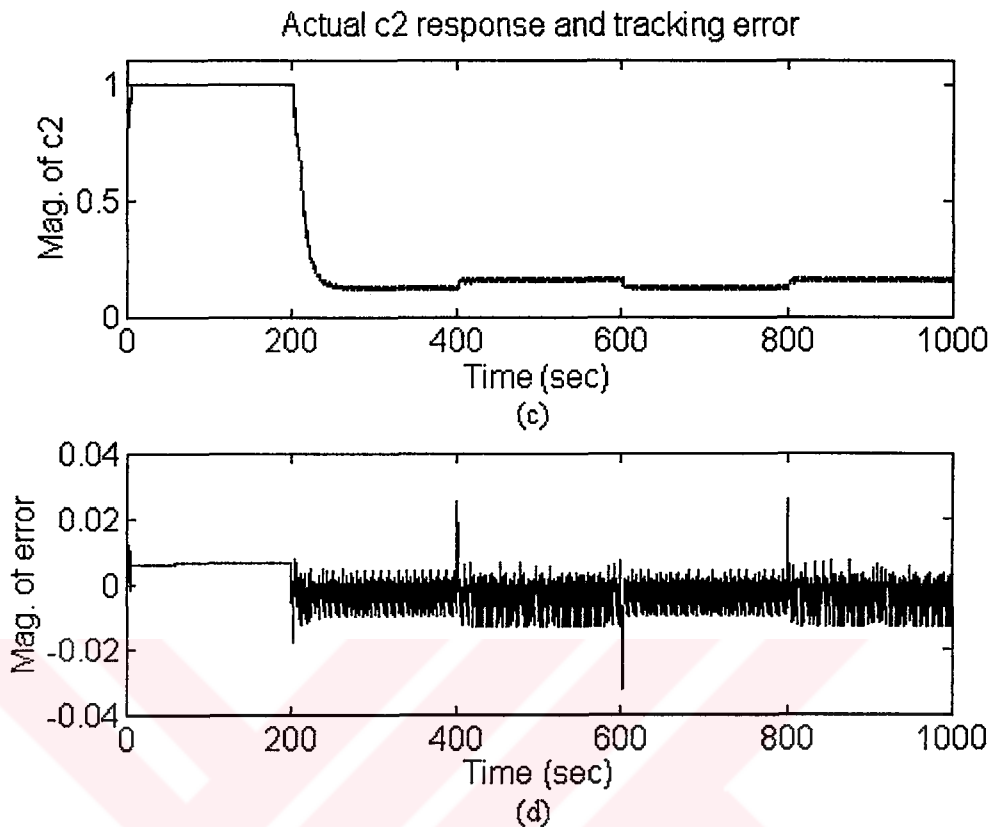
Figure 5.18 (c) Actual c_2 trajectory (d) The difference between command signal and actual c_1 value
