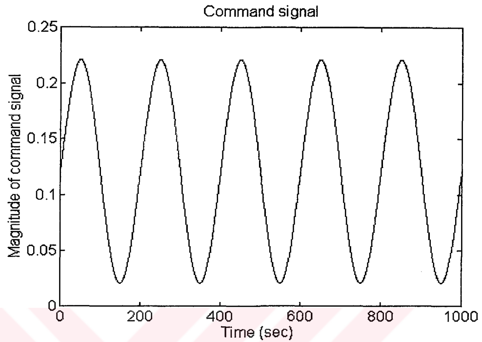
Figure 7.7(b) Command signal graph, r(t) = 0.1207 + 0.1\sin(2\pi t/200)
