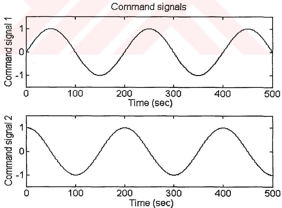
Figure 7.5(b) Applied reference inputs to the system
