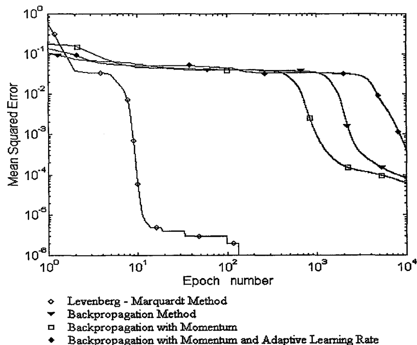
Figure 3.2 Mean squared error graph for function approximation problem
