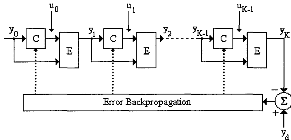
Figure 8.1 Controller training architecture for the self-learning control scheme
