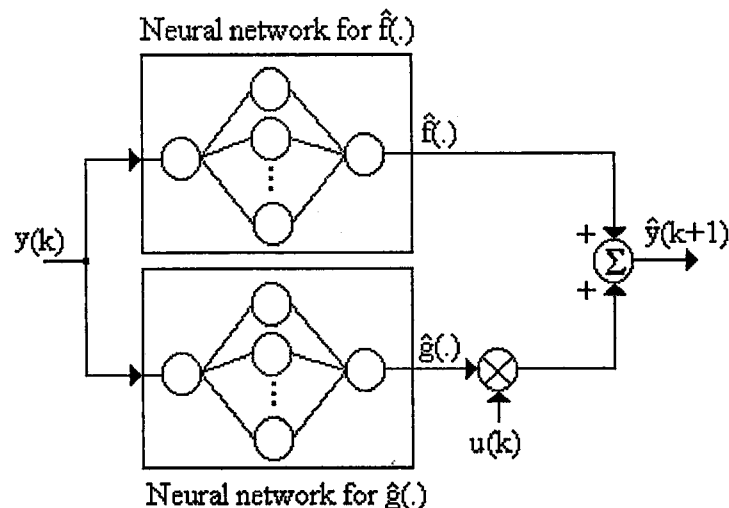
Figure 6.2 Structure of the neural network
