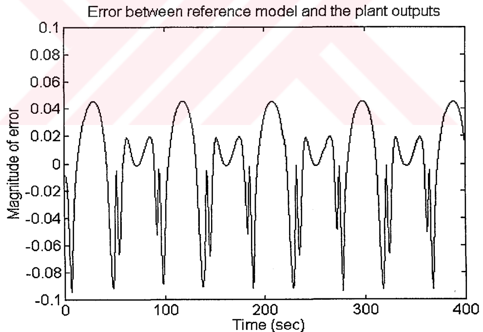
Figure 7.3(c) Error graph for the first reference input defined by Equation (7.3) and illustrated in Fig. 7.3(b)
