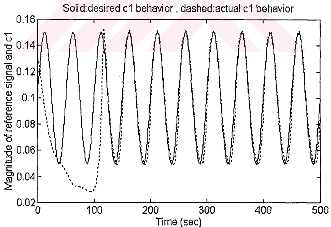
Figure 9.9(a) c_1(t) Output of the bioreactor plant defined by Equations (9.27) and (9.28) in response to the input defined by Equation (9.29)
