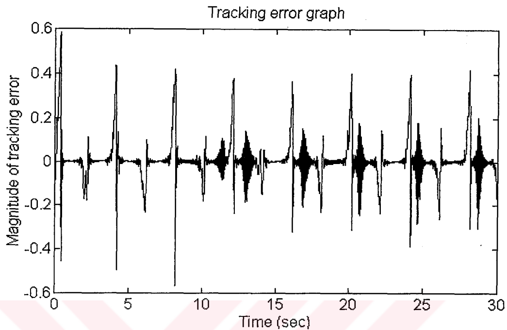
Figure 9.5(b) Output error for the plant defined by Equation (9.19) in response to the input defined by Equation (9.20), 10% Gaussian random noise is added to the measured state y(k)
