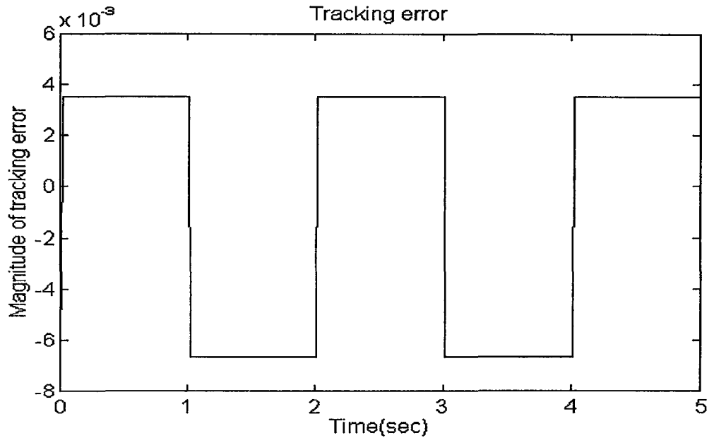
Figure 5.6(b) Tracking error for the first plant, the reference input is r(t) = 0.5 * \text{sgn}[\sin(\pi t)]
