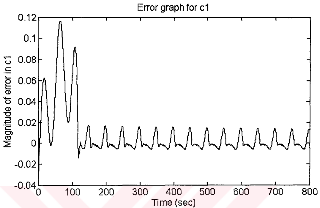
Figure 9.9(b) Tracking error in c_1(t) for the plant defined by Equations (9.27) and (9.28) in response to the input defined by Equation (9.29)
