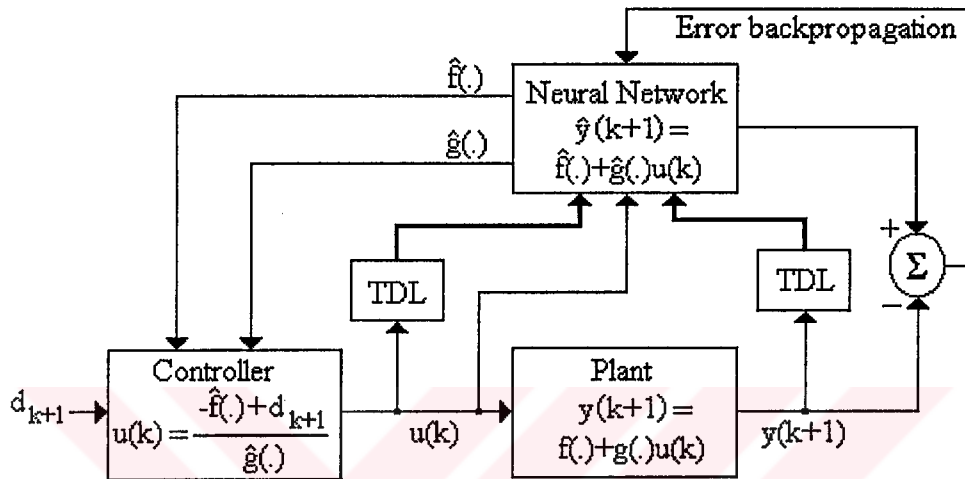
Figure 6.1 Self-tuning control scheme with neural networks
