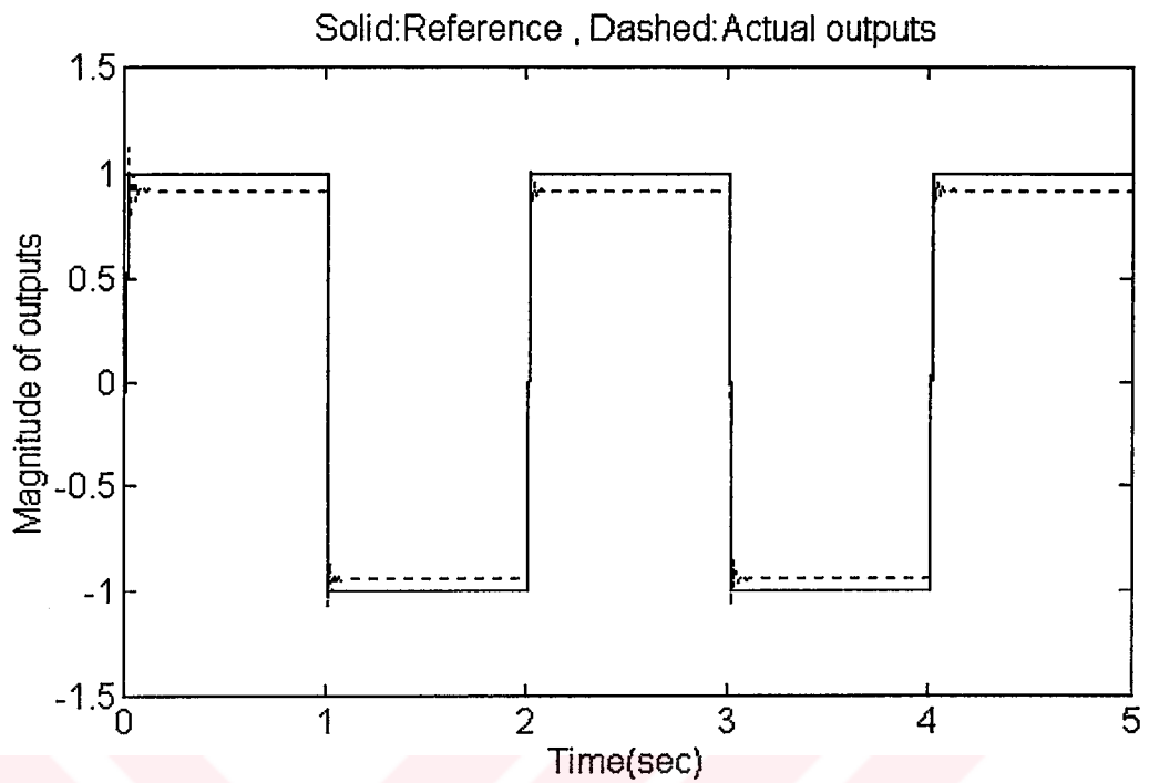
Figure 5.8(a) Reference and actual trajectories for the second plant, reference input is r(t) = \text{sgn}[\sin(\pi t)]
