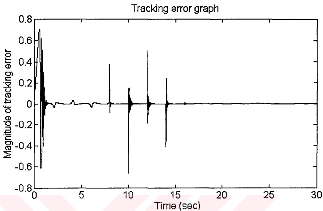
Figure 9.8(b) Output error for the plant defined by Equation (9.25) in response to the input defined by Equation (9.26)
