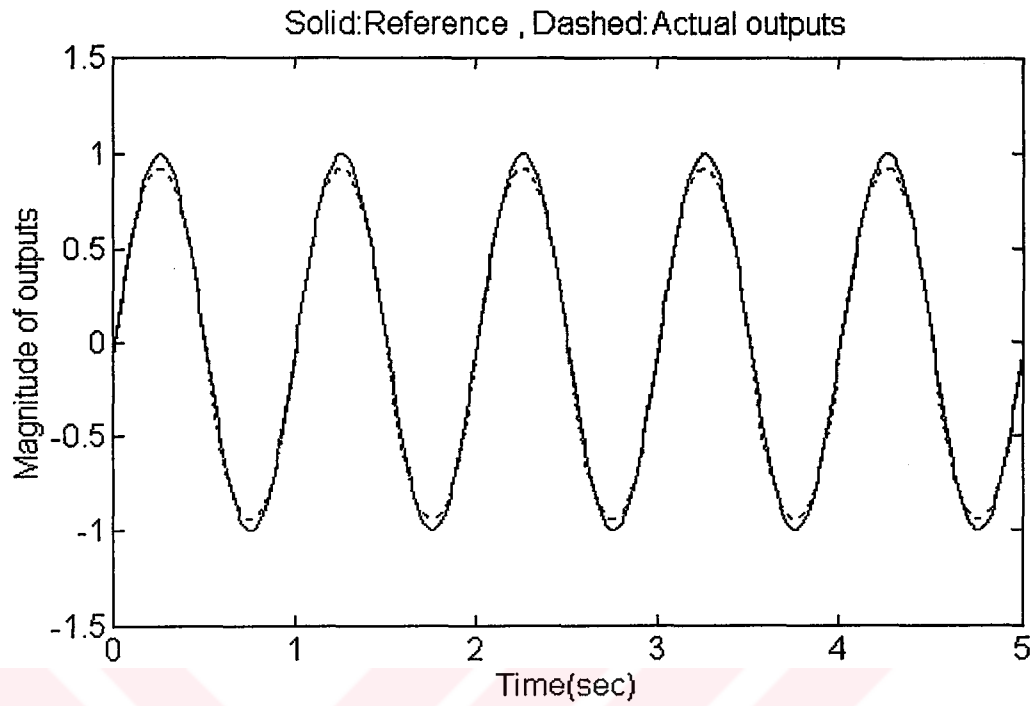
Figure 5.9(a) Reference and actual trajectories for the second plant, reference input is r(t) = \sin(2\pi t)
