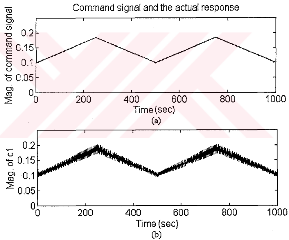
Figure 5.17 (a) Command signal (b) Actual c_1 trajectory
