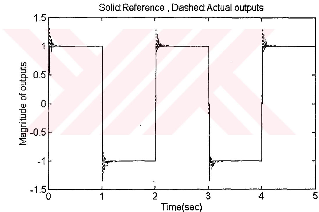
Figure 5.14(a) Reference and actual trajectories when a PI controller was used with the neural controller. Reference input is r(t) = \text{sgn}[\sin(\pi t)]
