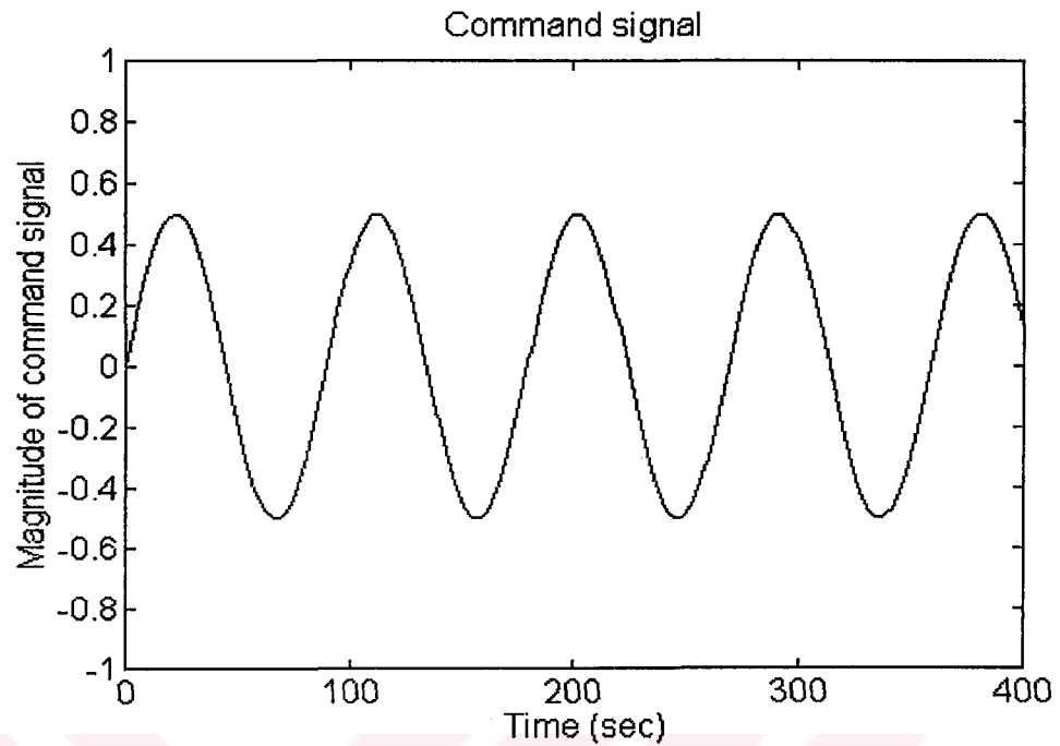
Figure 7.3(b) Applied reference input to the system
