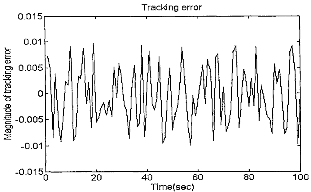
Figure 6.5(b) Tracking error graph for the third plant
