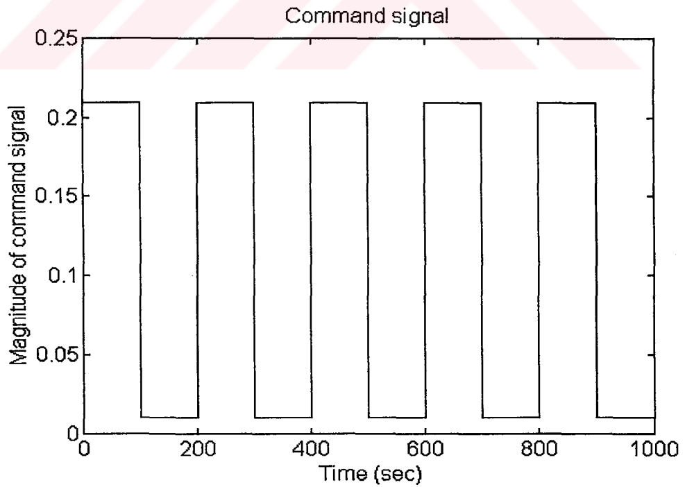
Figure 7.8(b) Command signal graph, r(t) = 0.11 + 0.1\text{sgn}(\sin(2\pi t/200))
