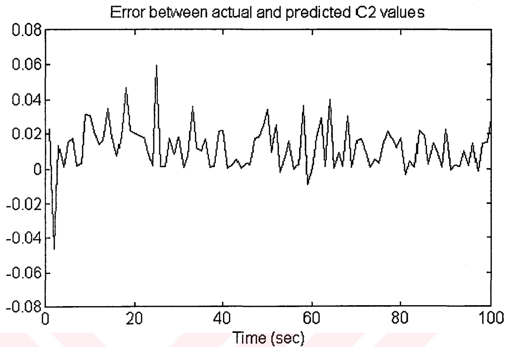
Figure 4.7(d) Error between actual and predicted c_2 values
