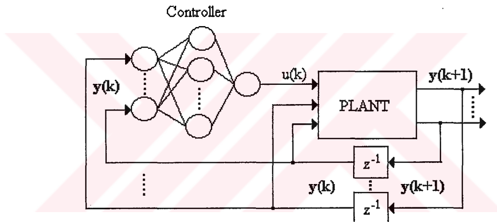
Figure 8.2 Control system structure with neural controller
