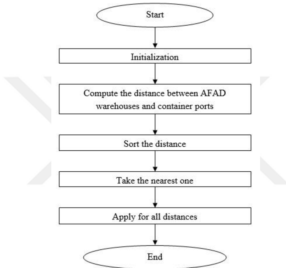
Figure 10 Flowchart of the heuristic approach
