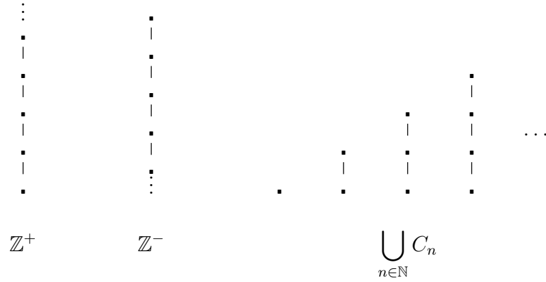
Figure 3.1. The three most basic unbounded posets.
