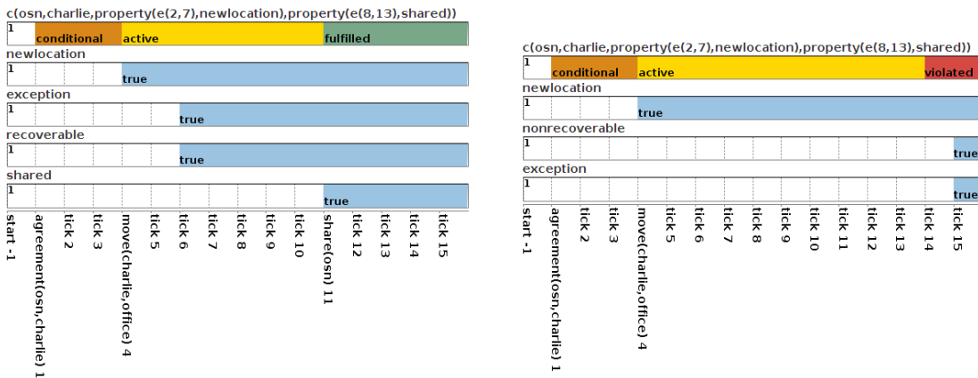
(a) Recoverable: j\text{-REC} output
