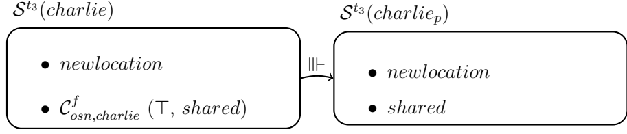
Figure 2.5. State satisfiability.
