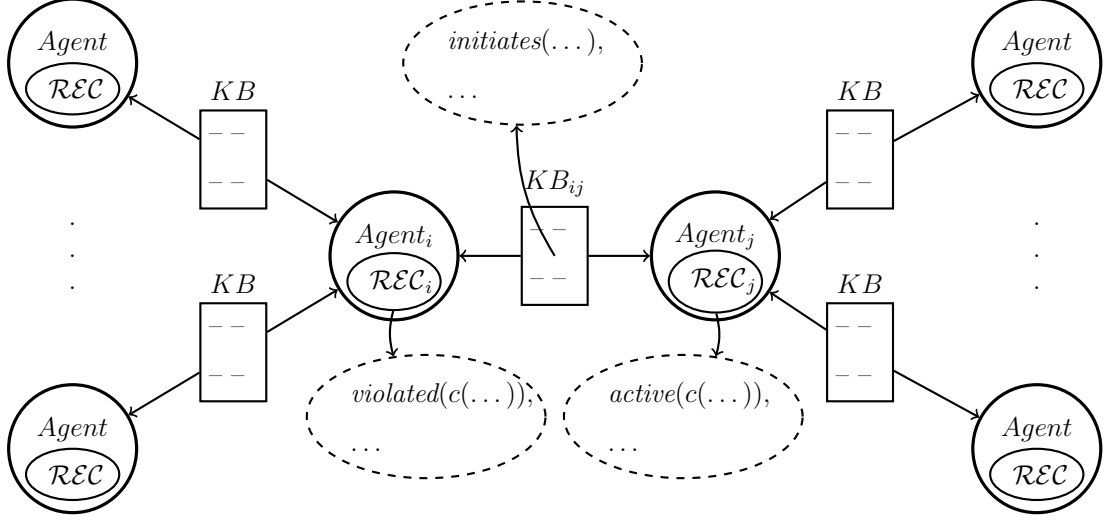
Figure 4.11. Diagnosis architecture.
