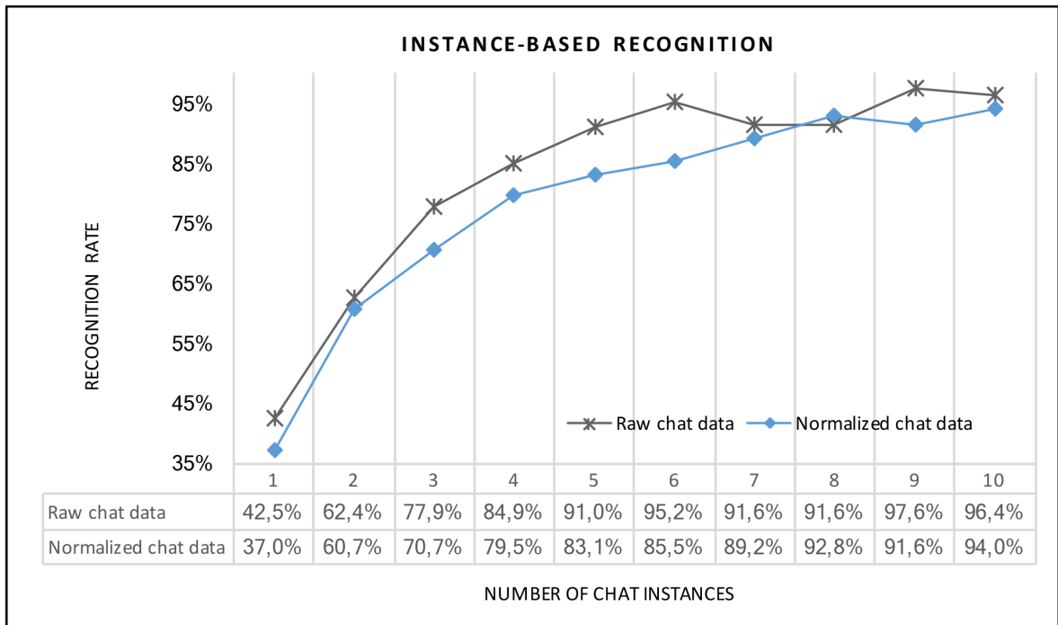
Figure 6.23. Comparison of recognition rates for COPA-NORM before and after the normalisation on the instance-based approach.
