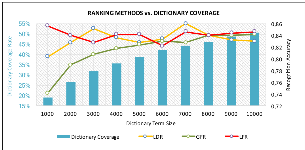
Figure 6.10. Average cross-validation accuracies with different rankings & dictionary size for C10 dataset (6-gram char. features, TF-IDF weighting, ELM parameters: \lambda = 230 , \alpha = 0, 7 , \omega = 0, 9 ).
