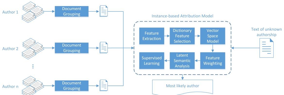
Figure 3.1. Pipeline of the proposed instance-based approach.
