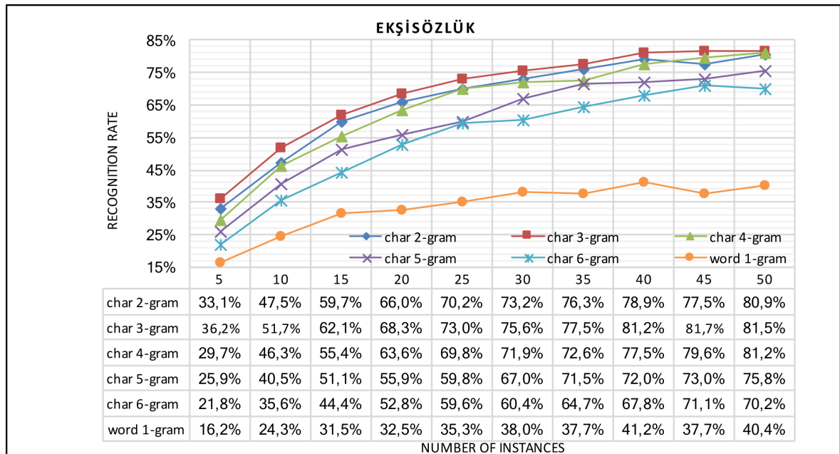
Figure 6.1. Comparison of lexical features for Ekşisözlük. (Dictionary size: 5,000 with local frequent ranking, no weighting, ELM params: \lambda = 250 , \alpha = 0,5 , \omega = 0,5 .)
