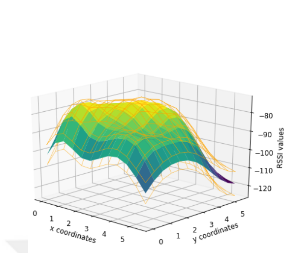
Figure 1.1. Deterministic radio map
