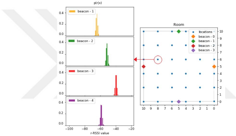
Figure 3.2. Room configuration based on synthetic data
