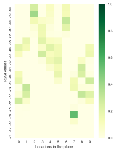
Figure 1.2. Probabilistic radio map
