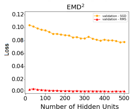
Figure 3.6. EMD^2 Loss Change
