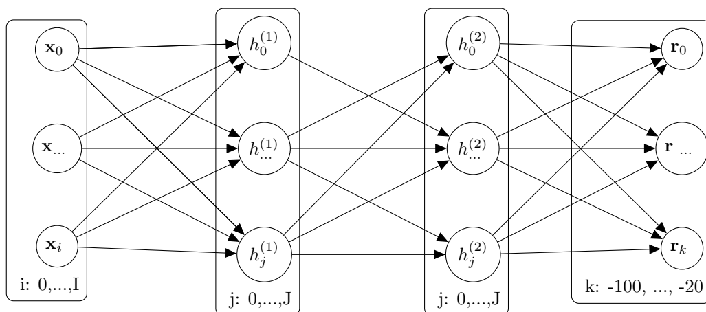
Figure 2.3. Computation Graph of a Deep Neural Network
