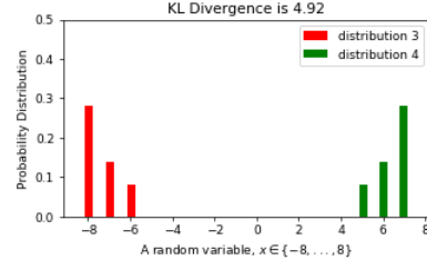
Figure 2.5. KL Divergence between Distribution 3 and 4
