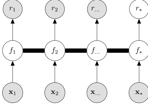
Figure 2.6. Graphical Model of Gaussian Process Regression [1]
