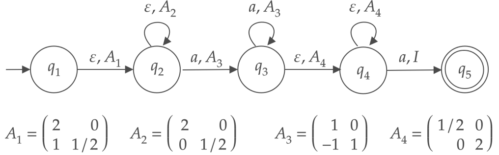
Figure 3.2. State transition diagram of \mathcal{E} recognizing \text{UPOW}_{\text{odd}}
