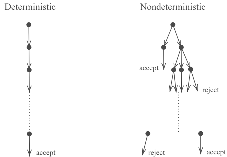
Figure 2.1. Deterministic and nondeterministic computation
