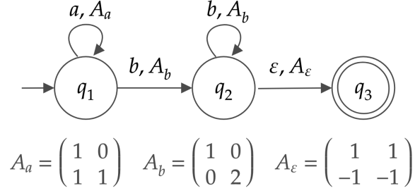
Figure 4.6. State transition diagram of \mathcal{V} recognizing \text{POW}_r
