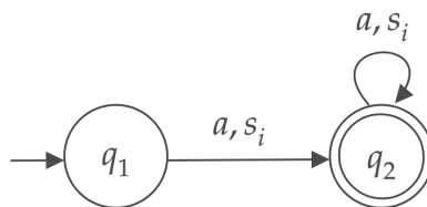
Figure 3.6. State transition diagram of \mathcal{E}_2
