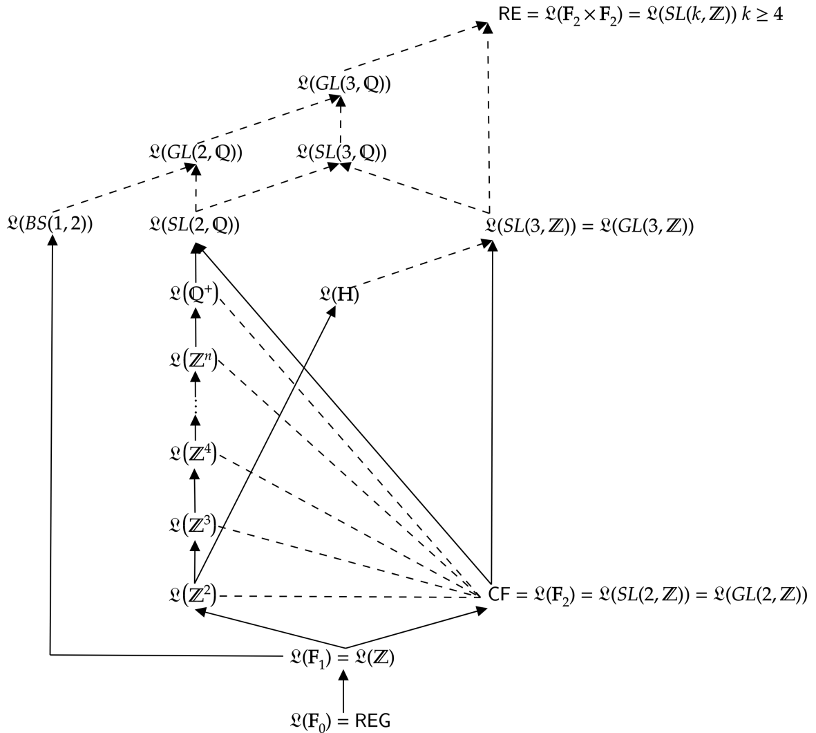
Figure 3.3. Language classes associated with groups
