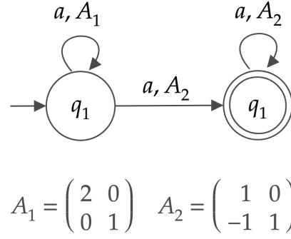
Figure 4.3. State transition diagram of \mathcal{V} recognizing \text{UPOW}'
