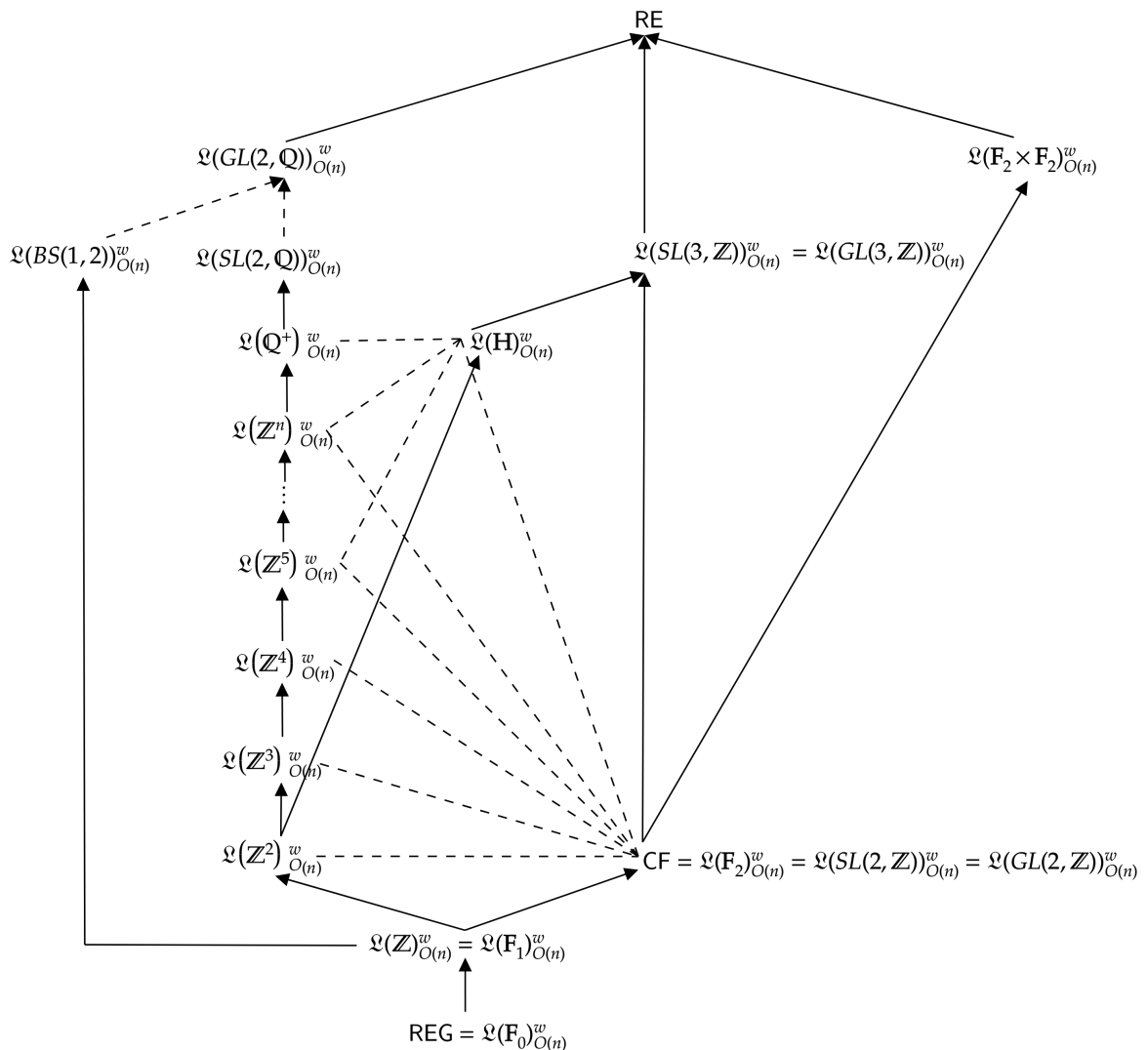
Figure 3.4. Language classes recognized by weakly linear-time bounded group automata
