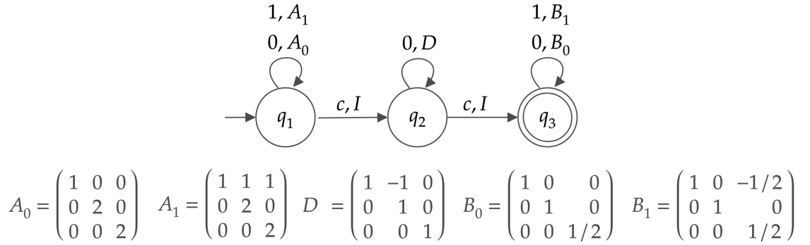
Figure 4.5. State transition diagram of \mathcal{V} recognizing BIN
