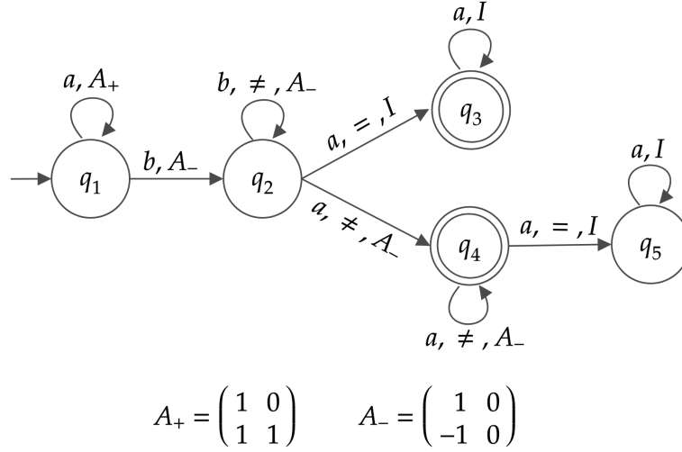
Figure 4.8. State transition diagram of \mathcal{V} recognizing SUM
