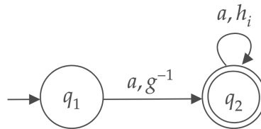
Figure 3.5. State transition diagram of \mathcal{E}_1
