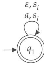
Figure 3.8. State transition diagram of \mathcal{E}_4
