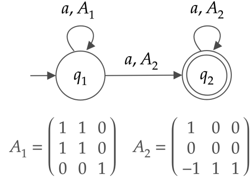
Figure 4.4. State transition diagram of \mathcal{V} recognizing \text{UPOW}'
