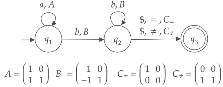
Figure 4.1. State diagram of \mathcal{V}' recognizing NEQ
