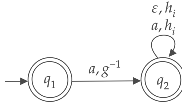
Figure 3.7. State transition diagram of \mathcal{E}_3
