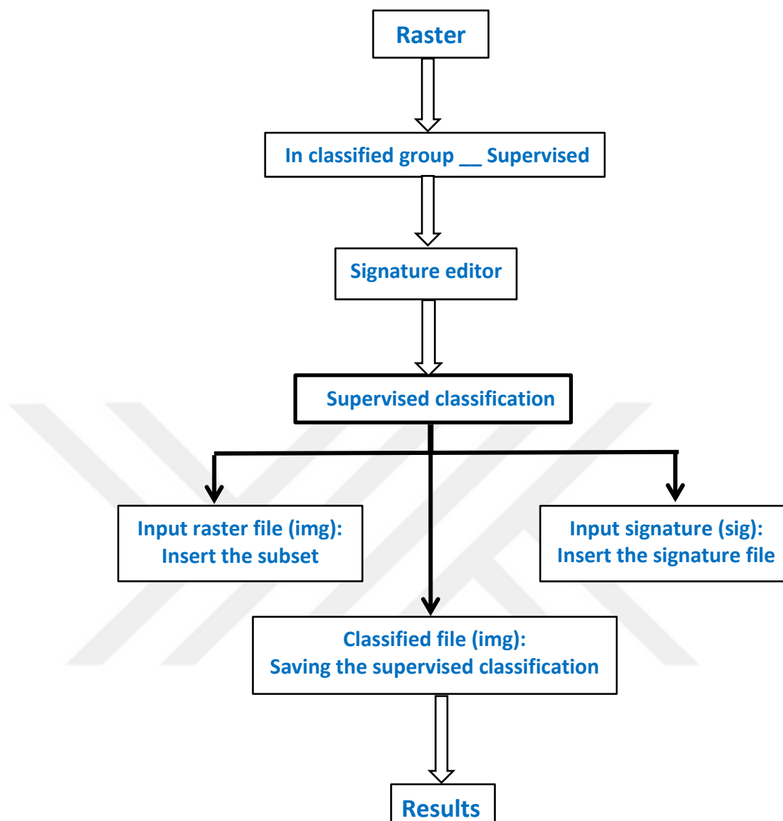
Figure 4.5. Workflow defining the supervised classification method
