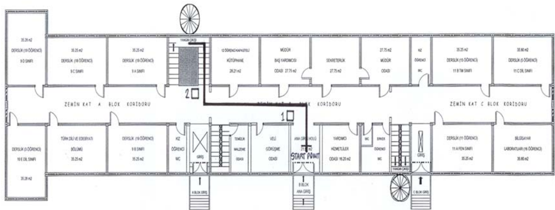
Figure 4.2. Ground Floor Plan of the high school building with selected route
