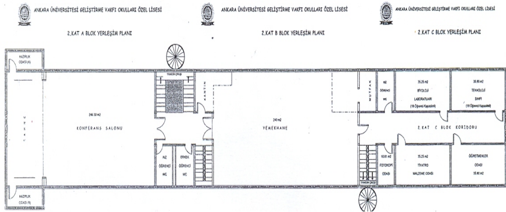
Figure A2.4. 2 nd Floor Plan of high school building.
