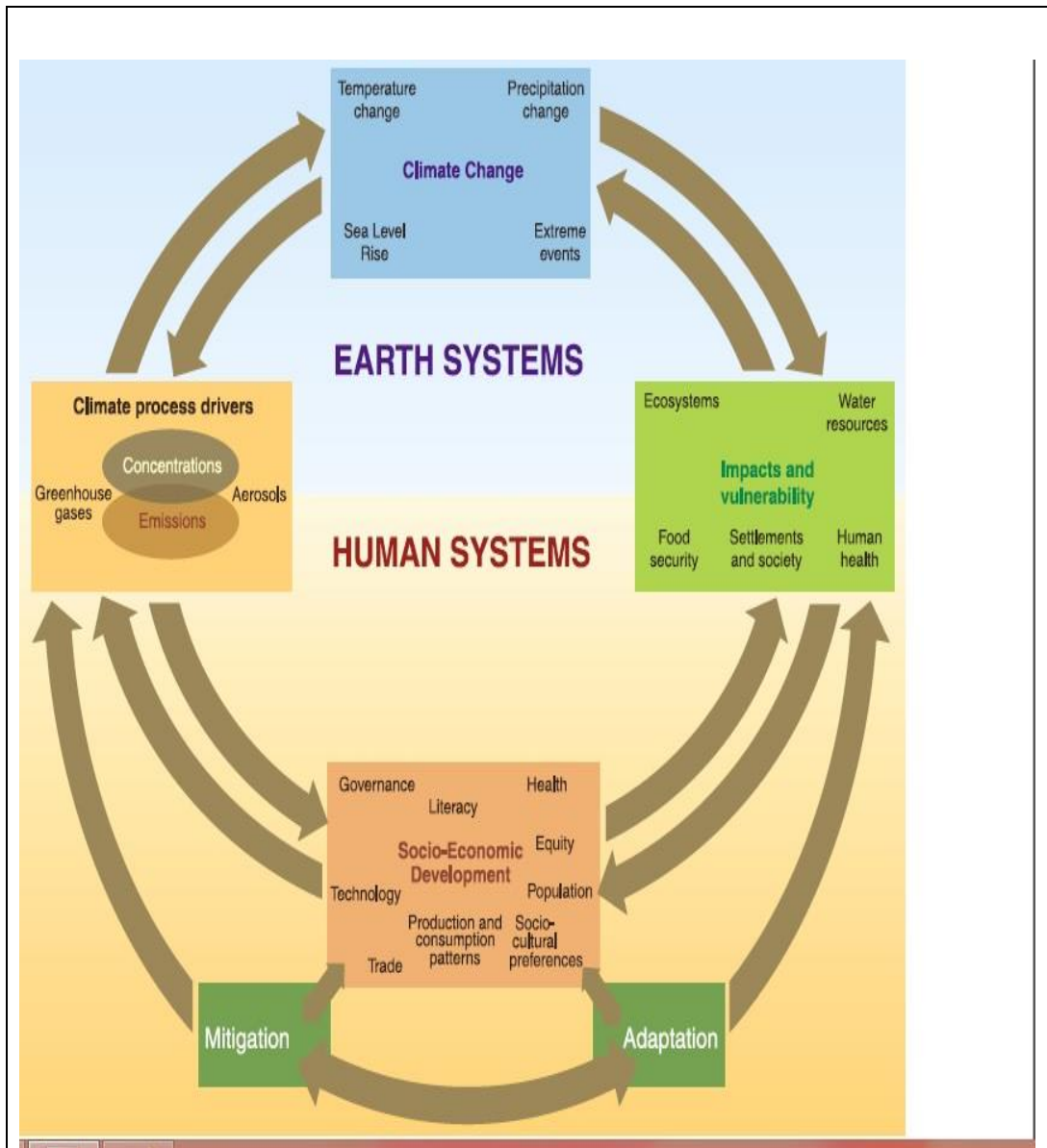
Figure 2.1 Schematic framework representing anthropogenic drivers, impacts of and responses to climate change and their linkages. Taken from “IPCC 4 th Assessment Report: Climate Change 2007: Synthesis Report”, p. 26.
