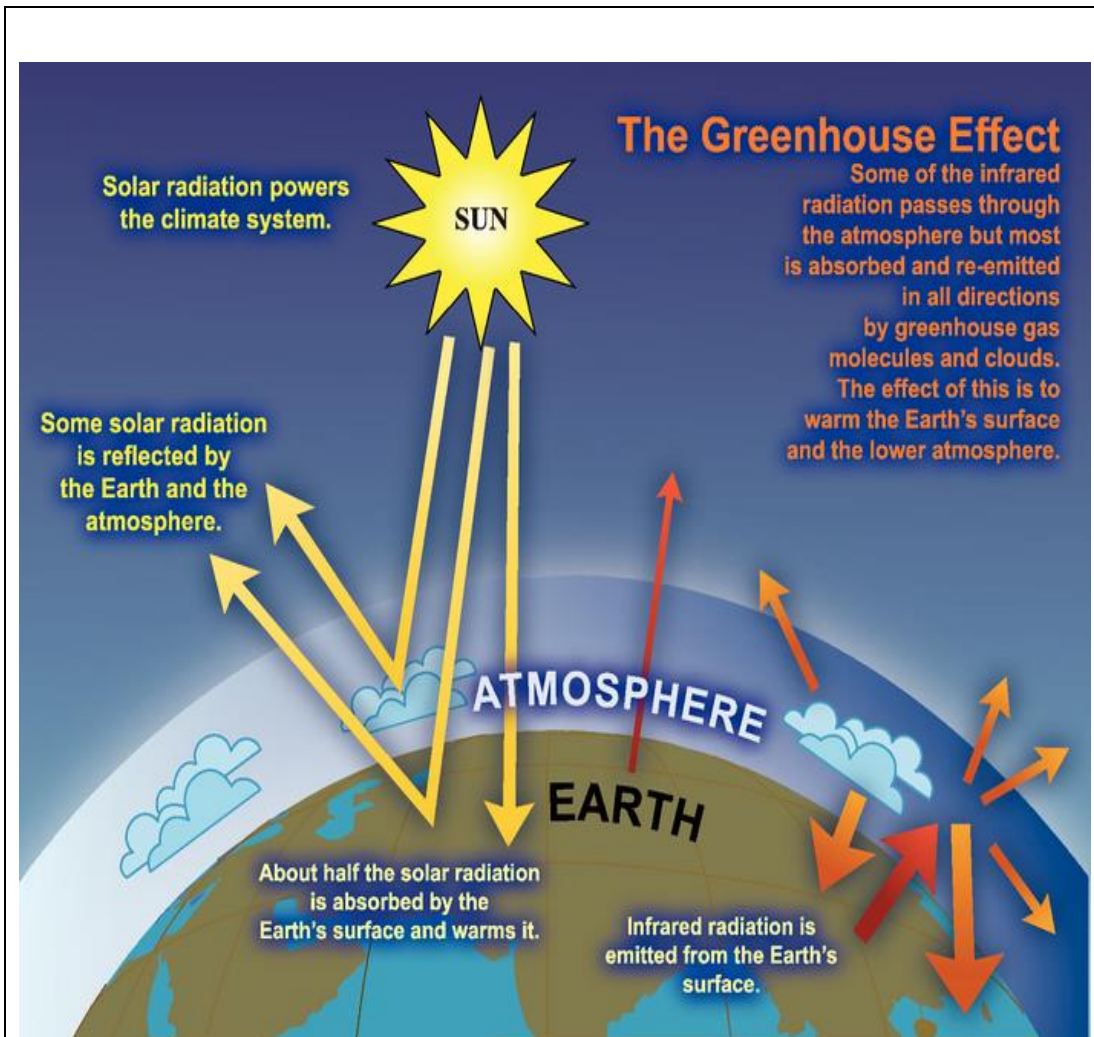
Figure 2.2 An idealized model of the natural greenhouse effect. From “IPCC Fourth Assessment Report: Climate Change 2007 Working Group I: The Physical Science Basis”, in Chapter 1, p. 115.
