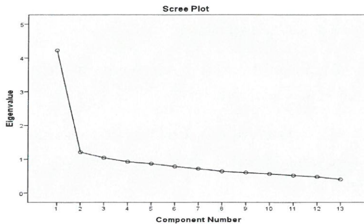
Grafik 6: Scree plot
