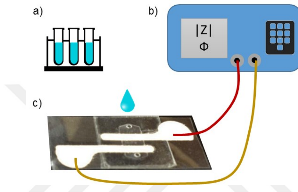
Figure 5.14 Electrical impedance measurement setup for FFChip. a) Solutions, b) LCR meter, c) FFChip.
