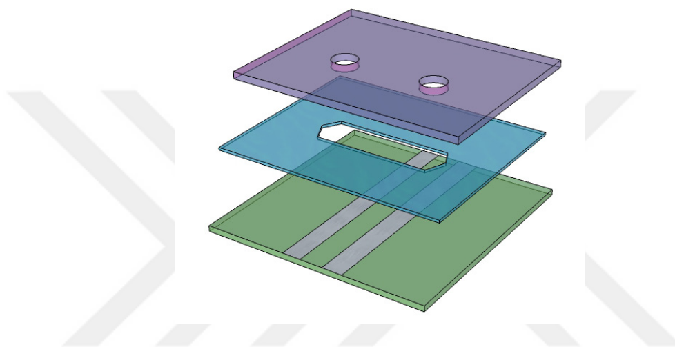
Figure 5.1 The three layers of flexible polymer based microfluidic chip (FFchip). From to bottom to top: the electrode layer, channel layer and inlet layer.
