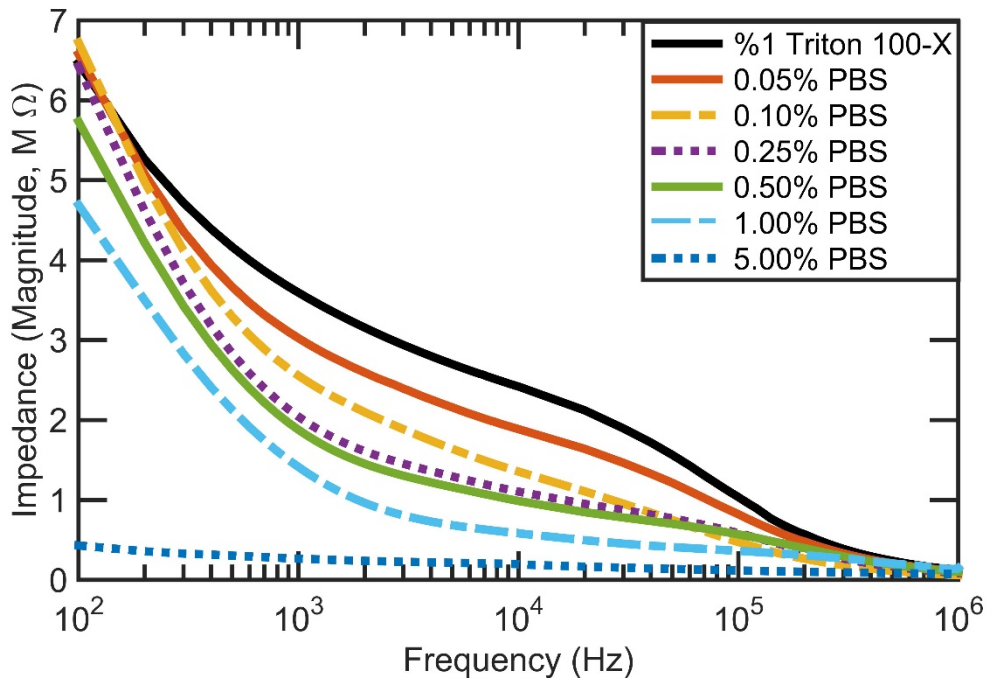
Figure 5.24 Impedance magnitude spectra of control and solutions with different PBS concentration for a frequency range between 100 Hz and 1 MHz.
