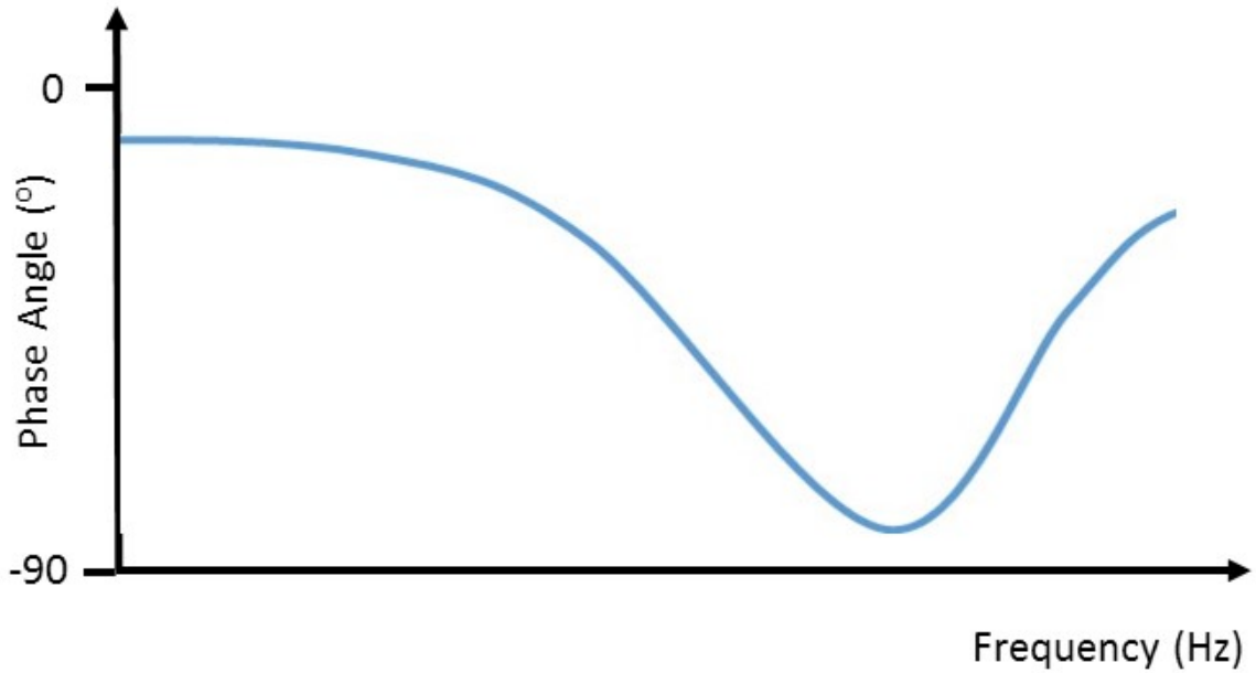
Figure 3.7 Bode plot of impedance phase against frequency for Randles electrical equivalent circuit model.
