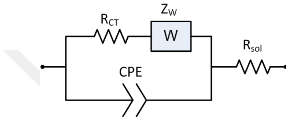
Figure 3.9 Randles electrical equivalent circuit model for each interface component in an electrochemical cell with CPE constant phase element instead of C_{DL} double layer capacitance. R_{CT} is the charge transfer resistance, Z_W is the Warburg impedance and R_{sol} is the bulk resistance.
