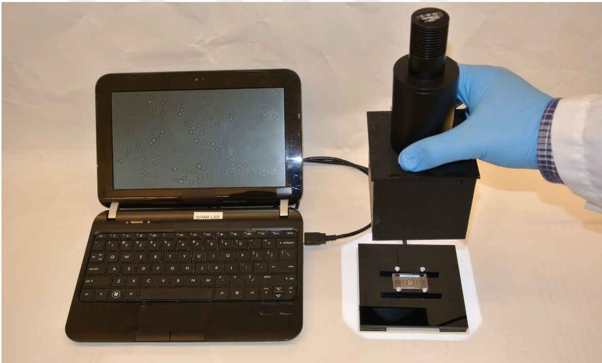
Figure 6.23 lensless wide-field microscopy system.
