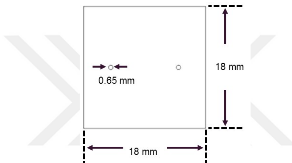
Figure 5.5 The CAD design of inlet layer.
