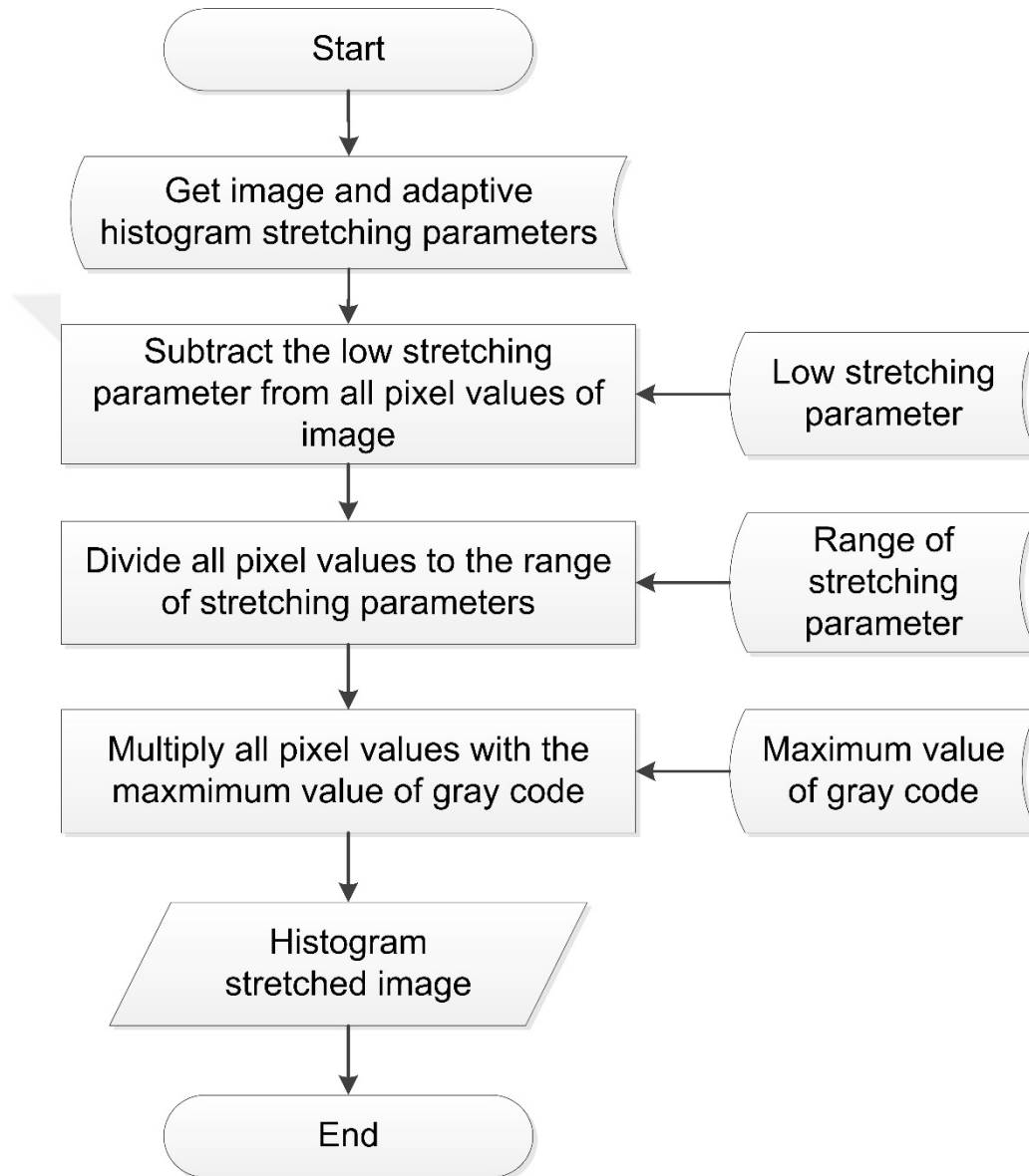
Figure 6.34 Histogram (contrast) stretching algorithm.
