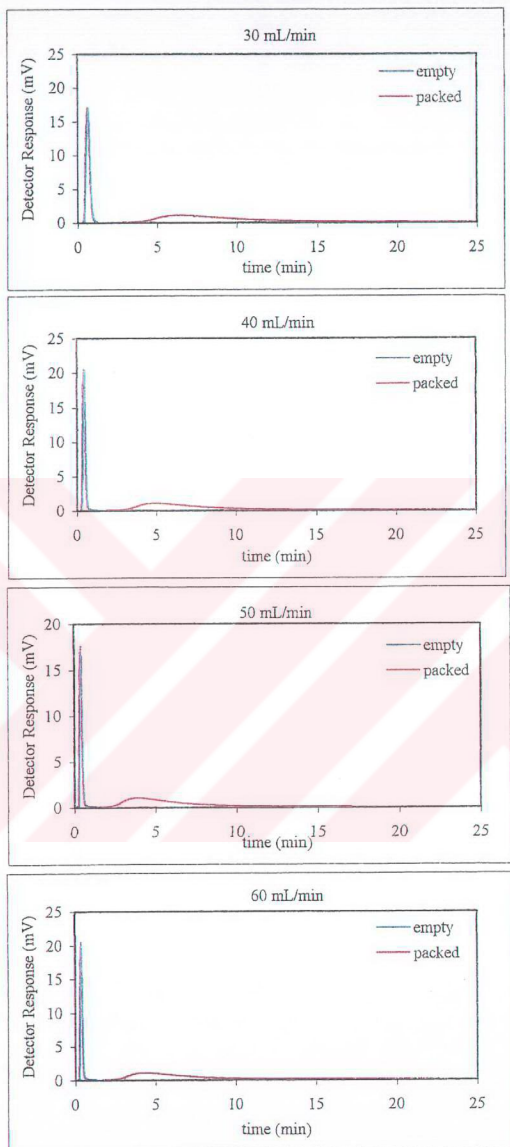
Figure 7.13. Chromatographic response peaks for empty and packed columns (80°C)
