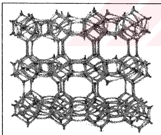
Figure 3.4. Clinoptilolite framework system
