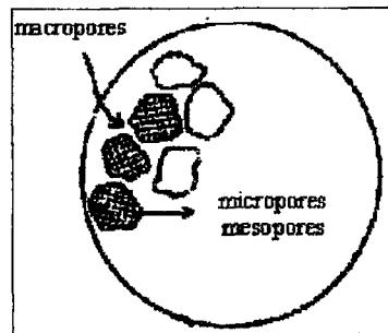
Figure 4.2. Schematic diagram for the biporous adsorbent particle [38]
