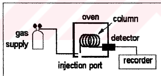
Figure 4.9. Schematic diagram of a gas chromatograph
