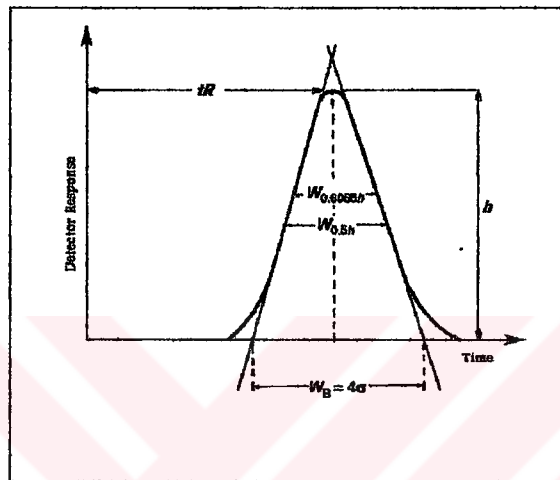
Figure 4.11. Pulse injection and response peak
