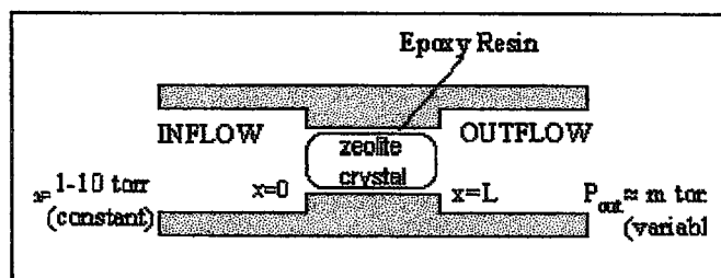
Figure 4.4. Schematic diagram of the membrane technique
