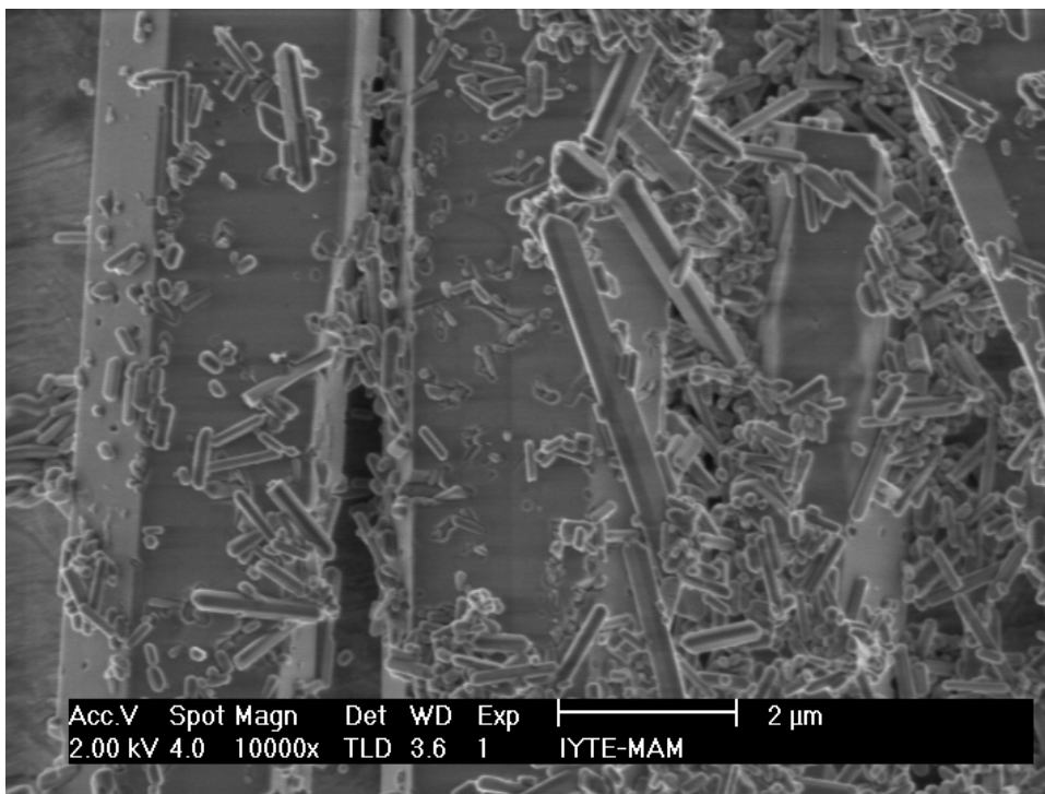
Figure 5.29 (b). SEM image of KNW4 whiskers synthesized at 875°C for 2 h where salt mixture/HA ratio during preparation was 3/1.
