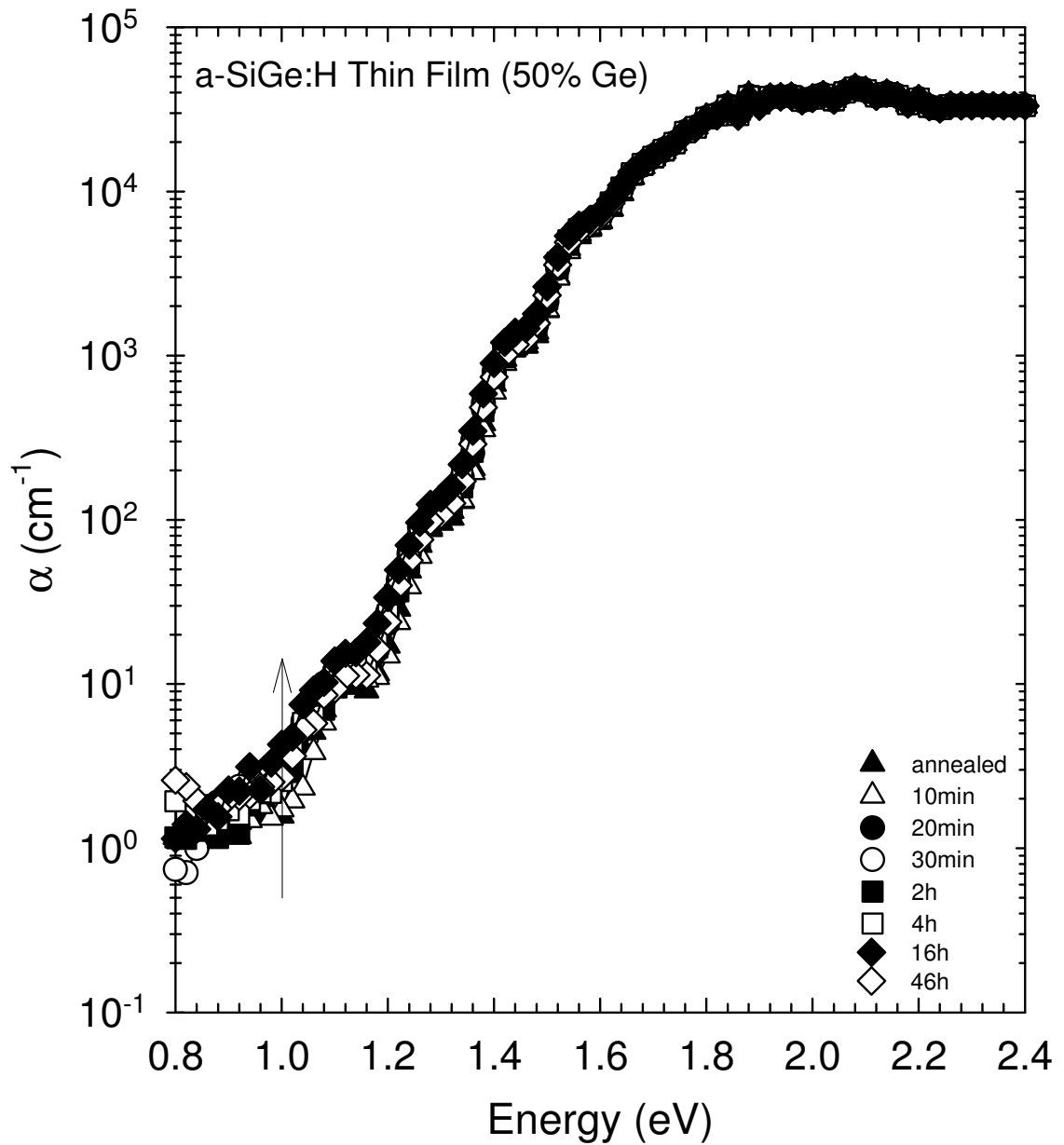
Figure 4.17 Absolute absorption spectrum of the sample with 50% Ge, for various light soaking intervals, calculated from the Y_{\text{DBP}} spectrum and simultaneously measured transmission signals.
