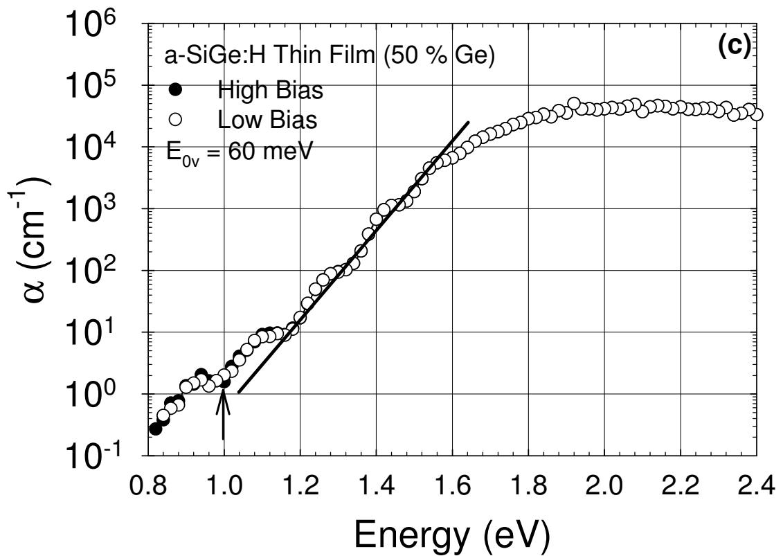
Figure 3.8 c) The calculated absolute \alpha ( h\nu ) spectra of DBP for high and low bias light measurements of a-SiGe:H thin film with 50 % Ge concentration.
