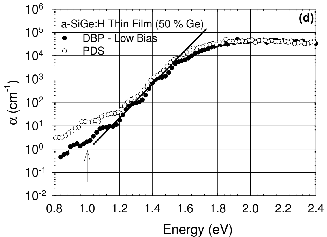
Figure 3.8 d) The calculated absolute \alpha ( h\nu ) spectra of PDS and DBP for low bias light measurements of a-SiGe:H thin film with 50% Ge concentration.
