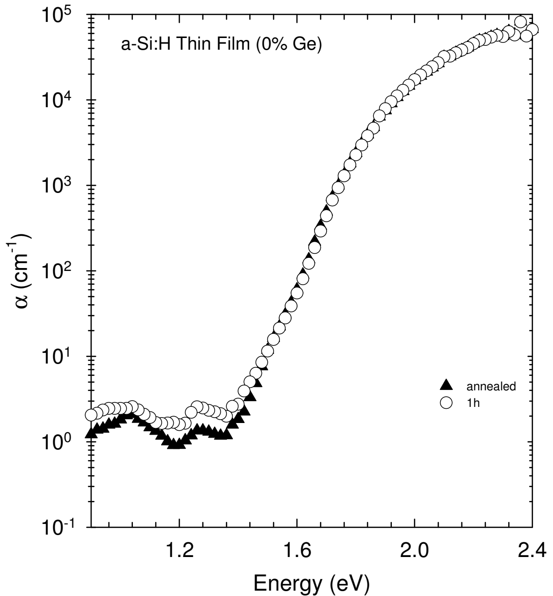
Figure 4.8 Absolute absorption spectrum of the sample with 0% Ge, for annealed and 1h light soaked states, calculated from the Y_{DBP} spectrum and simultaneously measured transmission signals.
