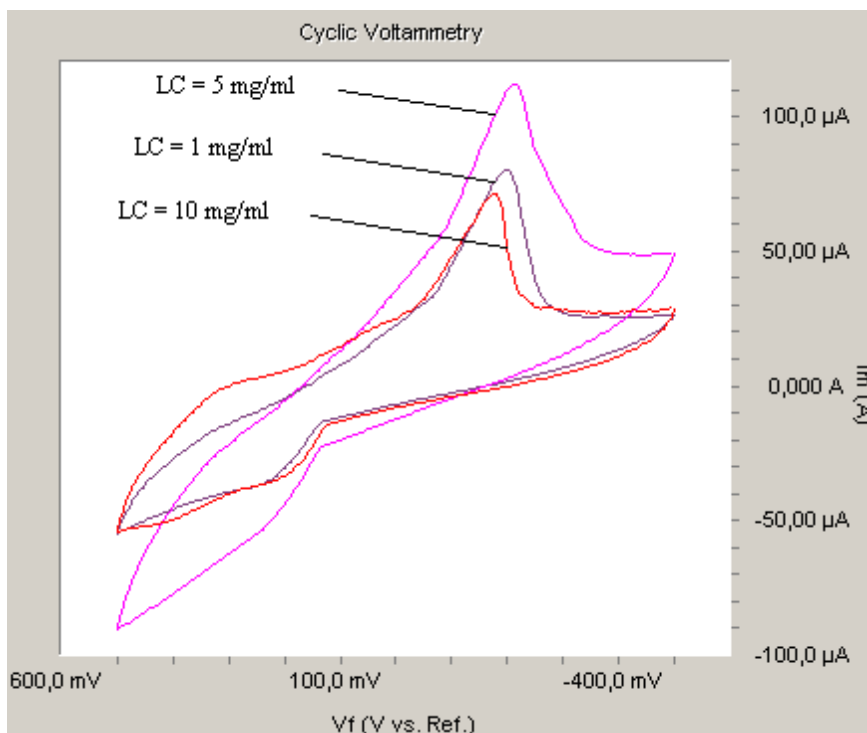
Figure 4.21. Cyclic voltammograms of biosensors with laccase concentration of 1, 5 and 10 mg/ml when GA = 17.01 % vol. of the biosensor bottom part (oleuropein concentration of 2 mg/ml, at 25 °C with \pm 0.5 V and 10 mV/s scan rate)
