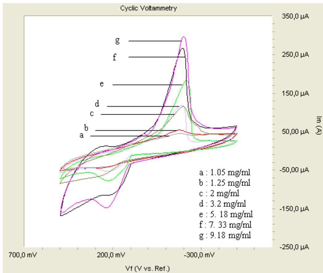
Figure 4.30. Cyclic voltammograms of oleuropein solutions in a temperature of 25 °C, scan rate of 10 mV/s and the potential range of -0.5 to 0.5 V
