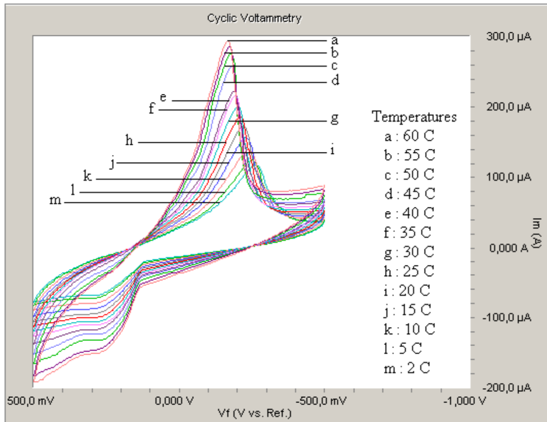
Figure 4.29. Cyclic voltammograms of laccase biosensor for 2 mg/ml oleuropein solution, in \pm 0.5 V potential interval, with 10 mV/s scan rate, at various temperatures
