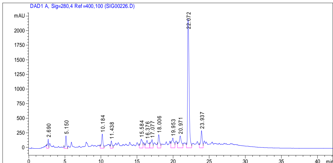
Figure 4.2. Chromatogram of olive leaf crude extract after the fourth loading procedure
