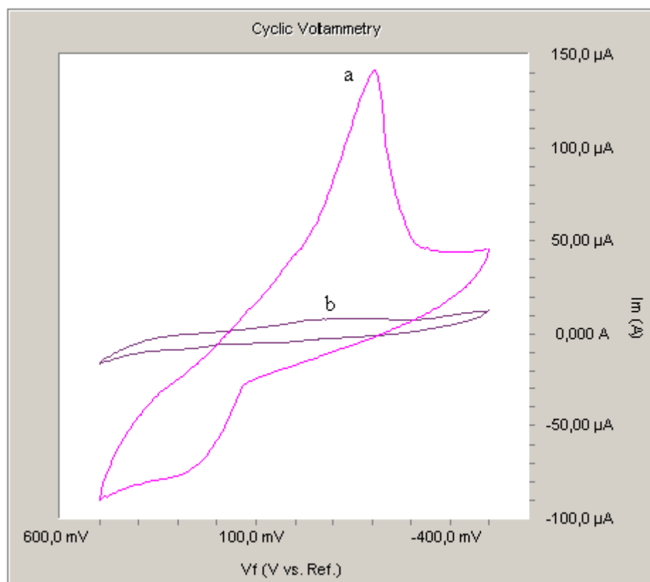
Figure 4.18. Cyclic voltammograms of (a) laccase biosensor and (b) electrochemical sensor in 2 mg/ml of oleuropein concentration at 25 °C with \pm 0.5 V and 10 mV/s scan rate
