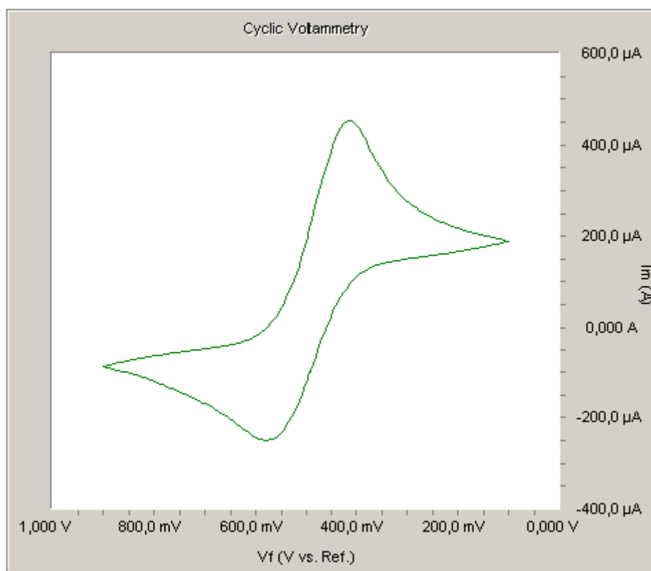
Figure 4.16. Voltammogram of 1.25 M FeCl 3 solution at 25°C and 10mV/s scan rate
