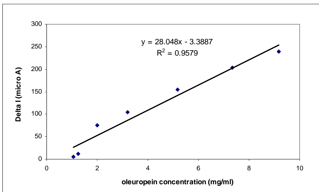
Figure 4.31. Calibration curve for oleuropein
