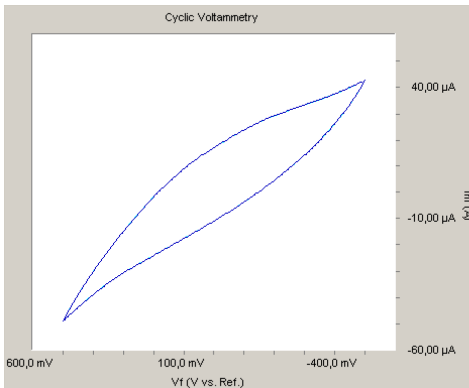
Figure 4.40. Cyclic voltammogram of laccase biosensor in 2 mg/ml of rutin
