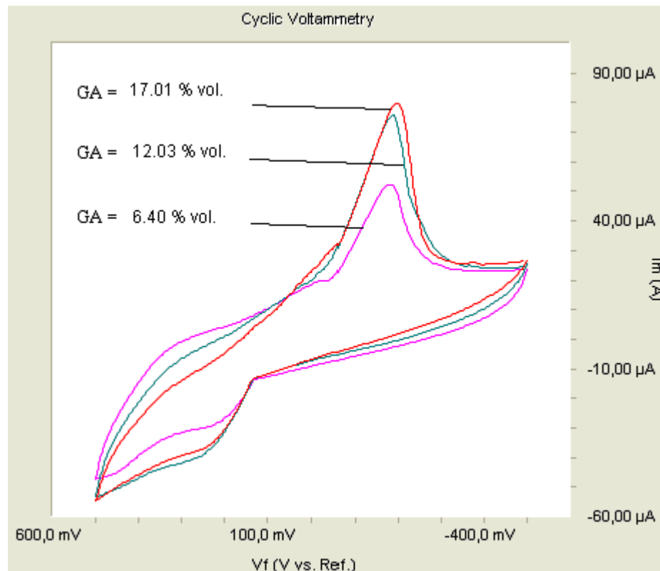
Figure 4.23. Cyclic voltammograms of biosensors with glutaraldehyde amount of 6.40, 12.03 and 17.01 % vol. of the biosensor bottom part when LC = 1 mg/ml (oleuropein concentration of 2 mg/ml, at 25 °C with \pm 0.5 V and 10 mV/s scan rate)
