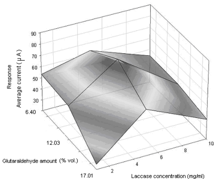
Figure 4.26. Graphical representation of the average cathodic peak current with respect to laccase concentration and glutaraldehyde amount
