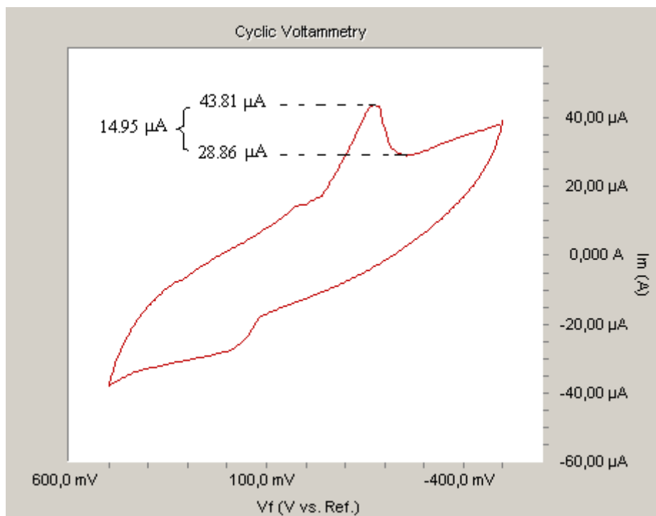
Figure 4.36. Cyclic voltammogram of laccase biosensor in 3 mg/ml of FIV
