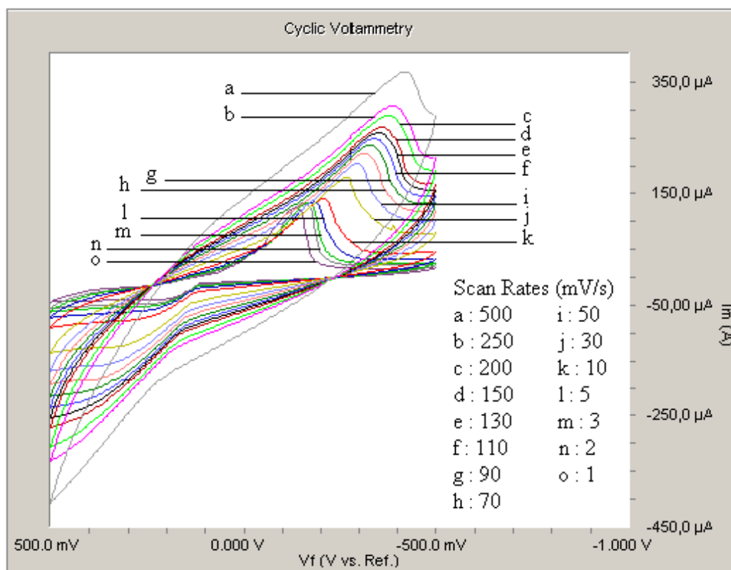
Figure 4.27. Cyclic voltammograms of laccase biosensor for 2 mg/ml oleuropein solution, at 25°C, in \pm 0.5 V potential interval, with various scan rates
