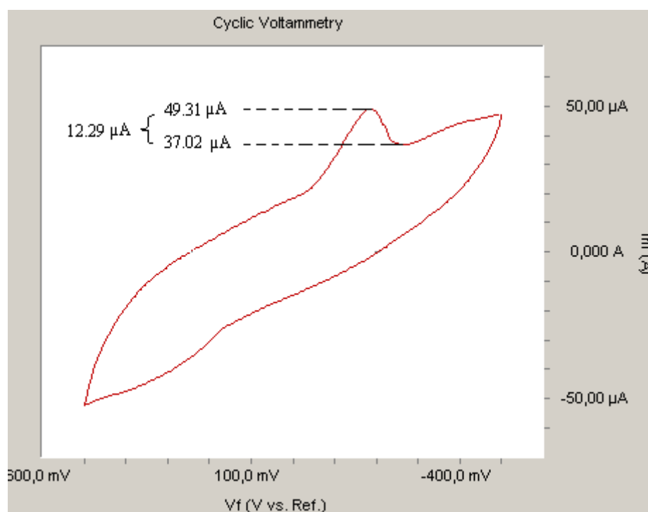
Figure 4.37. Cyclic voltammogram of laccase biosensor in 3 mg/ml of FV
