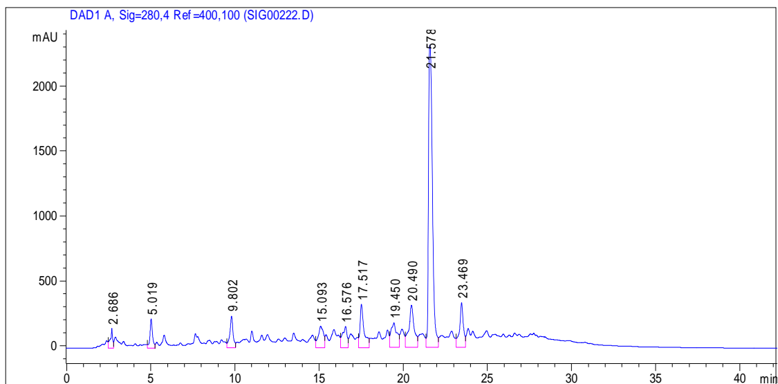
Figure 4.1. Chromatogram of olive leaf crude extract
