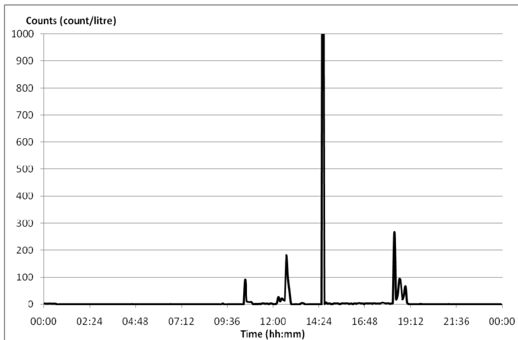
Figure 9.30. 0.3 micron particle count, October 25 th (counts/liter)
