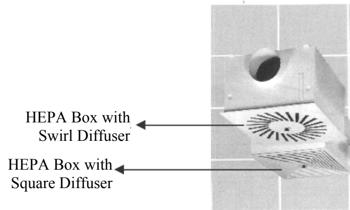
Figure 8.6. Swirl and square diffusers and HEPA filter boxes
