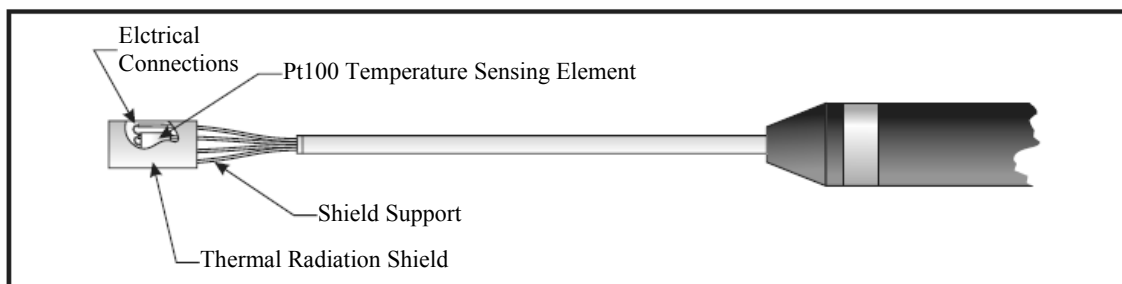
Figure 9.5. MM0034 air temperature transducer (Source: LumaSense Technologies A/S 2005)
