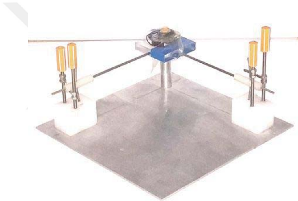
Figure 3.3. The IMU testing platform
