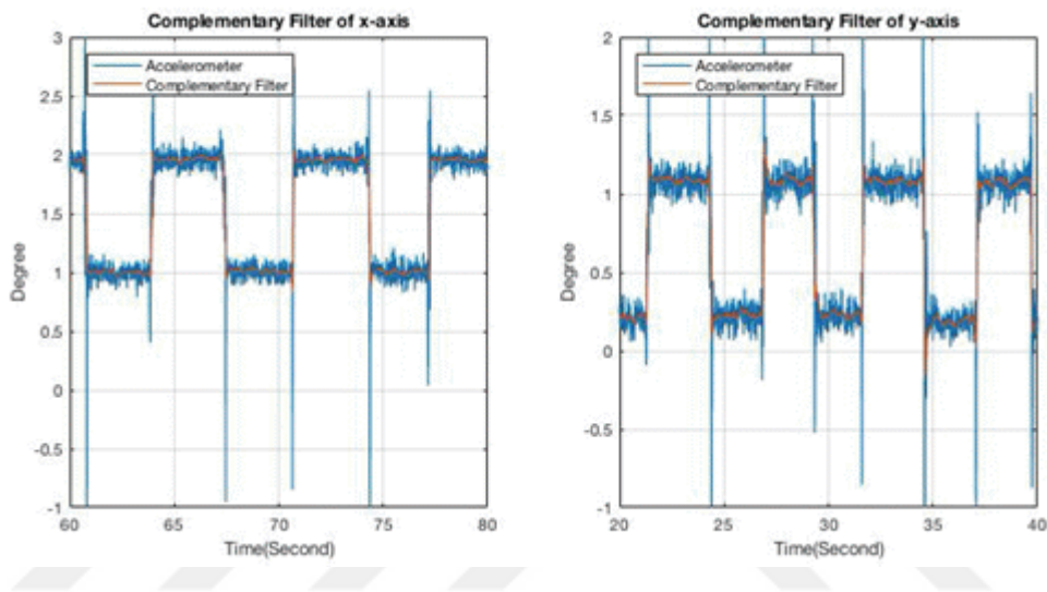
Figure 3.10. Angle calculation by using accelerometer and complementary filter
