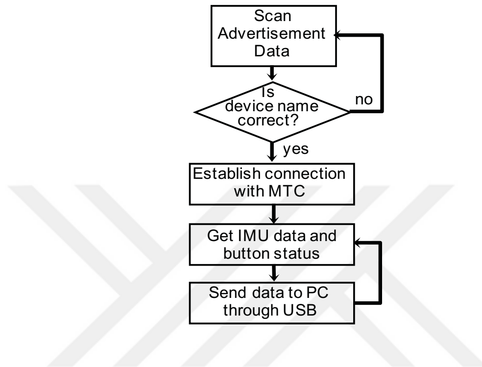
Figure 4.8. Operations of the scanner card
