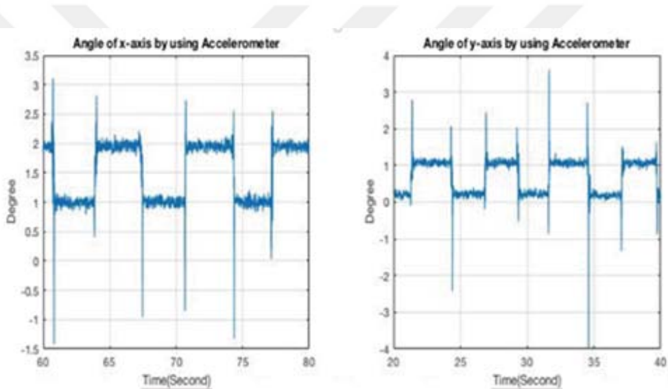
Figure 3.5. Angle calculation by using accelerometer in motion
