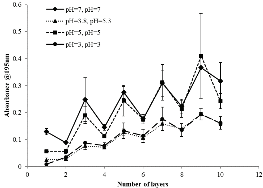
Figure 3.3. Monitoring the effect of solution pH on Lysozyme-Gum Arabic multilayer formation by UV-Vis spectroscopy. (The absorbances at 195 nm was monitored. Adsorption time was 20 minute. Error bars represent the standard deviations).
