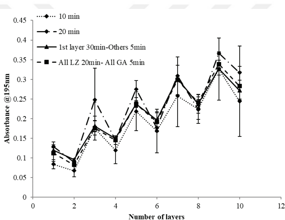
Figure 3.4. Monitoring the effect of adsorption time on Lysozyme-Gum Arabic multilayer deposition at pH 7&7 combination by UV-Vis spectroscopy. (The absorbances at 195 nm was monitored. Error bars represent the standard deviations).
