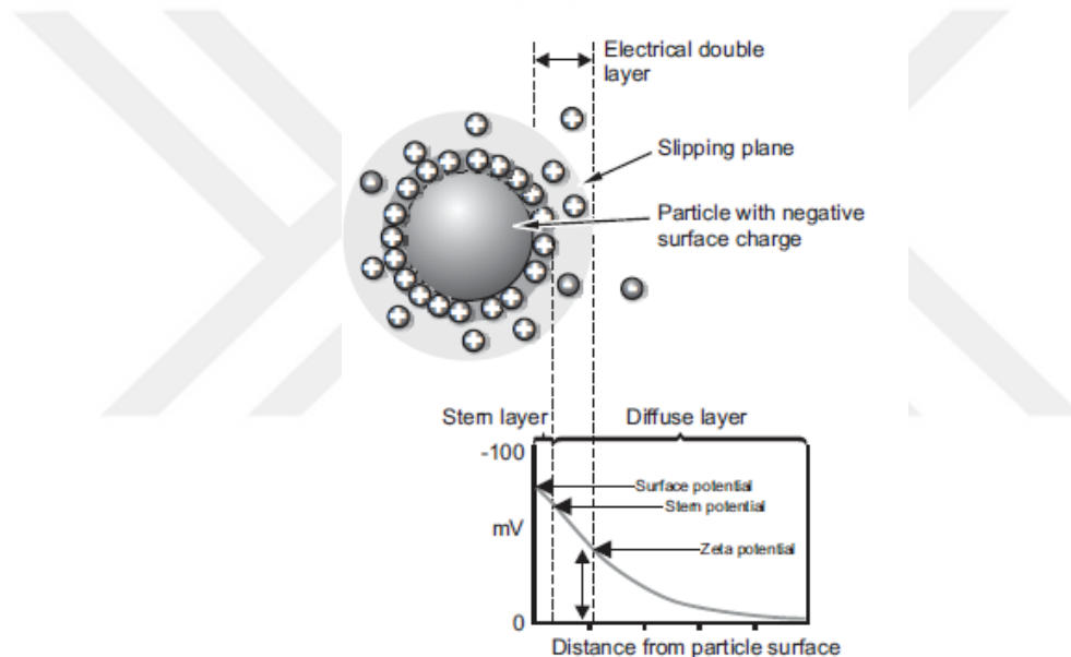
Figure 3.1. Zeta Potential of a particle with negative surface charge (Source: Nanotechnology in Soil Science, 2015).
