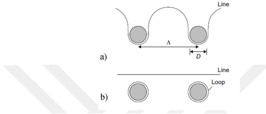
Figure 2.8. Schematic drawing of Orowan strengthening mechanism a) The line bows between the obstacles b) Orowan loops (Source Bacon, 2011)
