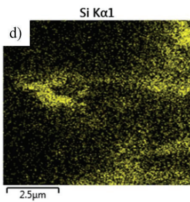
Figure 4.5. EDX mapping of A360 / 0.5 wt.% GNPs
