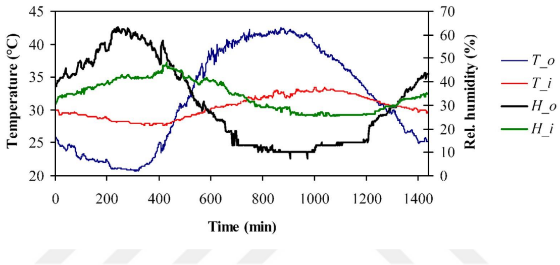
Figure 2.1. Temperature (indicated T) and relative humidity (indicated H) variations at the inside (indicated i) and outside (indicated o) of the domed houses, (Source: [20])
