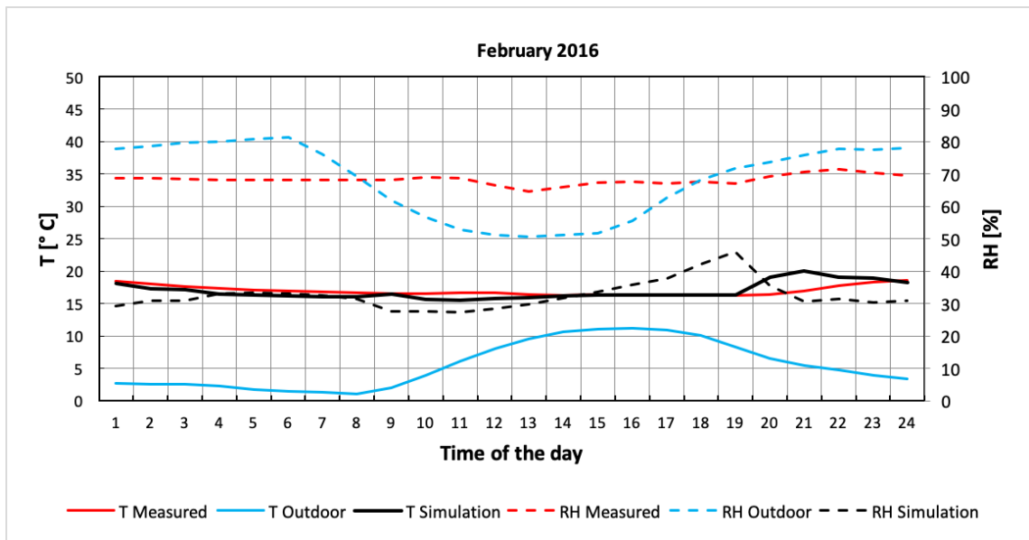
Figure A 18. Daily average of February 2016 [32]
