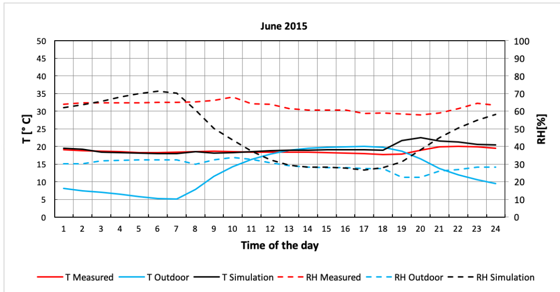
Figure A 1. Daily average of June 2015 [32]
