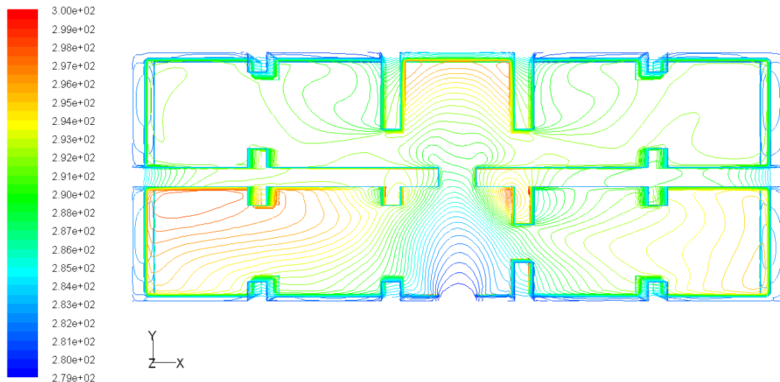
Figure 2.2. Temperature (K) distribution of the inside of the house at 1m high level, (Source: [20])
