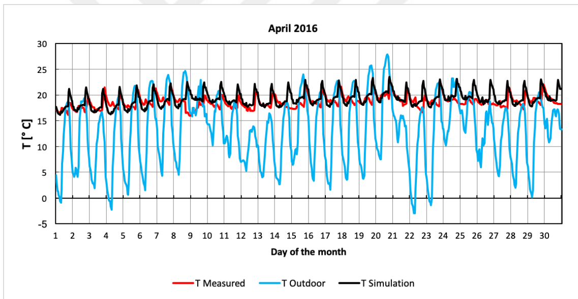
Figure 6.16. Measured, simulated interior and outdoor temperatures versus day of the month graph, April 2016
