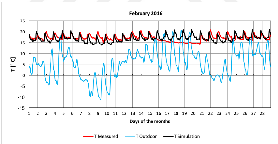
Figure A 20. Measured, simulated interior and outdoor temperatures versus day of the month graph, February 2016
