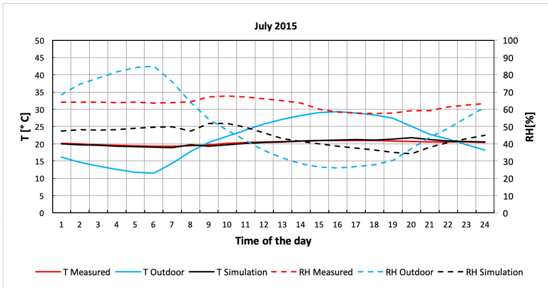
Figure 6.3. Daily Average of July 2015 [32]
