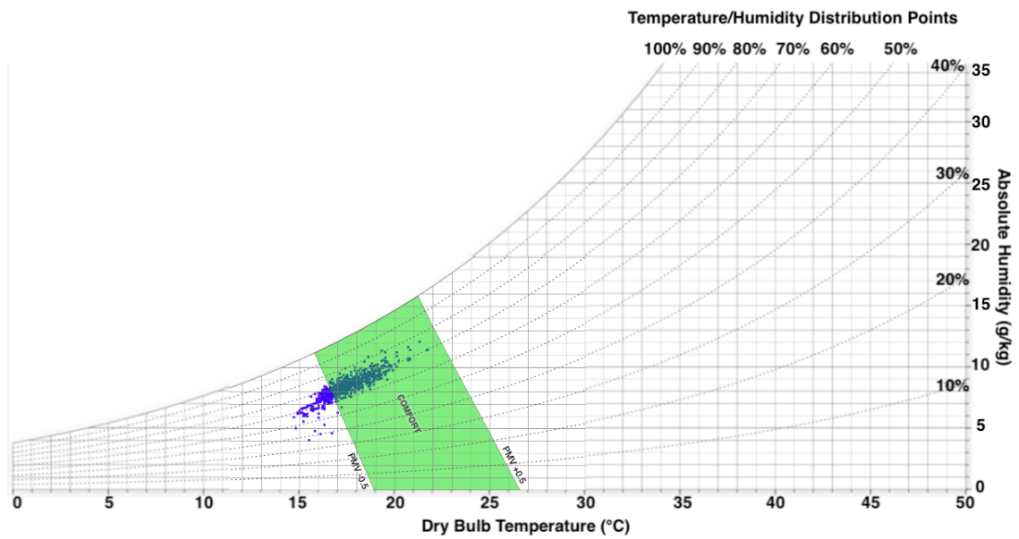
Figure A 24. Hourly temperature, humidity distribution on psychrometric chart, February 2016 [33], (Source: [43])
