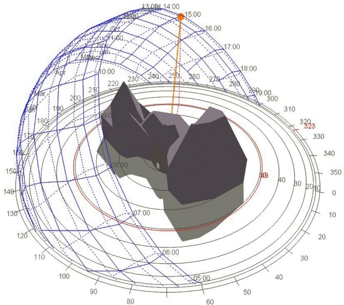
Figure 5.2. The 3D model of the cave dwelling and the solar radiation pattern
