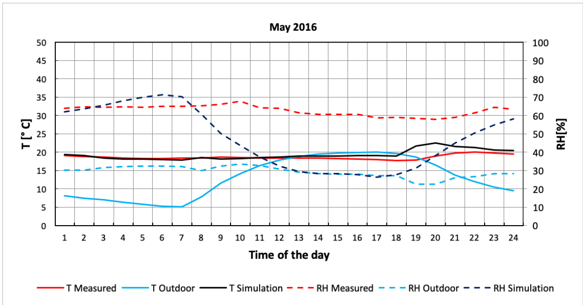
Figure A 26. Daily average of May 2016 [32]
