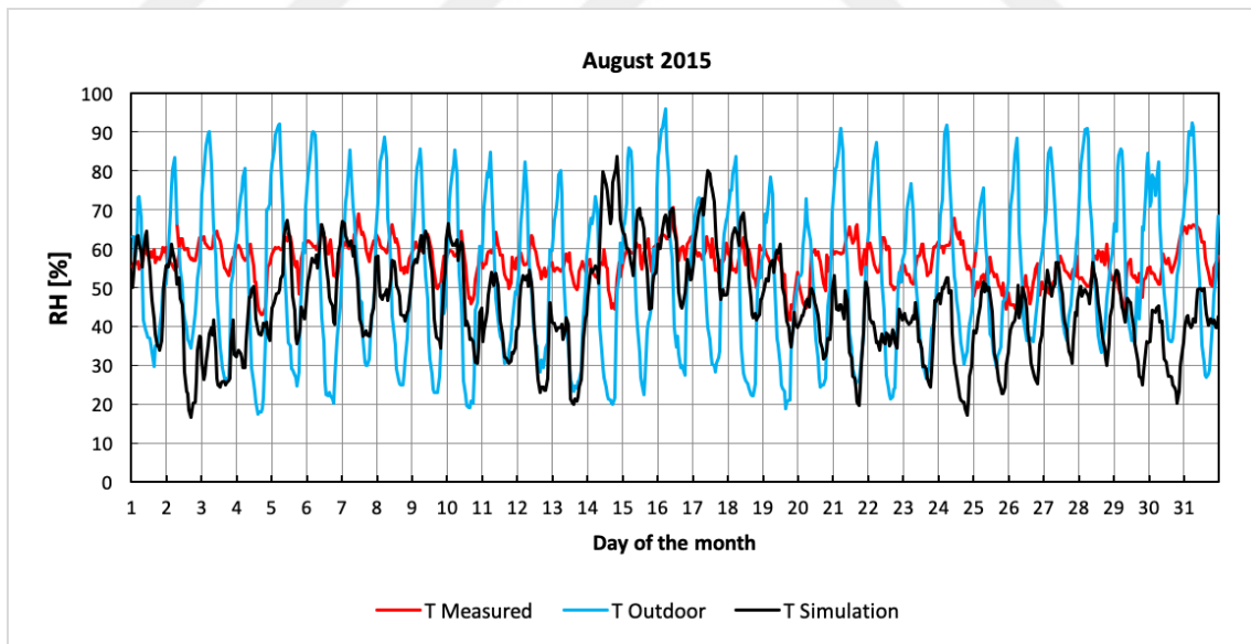
Figure A 6. Measured, simulated interior and outdoor relative humidity versus day of the month graph, August 2015
