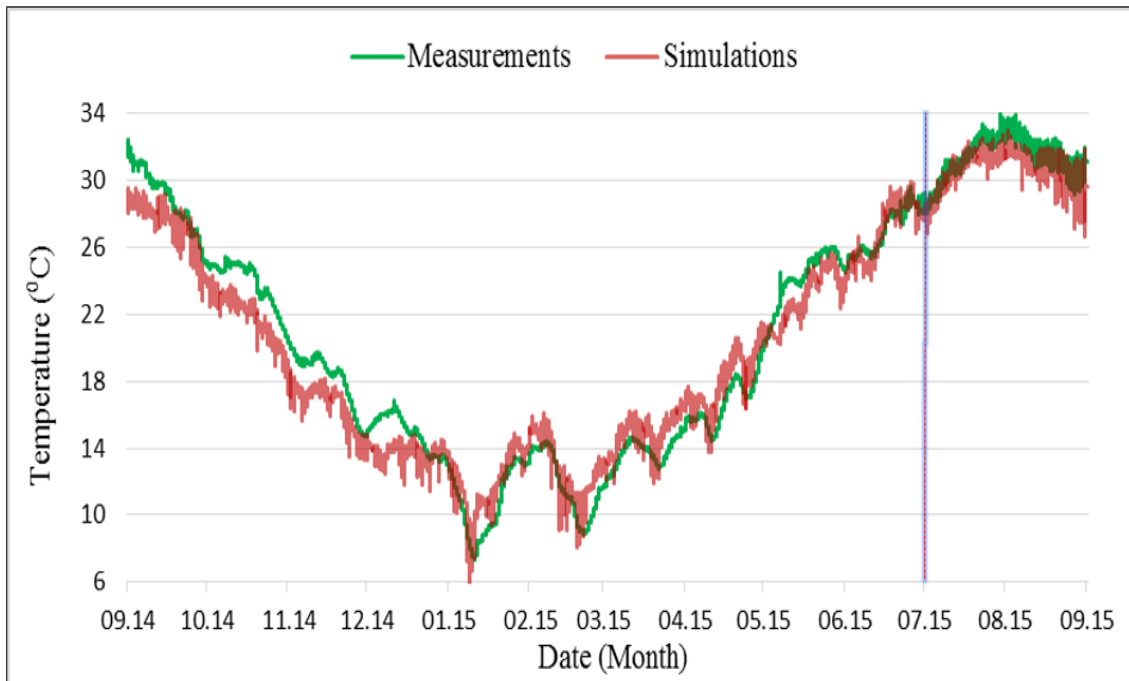
Figure 2.6. Measured and simulation temperature graph, (Source: [24])
