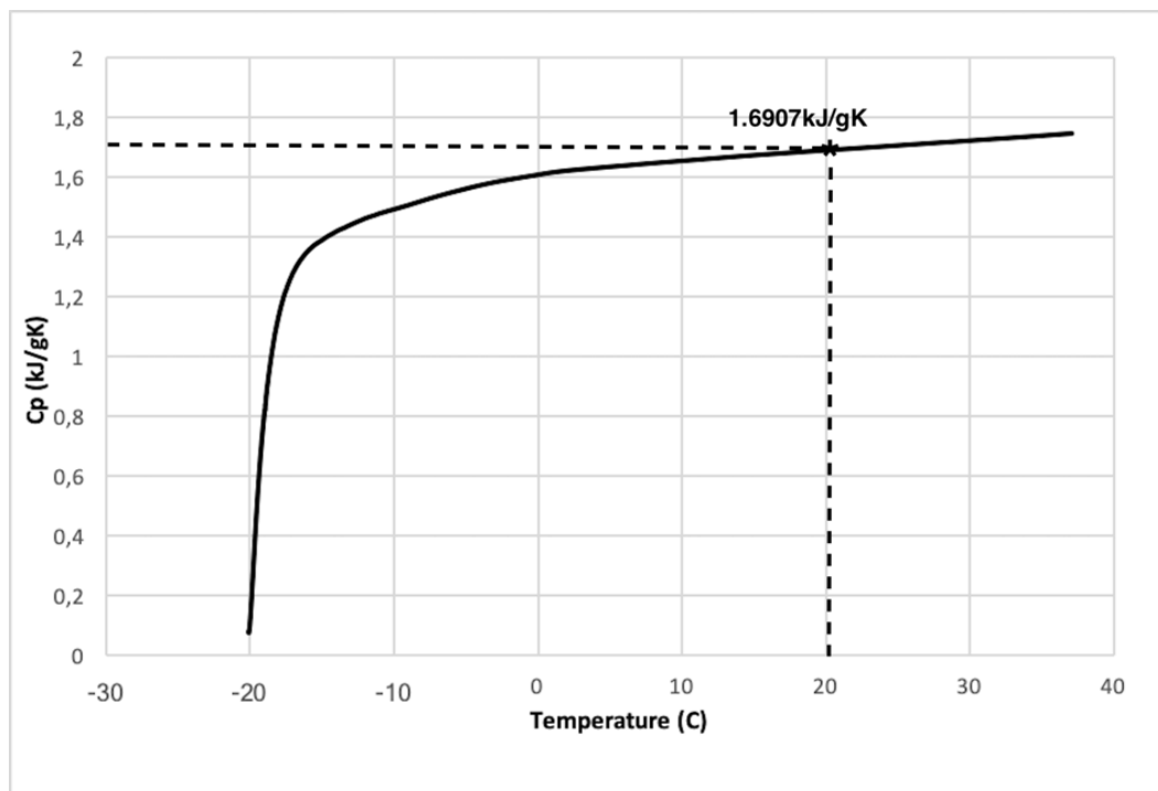
Figure 4.10. The temperature function of the specific heat.
