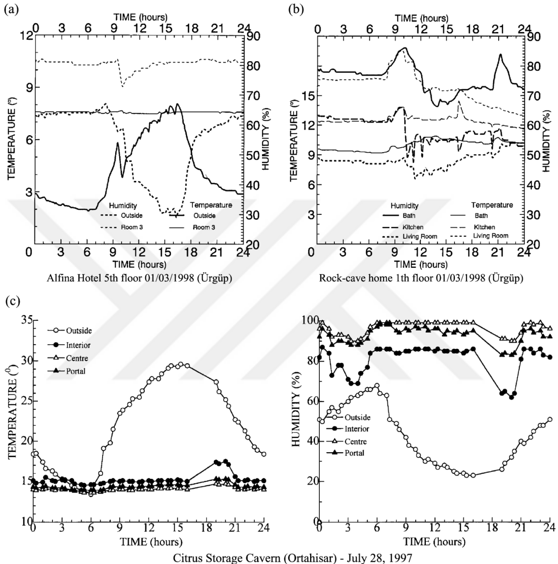
Figure 2.3. Variation of temperature and humidity in different modern rock settlements (a and b) and in a storage cavern (c) at the Cappadocia Region as documented by Aydan and Ulusay, (Source: [21])
