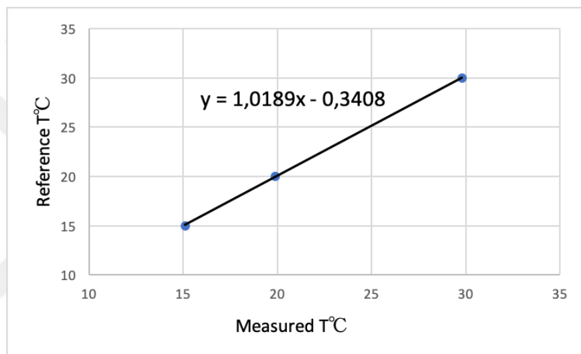
Figure 4.4. Temperature correction function
