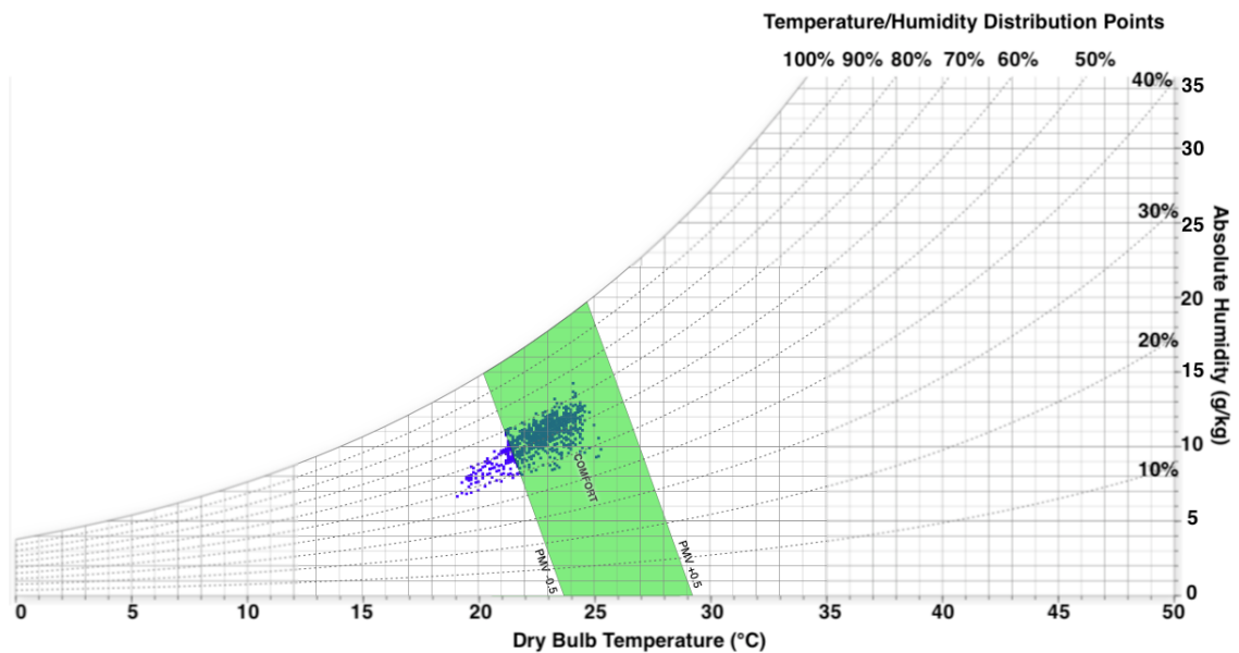
Figure A 8. Hourly temperature, humidity distribution on psychrometric chart, August 2015 [33], (Source: [43])
