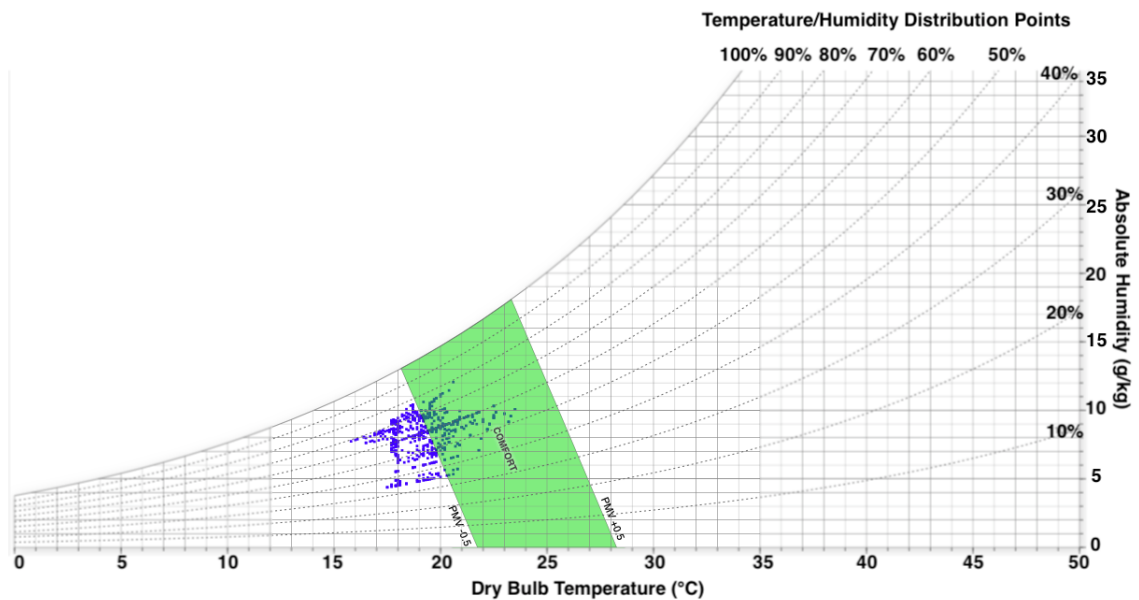
Figure A 16. Hourly temperature, humidity distribution on psychrometric chart, October 2015 [33], (Source: [43])
