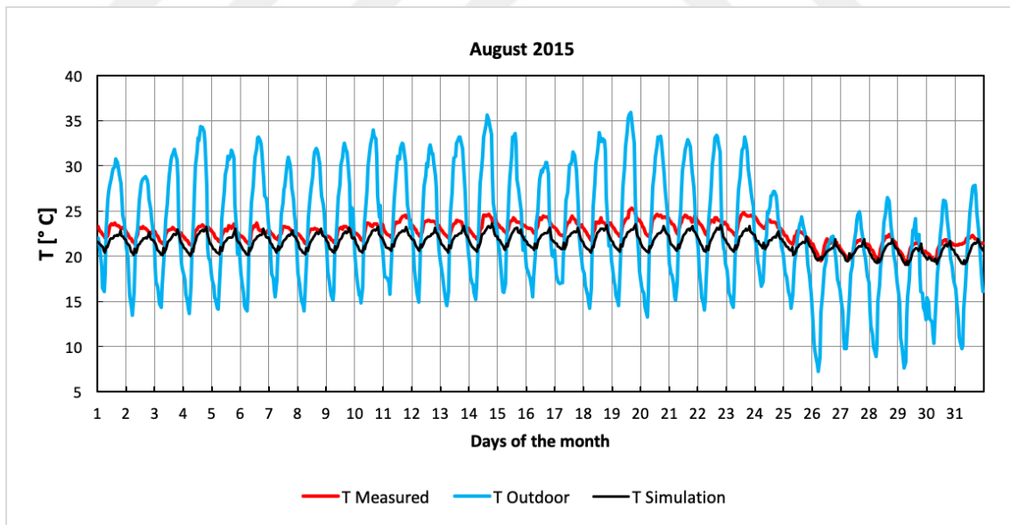
Figure A 4. Measured, simulated interior and outdoor temperatures versus day of the month graph, August 2015
