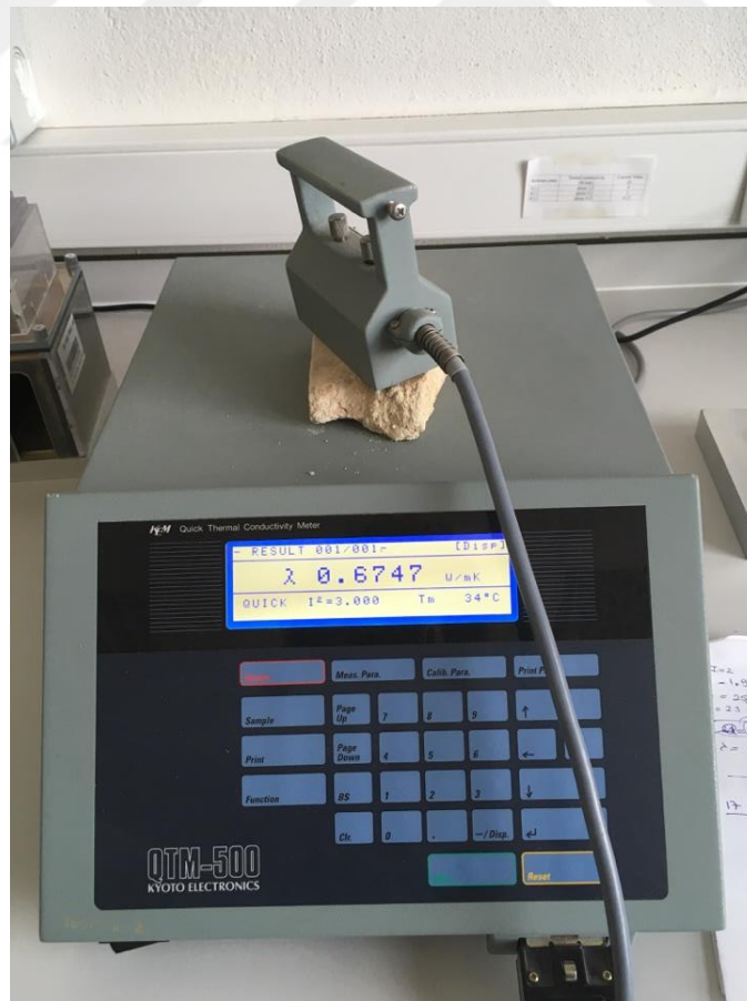
Figure 4.7. Thermal conductivity measurement with KEM QTM 500.
