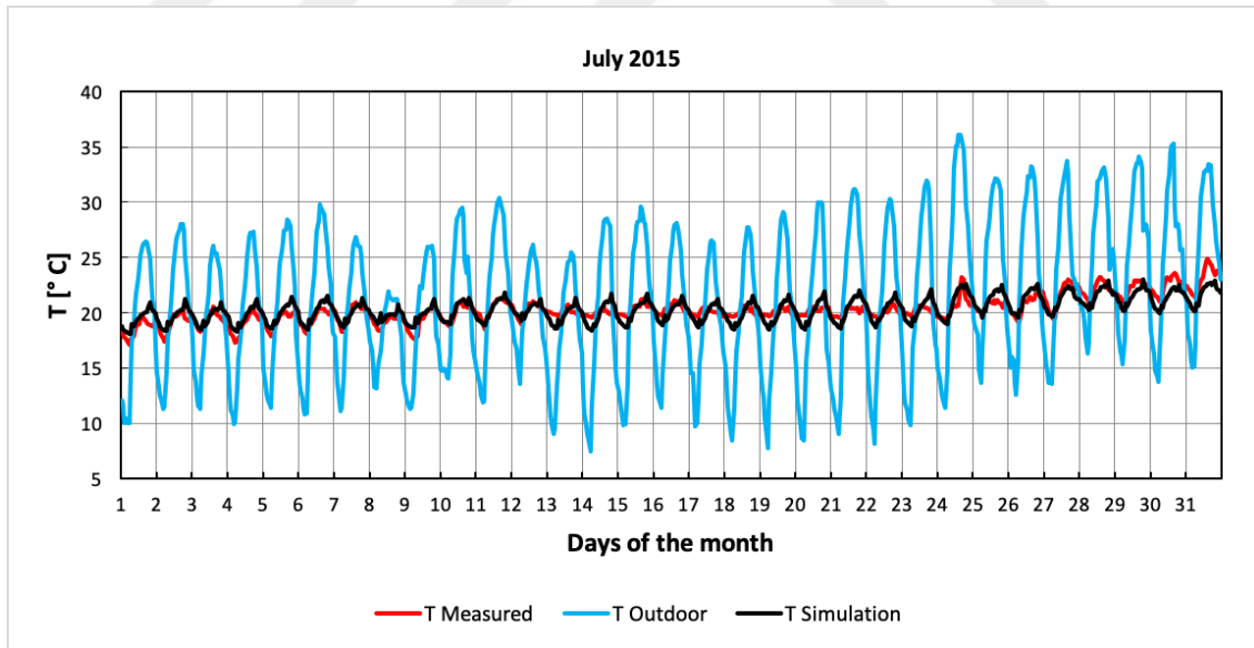
Figure 6.4. Measured, simulated interior and outdoor temperatures versus day of the month graph, July 2015
