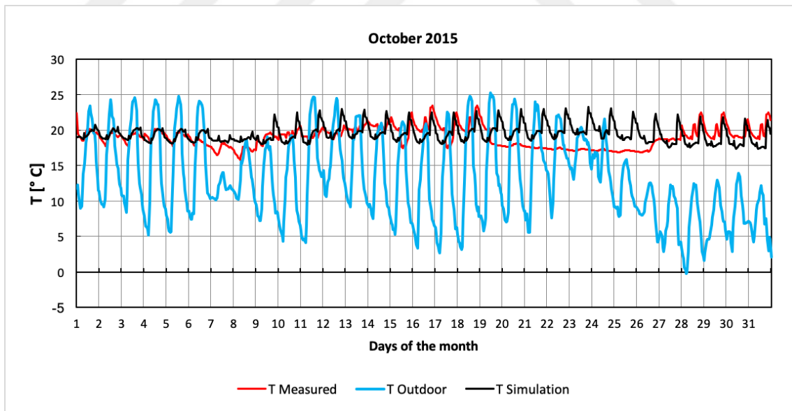
Figure A 12. Measured, simulated interior and outdoor temperatures versus day of the month graph, October 2015
