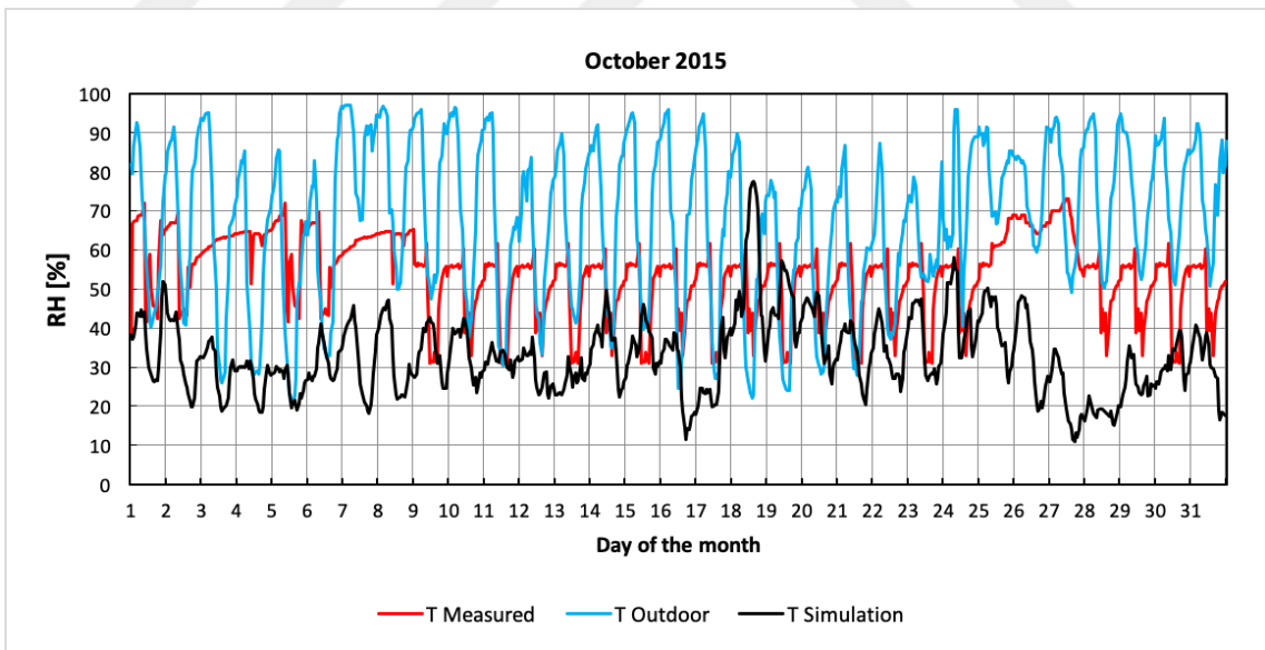
Figure A 14. Measured, simulated interior and outdoor relative humidity versus day of the month graph, October 2015
