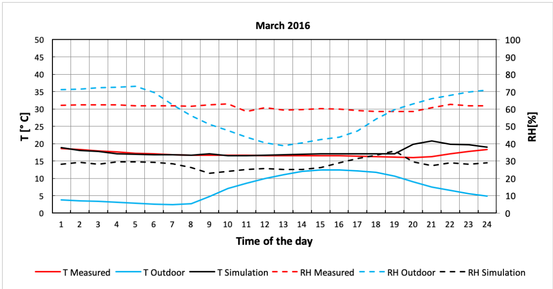
Figure A 25. Daily average of March 2016 [32]
