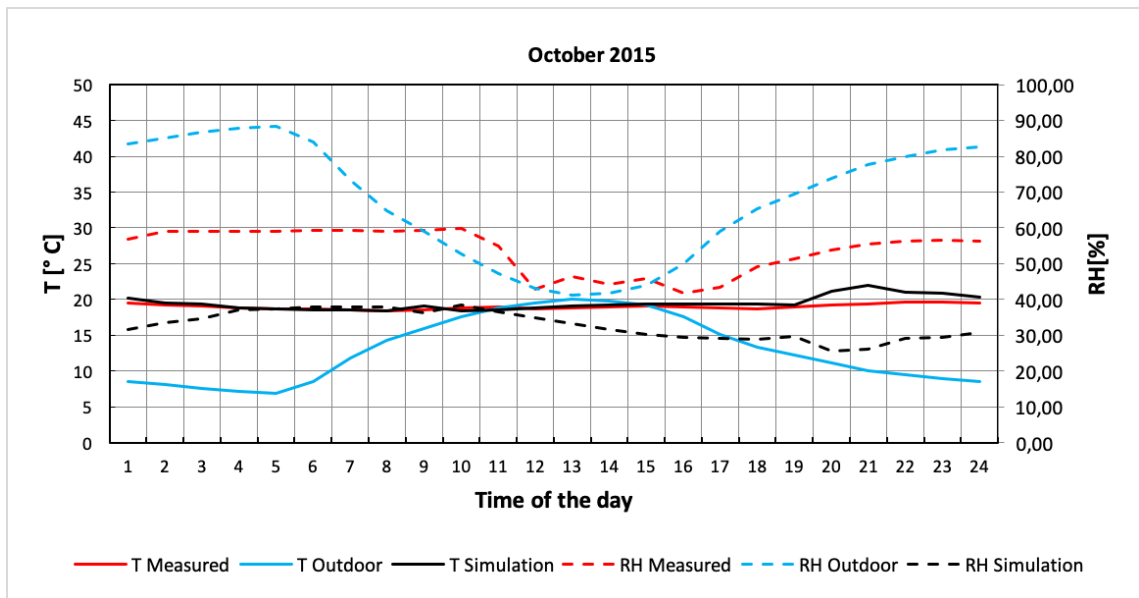
Figure A 10. Daily average of October 2015 [32]
