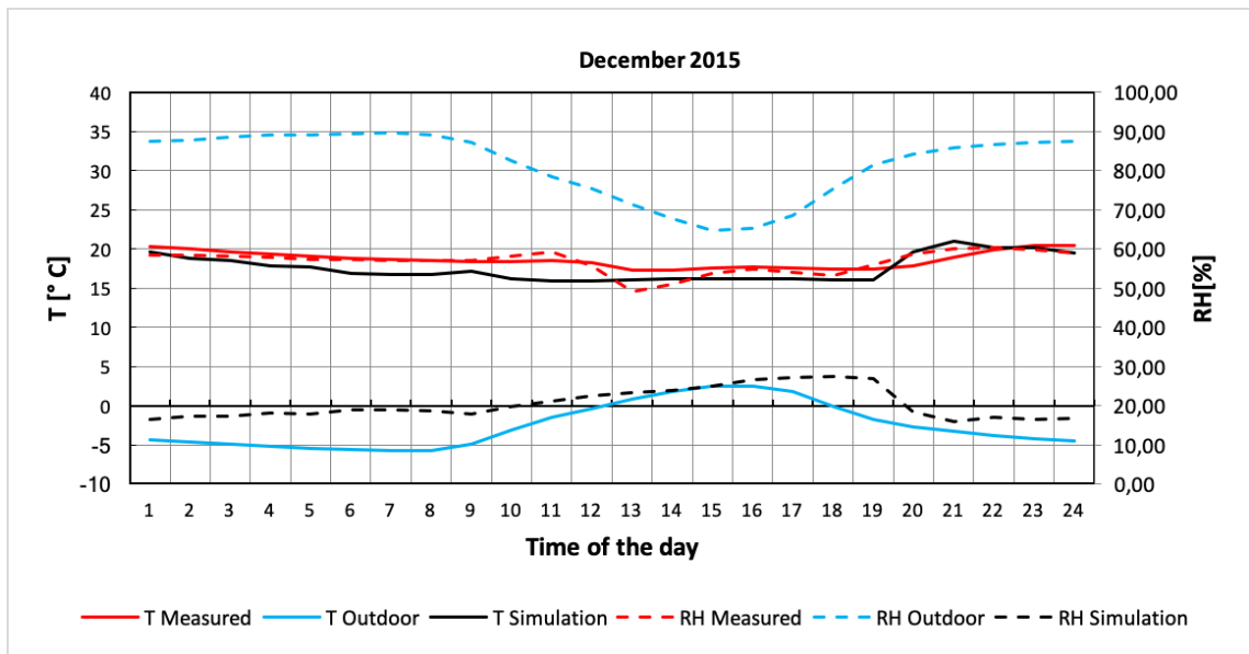
Figure A 17. Daily average of December 2015 [32]
