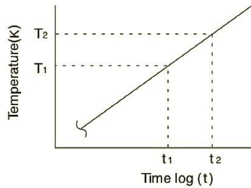
Figure 4.6. KEM QTM 500 Principle of thermal conductivity calculation, (Source: [31])
