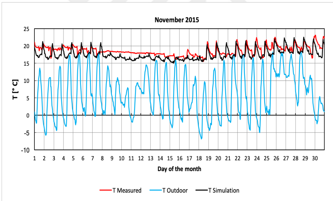
Figure 6.8. Measured, simulated interior and outdoor temperatures versus day of the month graph, November 2015
