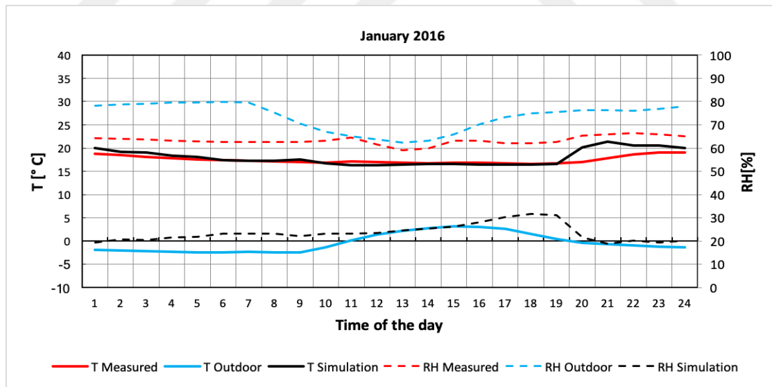
Figure 6.11 Daily Average of January 2016 [32]
