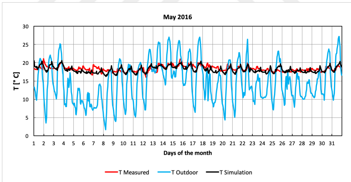
Figure A 28. Measured, simulated interior and outdoor temperatures versus day of the month graph, May 2016
