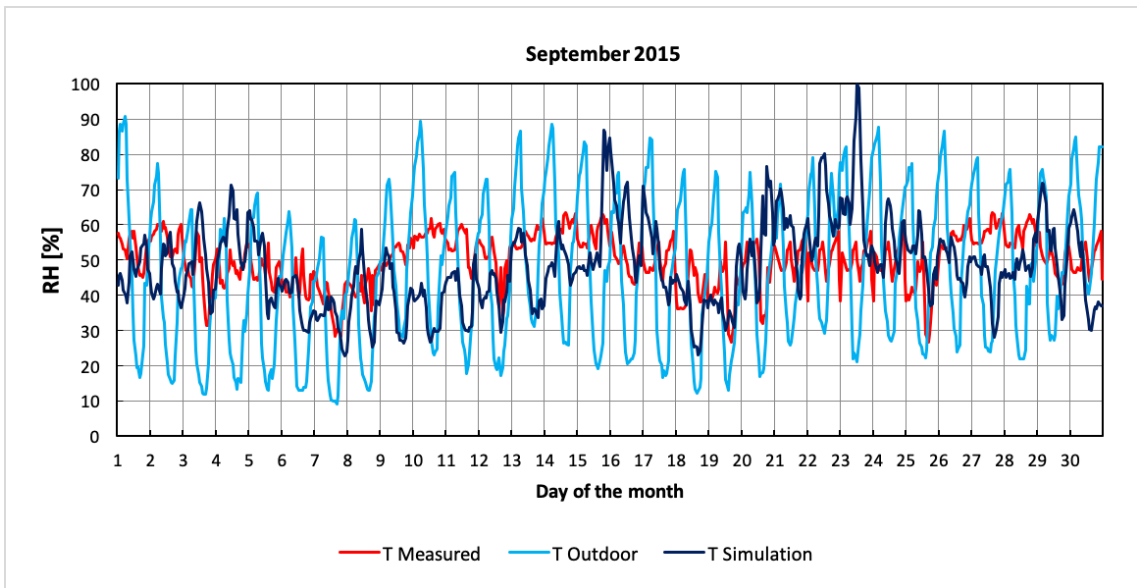
Figure A 13. Measured, simulated interior and outdoor relative humidity versus day of the month graph, September 2015
