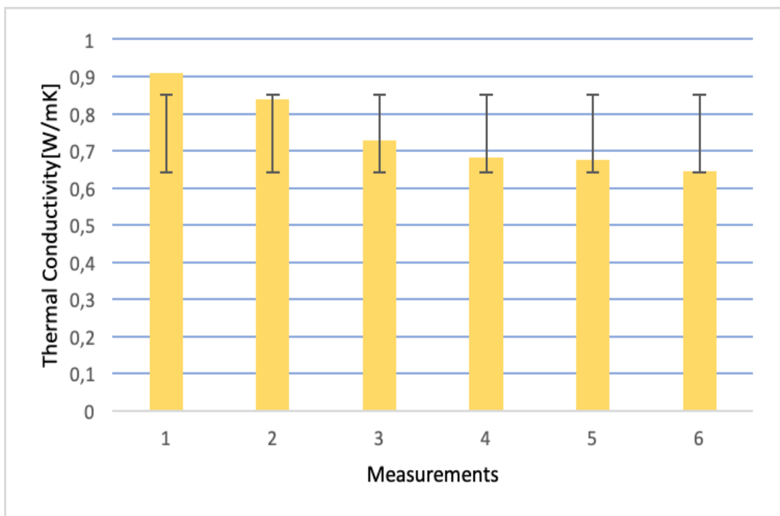
Figure 4.8. Thermal conductivity measurements with standard deviation error bar
