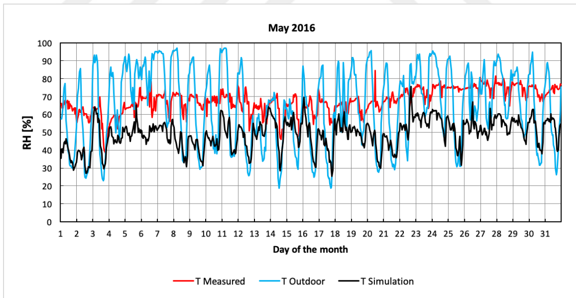
Figure A 30. Measured, simulated interior and outdoor relative humidity versus day of the month graph, May 2016
