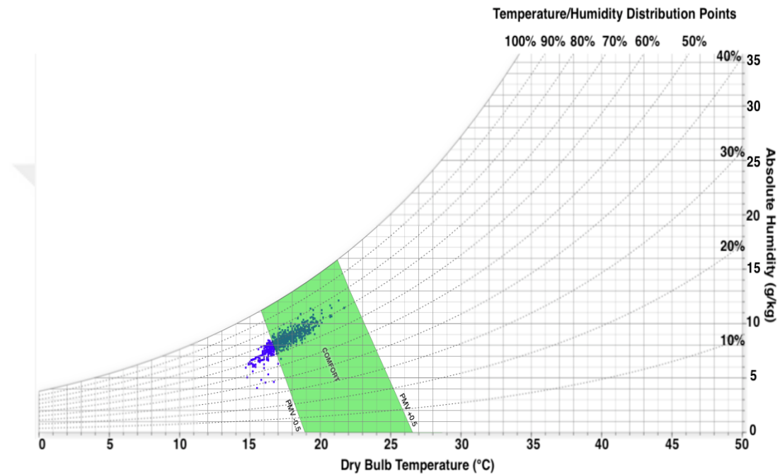
Figure 6.14. Hourly temperature, humidity distribution on psychrometric chart, January 2016 [33], (Source: [43])
