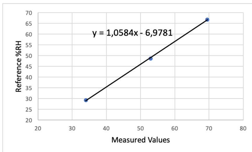
Figure 4.5. Relative humidity calibration function
