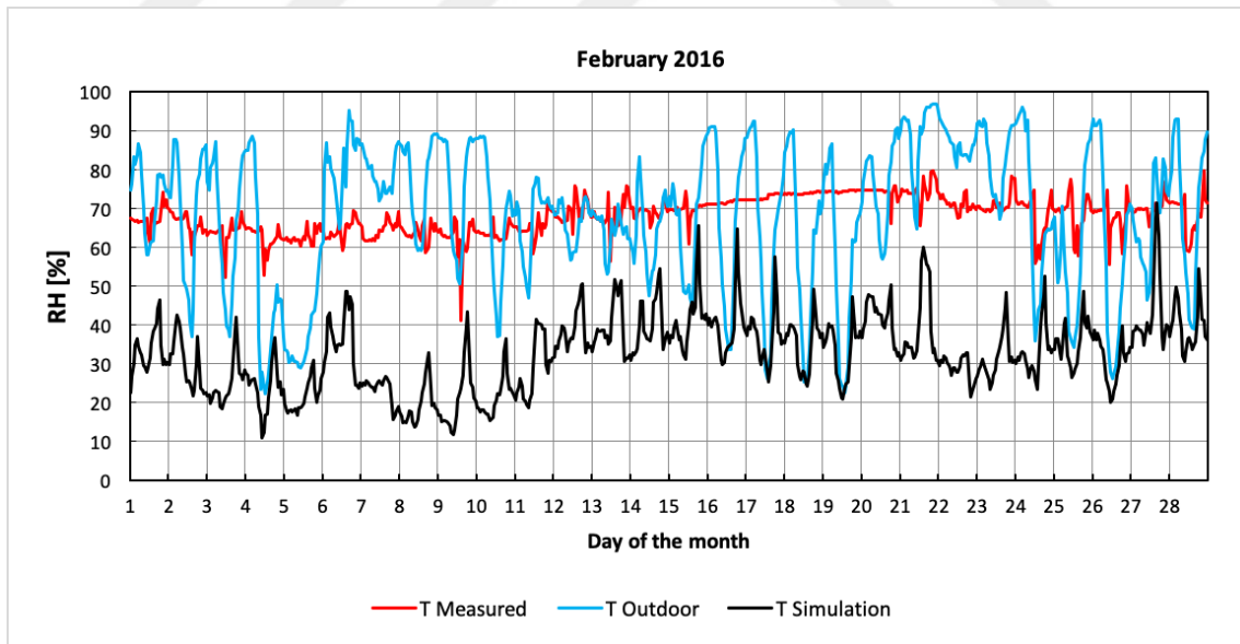
Figure A 22. Measured, simulated interior and outdoor relative humidity versus day of the month graph, February 2016
