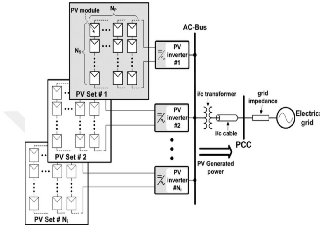
Figure 3.4: Block diagram of the large PV plant [31].
