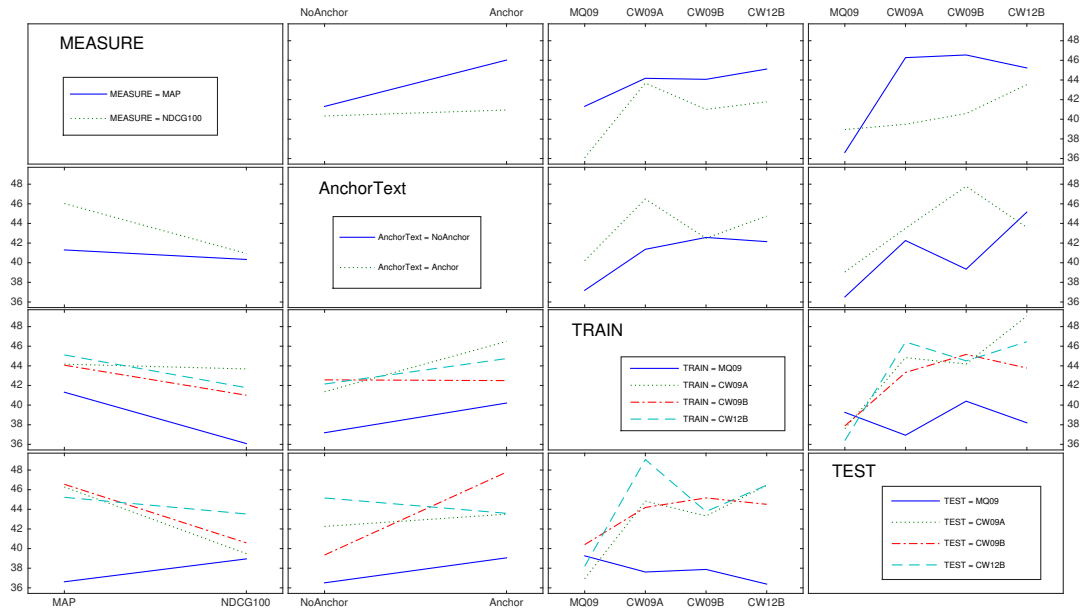
Figure 6.10. Classification Accuracy Interaction Plot of cross-collection experiments for selective term-weighting approach SEL.
