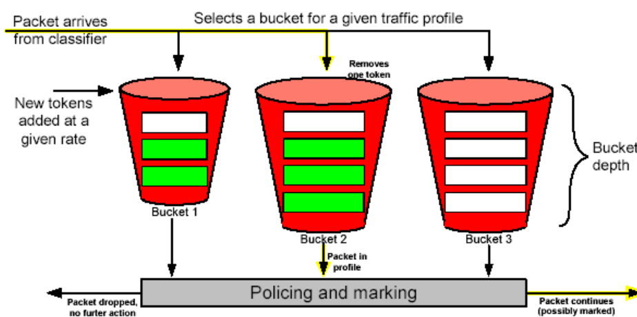
Figure 3.3 Token buckets providing a simple metering function.
