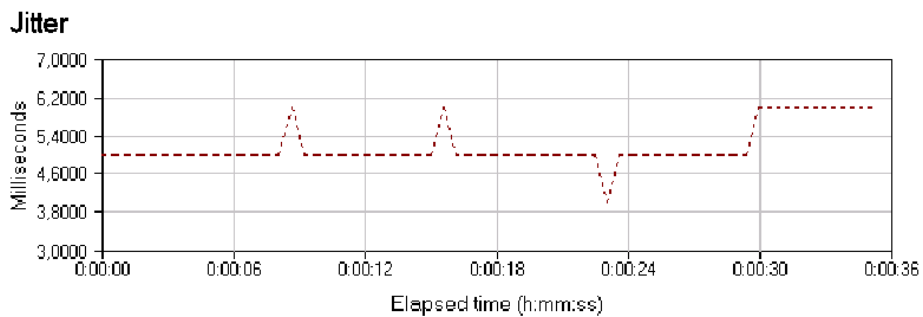
Figure 5.2 Measured Intserv Controlled Load jitter performance (mean 5.170ms).
