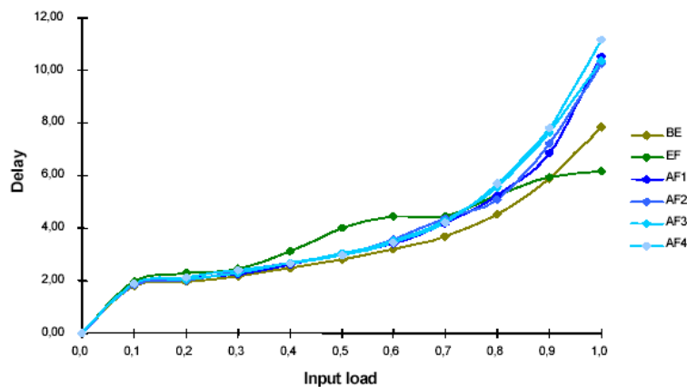
Figure 5.13 Measured Delay for Diffserv
