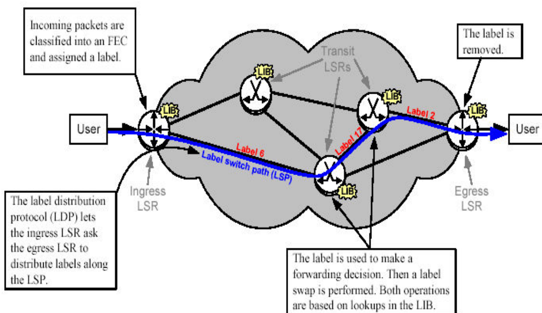
Figure 4.2 The MPLS functionality
