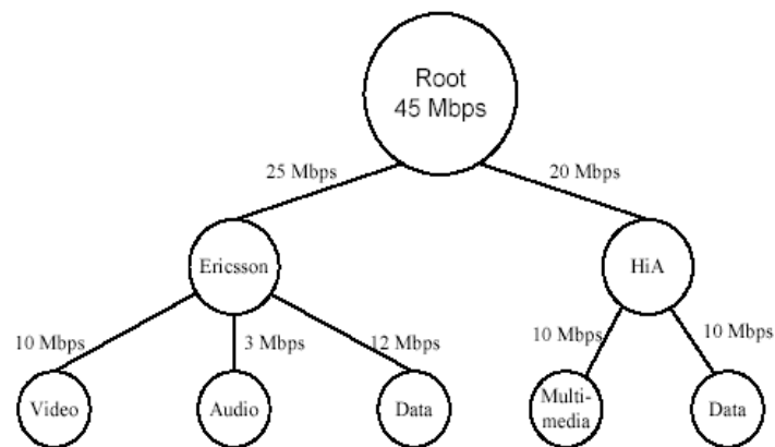
Figure 3.9 An example of a link-sharing hierarchy.
