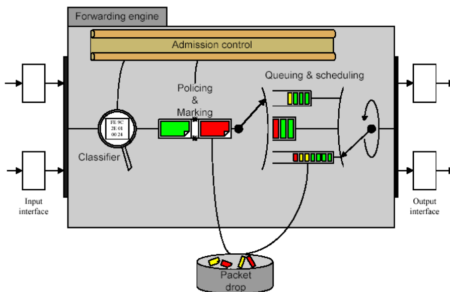
Figure 3.1 Packet handling in a router that supports QoS
