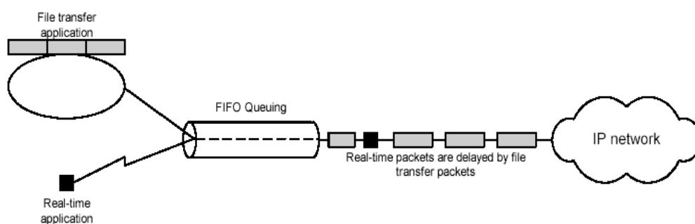
Figure 3.4 Potential impact of a file transfer on Interactive Traffic with FIFO queuing.
