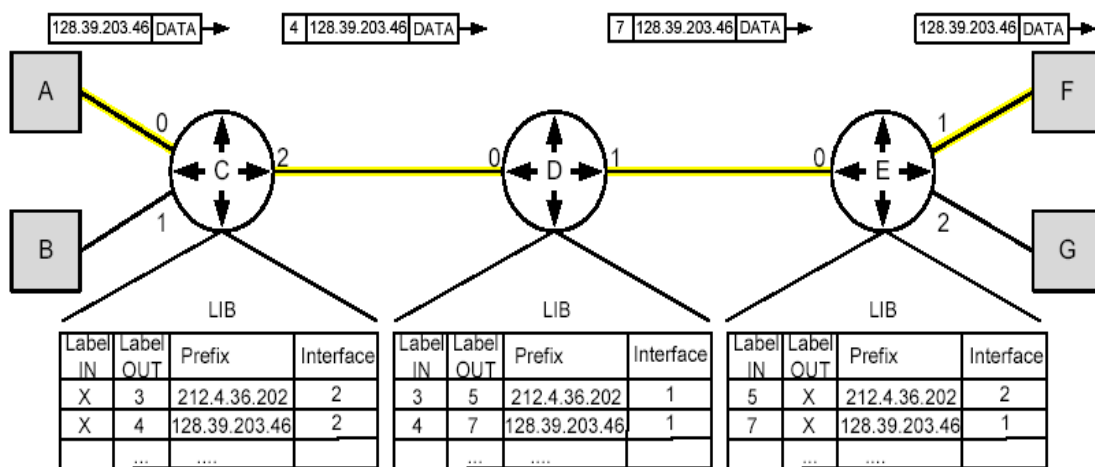
Figure 4.4 Label swapping and forwarding in MPLS
