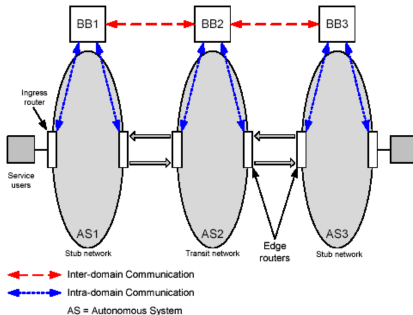
Figure 4.6 Bandwidth Broker communication
