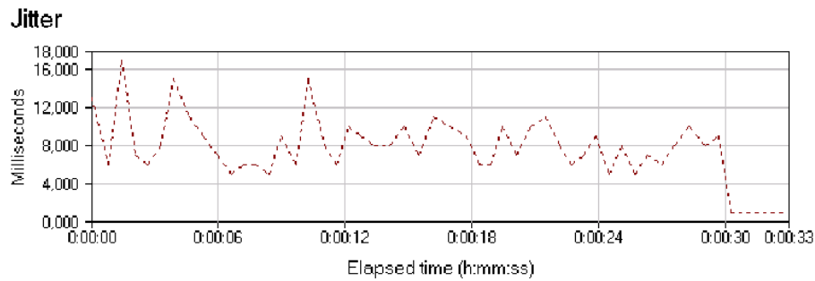
Figure 5.1 Measured Best Effort jitter performance(mean 8.208ms)
