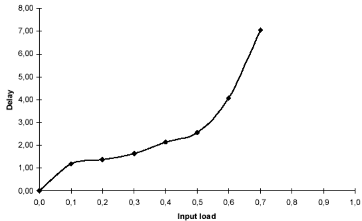
Figure 5.7 Measured Delay for Best Effort
