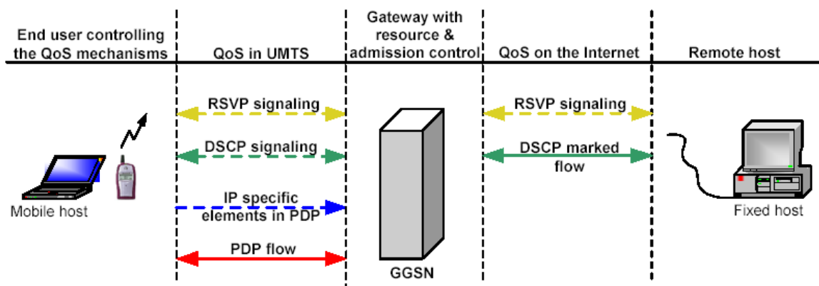
Figure 6.3 QoS model of a mobile network
