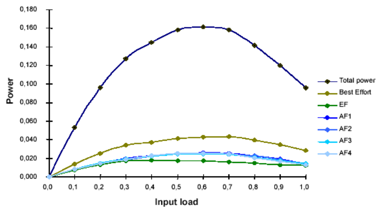
Figure 5.12 Computed Power for Diffserv
