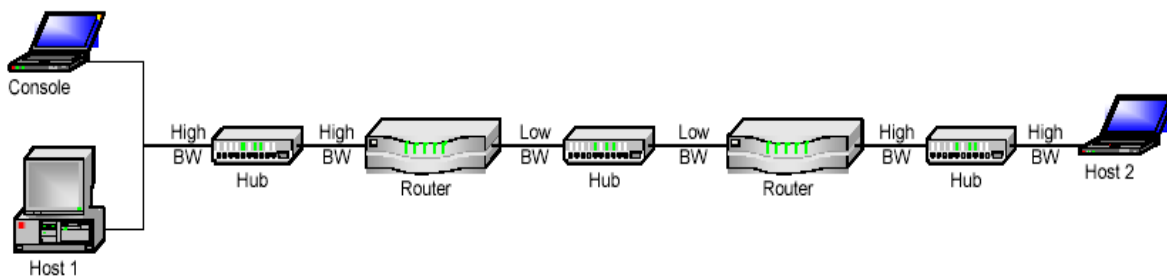
Figure 5.2 The testbed Scenario
