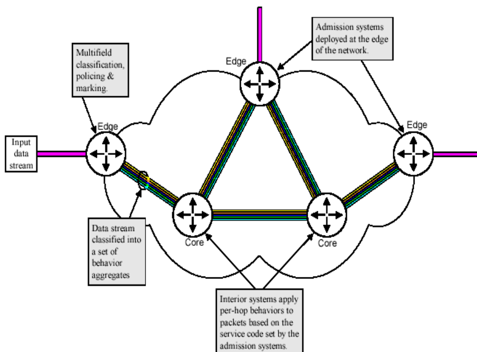
Figure 3.15 The Differentiated Services Architecture.
