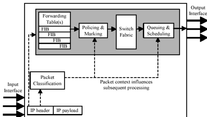
Figure 3.2 An overview to how classification influences forwarding .
