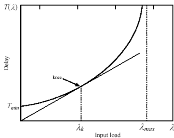
Figure 5.5 The Delay Characteristic of a system.
