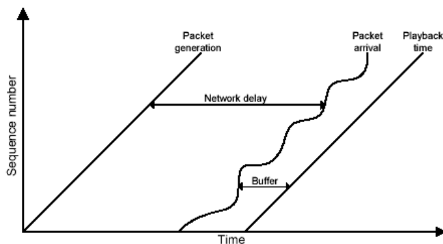
Figure 2.3 The role of a playback buffer
