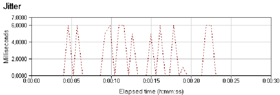
Figure 5.3 Measured DiffServ EF jitter performance (mean 1.321ms).
