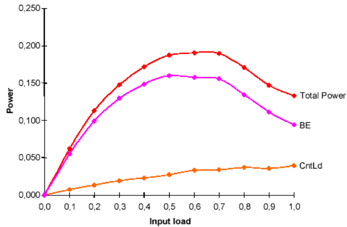
Figure 5.8 Computed power for Intserv.
