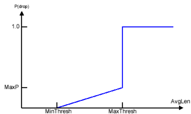
Figure 3.10 Drop Probability function for RED
