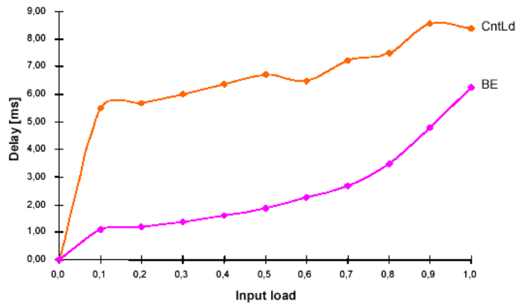
Figure 5.9 Measured Delay for Intserv
