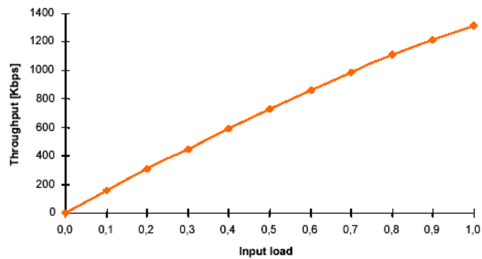
Figure 5.10 Measured throughput for controlled load
