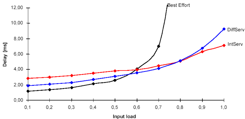
Figure 5.15 The Delay Graphs compared
