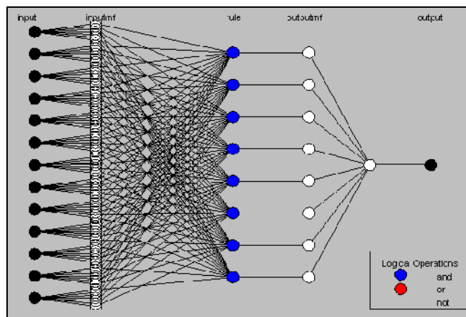
Figure 3.5: ANFIS model structure of Gliflix dataset.
