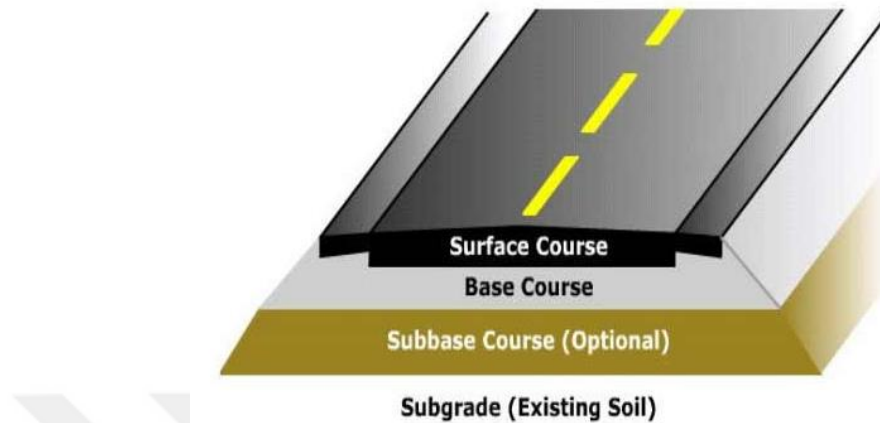
Figure 3.3. Flexible Pavement Cross Section [49].
