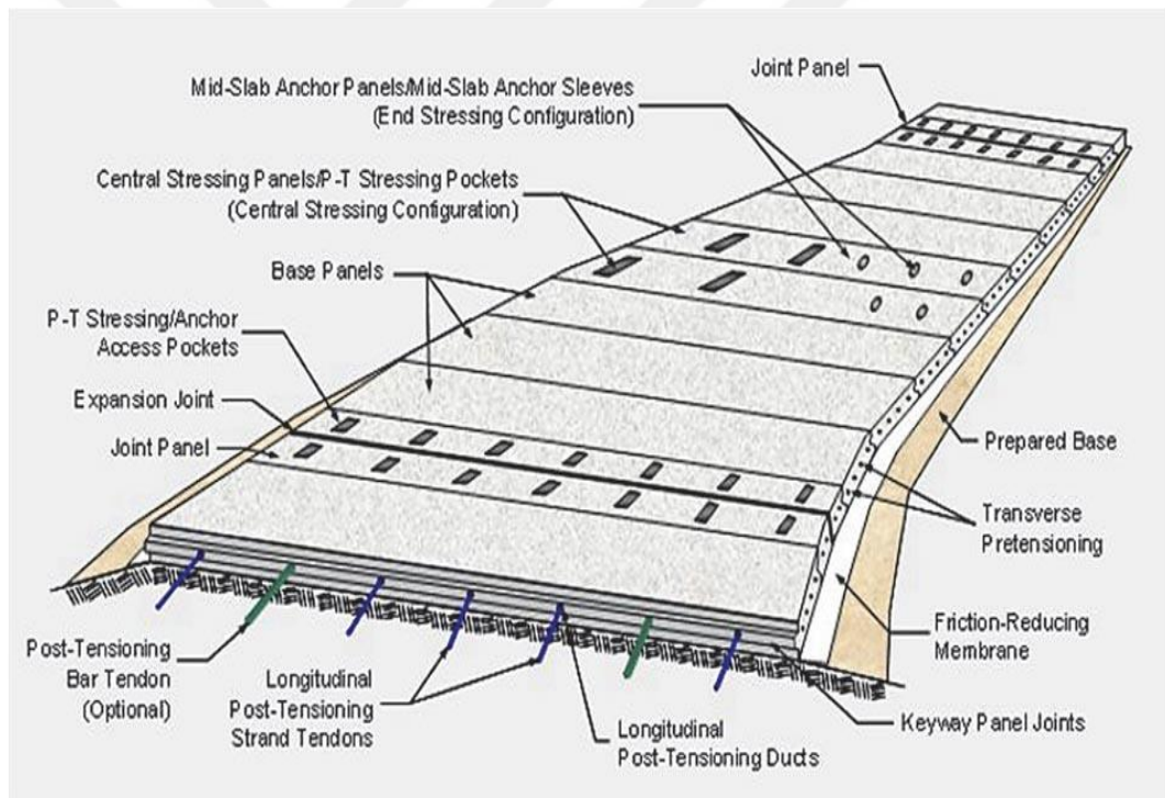
Figure 5.18. Construction joint [63].
