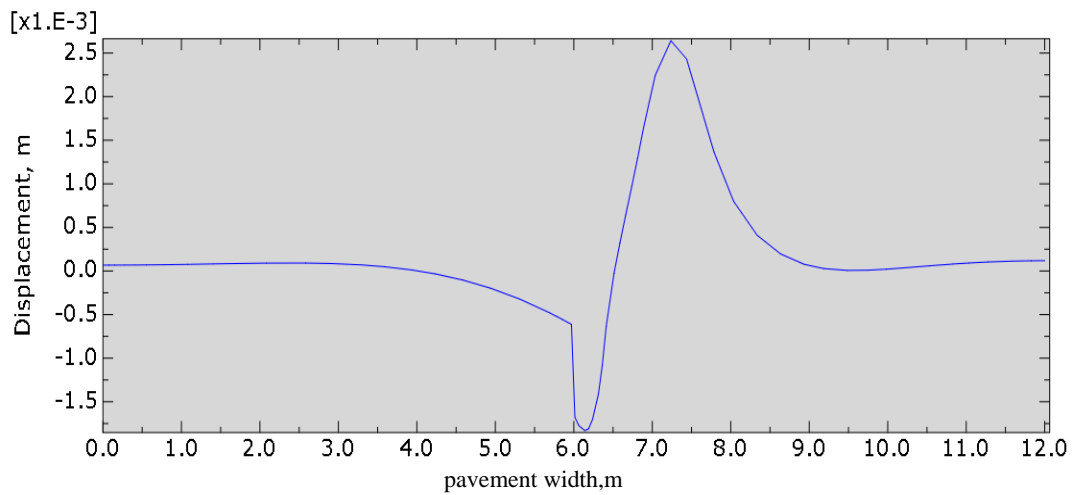
Figure 5.51. Vertical displacement along the pavement surface.
