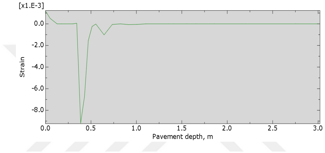
Figure 5.50. Vertical plastic strain vs pavement depth.
