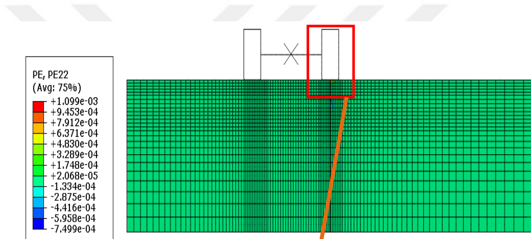
Figure 5.34. The vertical plastic strain distribution on the joint.
