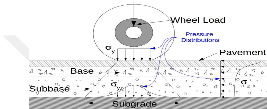
Figure 5. 20. Pavement design due to rutting criterion [71].
