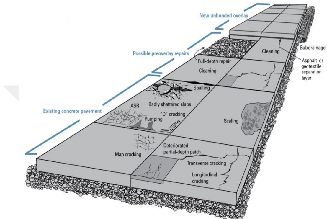
Figure 5.11. Shows us of rigid paving deformations [65].
