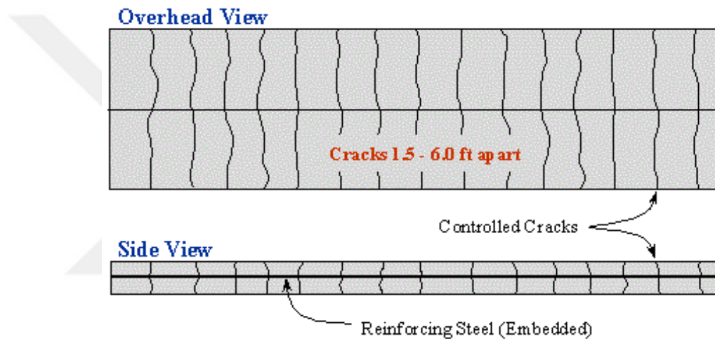
Figure 3.17. Cross section of CRCP [58].
