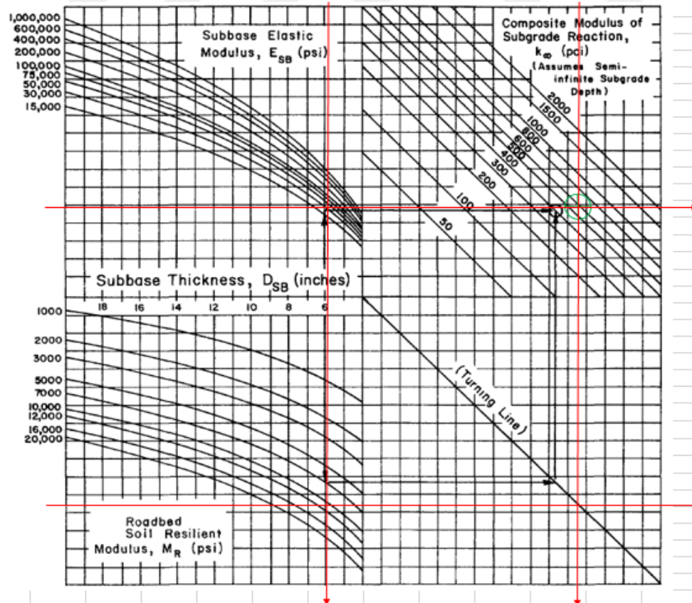
Figure 4.2. Data used in the design [30].
