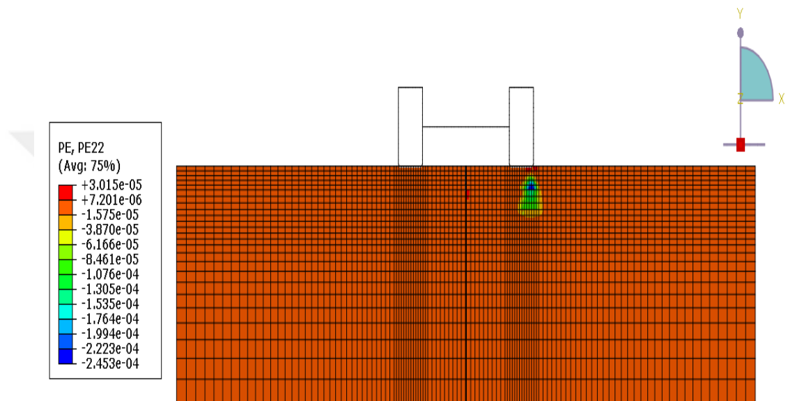
Figure 5.28. Plastic strain in the direction of “y”.
