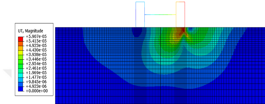
Figure 5.25. Model of displacement with repeated loads.
