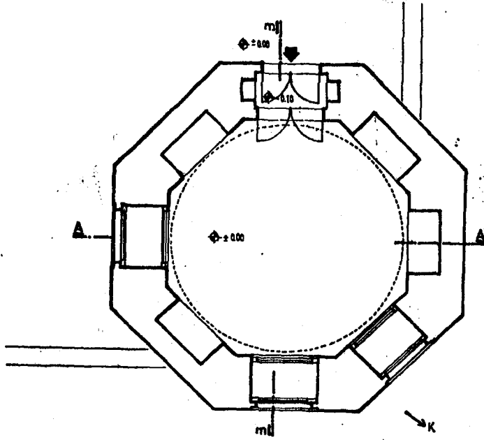
ÇİZİM. 58 AFYON YENİ CAMİİ MUVAKKİTHANESİ PLANI
