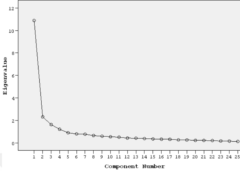
Scree Plot
