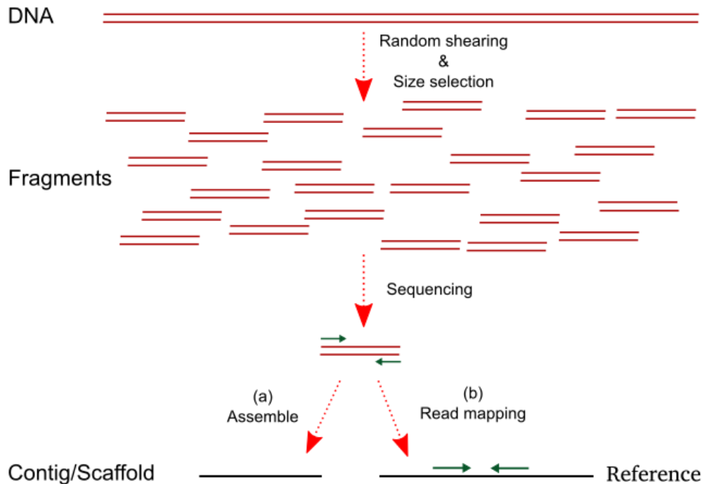
Figure 1.4: Whole Genome Shotgun (WGS) sequencing. Firstly, DNA is fragmented randomly and then each fragment is sequenced from both left and right ends using a sequencer. These are called paired-end reads. The number of base-pairs that the sequencer reads called read length depends on the sequencing machine used. Finally, the reads; (a) can be assembled into contigs when a reference genome is not available or (2) can be mapped to a reference genome
