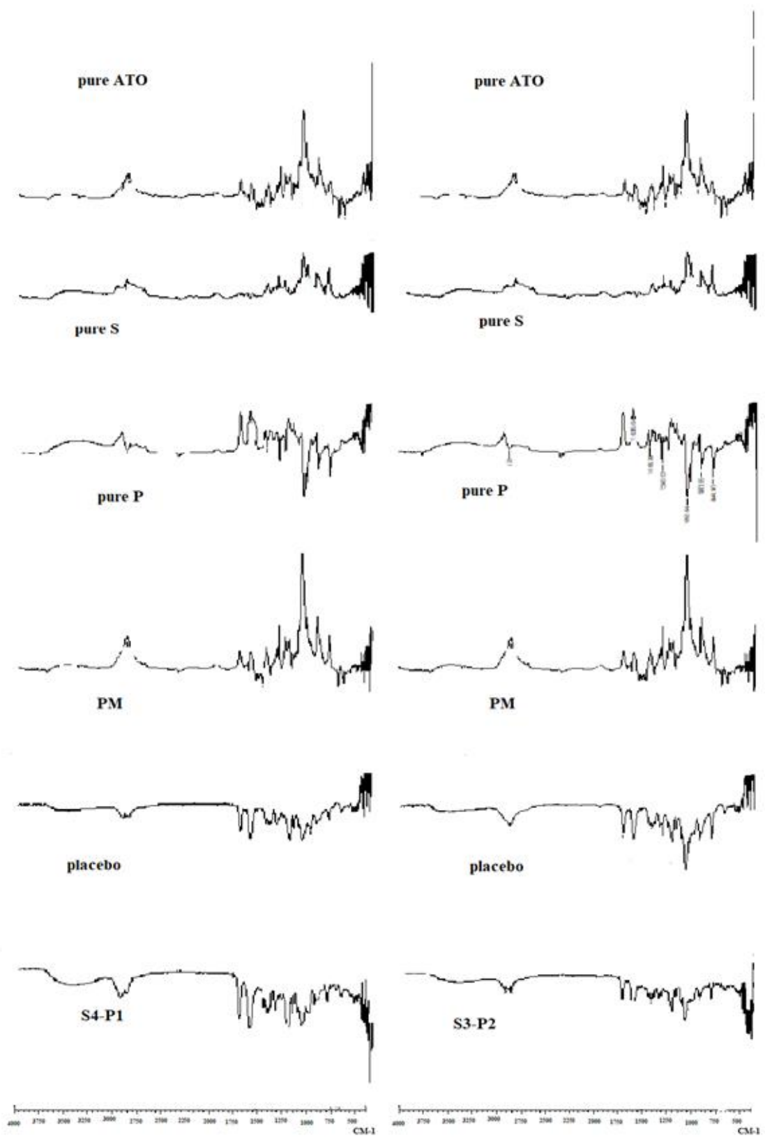
Figure 4.21. FT-IR spectrums of ATO, polymers, PMs, placebo and PMs for S4-P1 and S3-P2.
