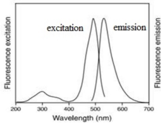
Figure 1.11: Excitation and emission spectra of SYBR Gold nucleic acid gel stain bound to double-stranded DNA [18].
