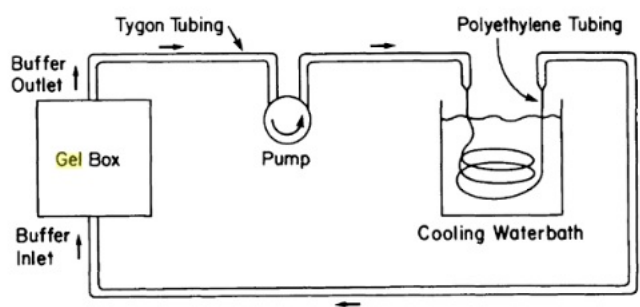
Figure 1.6: Components of a PFGE system [11]
