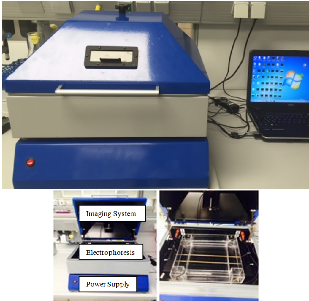
Figure 2.3: Observable Real-Time PFGE. Imaging System, electrophoresis and power supply combined in one device.
