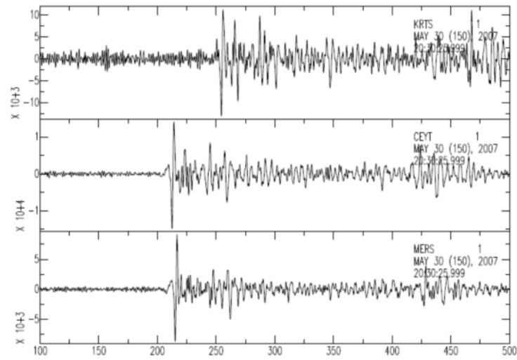
Figure 3.6. A teleseismic earthquake recorded at KRTS (top), CEYT (middle), MERS (bottom) stations. A time shift of 40 sec is apparent between KRST and other stations.
