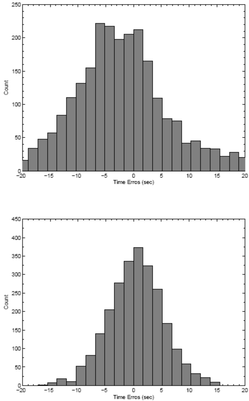
Figure 4.7. Histograms of travel time misfits for initial model (top) and final model (bottom) at 20 sec period.
