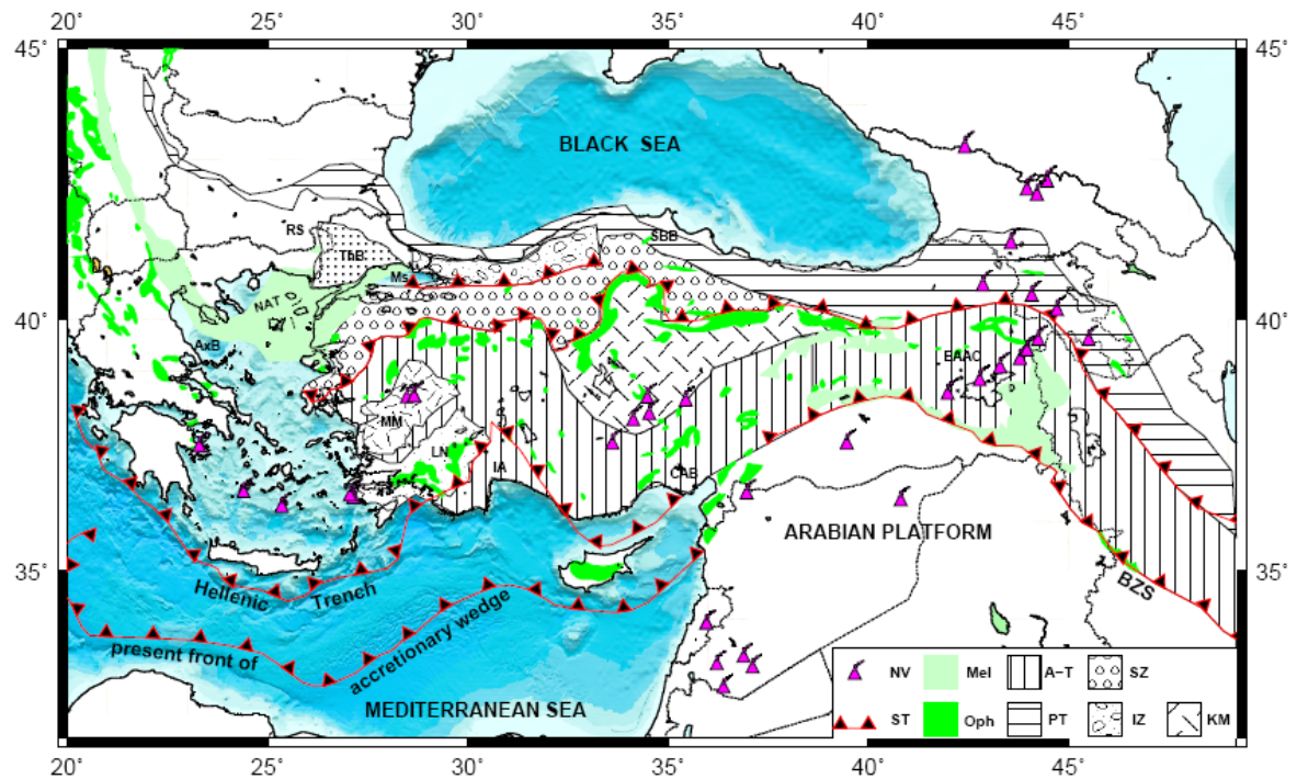
Figure 1.1. Tectonic setting of Turkey; AxB, Axios Basin; A-T, Anatolid-Tauride Block; CAB, Clicia-Adana Basin; EAAC, East Anatolian Accretionary Complex; IA, Isparta Angle; IZ, Istanbul Zone; KM, Kırşehir Massif; LN, Lycian Nappes; MM, Menderes Massif; NAT, North Aegean Trough; PT, Pontides; RS, Rhodope-Strandja Basin; SBB, Sinop-Boyabat Basin; SZ, Sakarya Zone; ThB, Thrace Basin. Green and light green units represent the ophiolites and ophiolitic mélanges, respectively. Bathymetry of the region derived from ETOPO5. Purple volcano signs show neogene and quaternary volcanism. Red triangles show the sutures and earlier subduction zones. (Modified from Stampfli, http://www-sst.unil.ch/research/plate_tecto/present_day.htm ; Okay and Tüysüz 1999;
