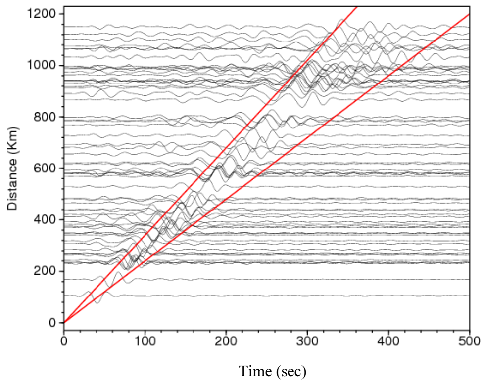
Figure 3.10. Top: The event gather of the earthquake band-pass filtered between 30-60 sec periods. Bottom: The estimated Green's functions from the long term correlations of PTK station with the other broadband stations. Red curves indicate the times corresponding to velocity of 2.4 km/s and 3.4 km/s.
