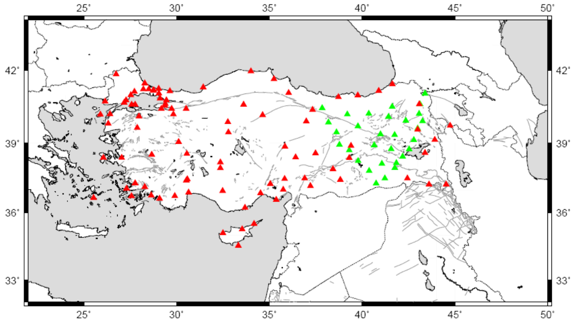
Figure 2.1. Permanent and temporary seismic stations used in the noise analysis. Red triangles are the broadband stations from different networks recording during 2005-2007. Green triangles are ETSE stations operated during 1999-2001.
