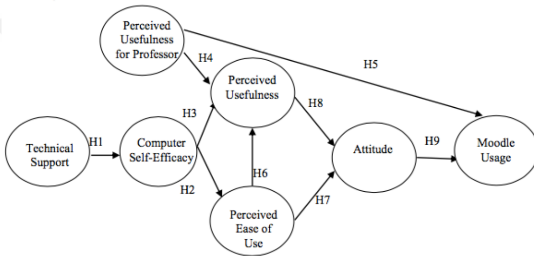
Figure 13. Kilic (2014) e-TAM
