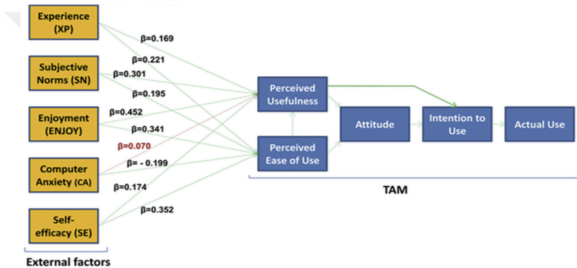
Figure 12. Abdullah and Ward (2016) e-TAM
