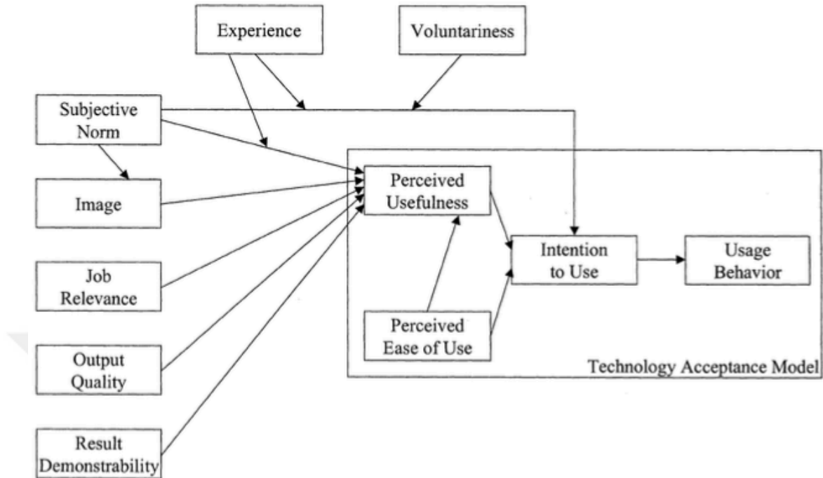
Figure 14. Acarli and Saglam (2015) TAM2
