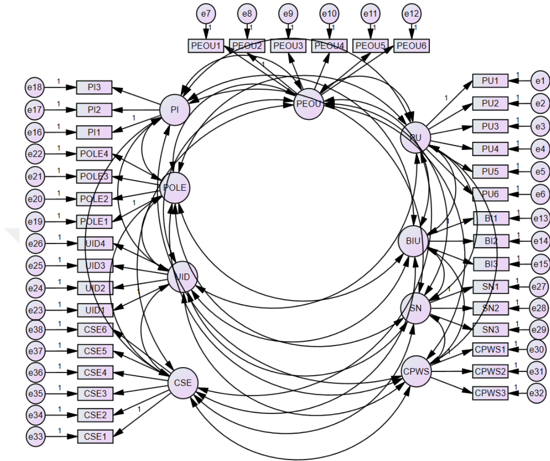
Figure 22. Amos covariance diagram for measurement model
