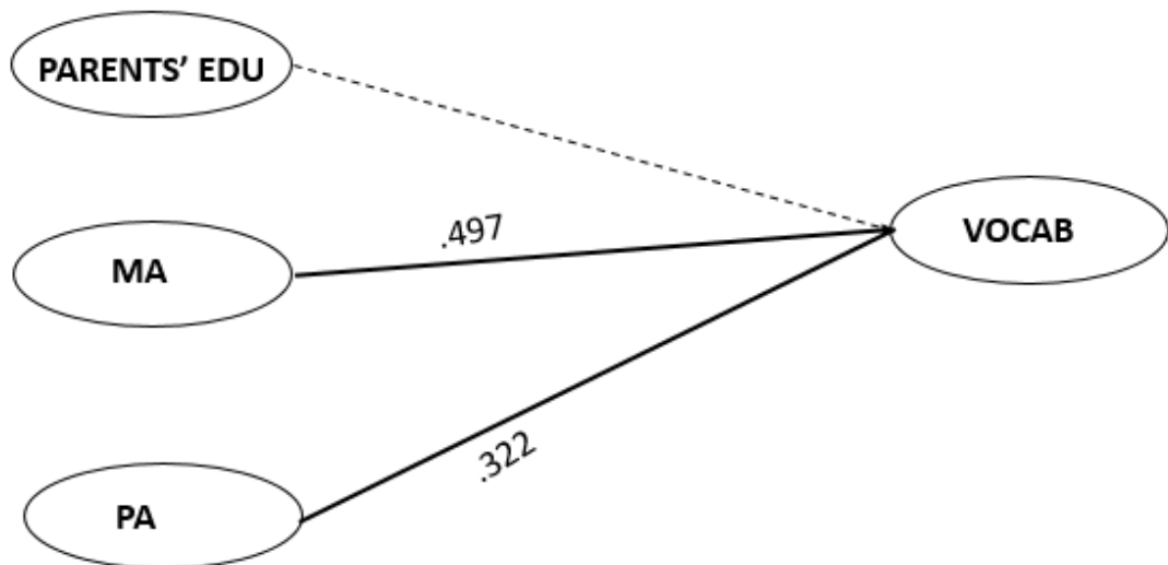
Figure 5. Direct effects of parents' education level, MA and PA on vocabulary for Grade 2
