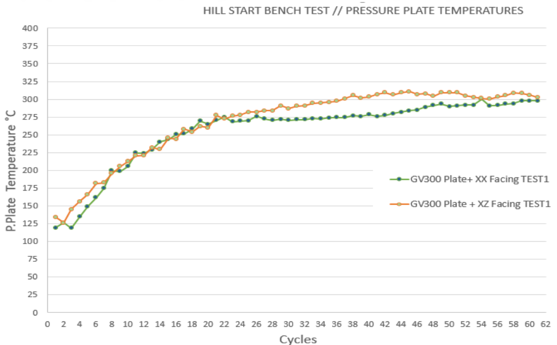
Figure 3.33. Hill Start Bench Test P. Plate Temperature Measurement
