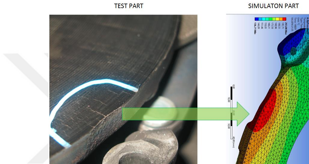
Figure 3.15. Comparison output of FEA and experimental study
