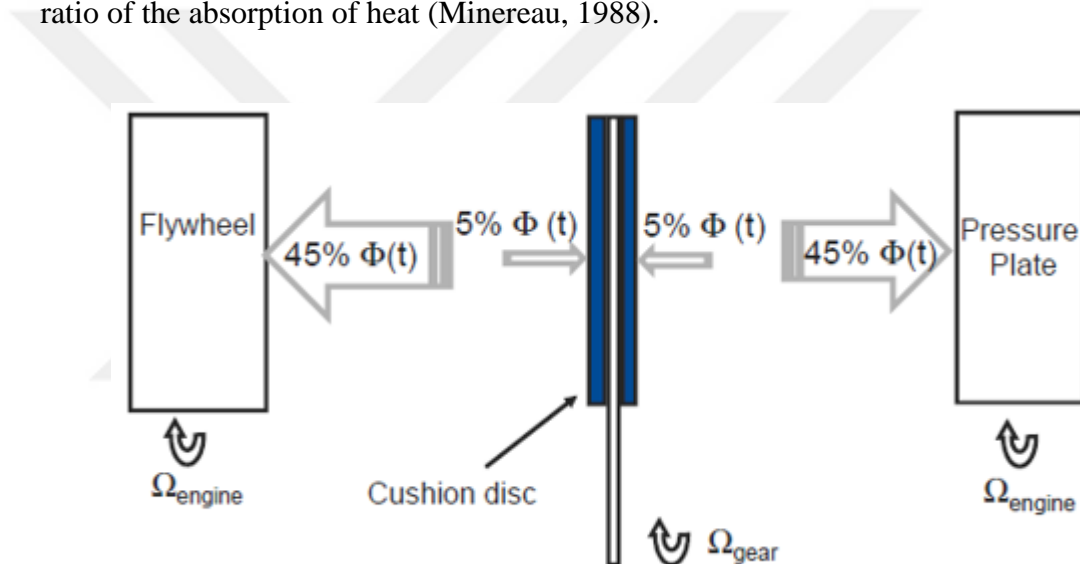
Figure 2.1. Usual assumption for heat distribution
