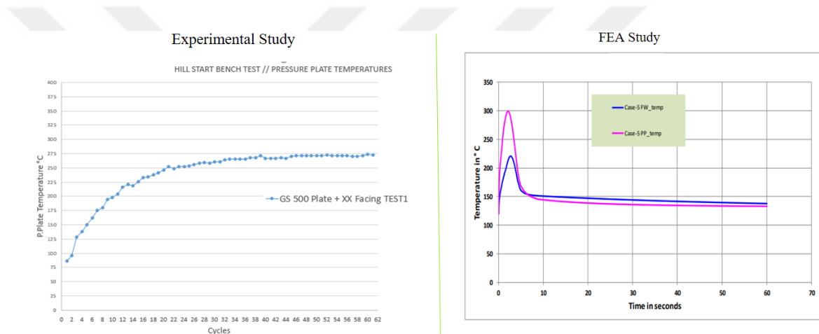
Figure 3.27. Hill Start Test FEA outputs as Temperature vs Time
