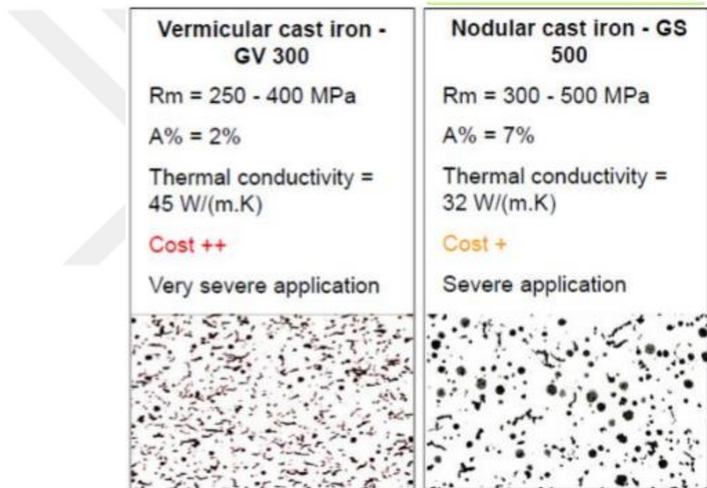
Figure 3.28. Comparison of GV 300 and GS 500 (Valeo Cast Iron Guide)
