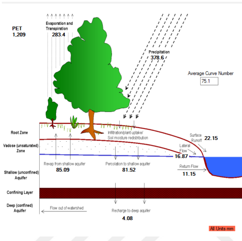
Figure A.2: Hydrological cycle for Lake Mogan in SWAT
