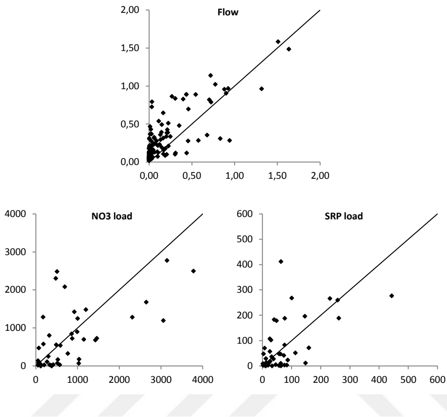
Figure 4.3: Scatterplots of the relationship between observed (X-axis) and simulated (Y-axis) flow rate, NO 3 loading and SRP loading with the line representing a 1:1 relationship shown.
