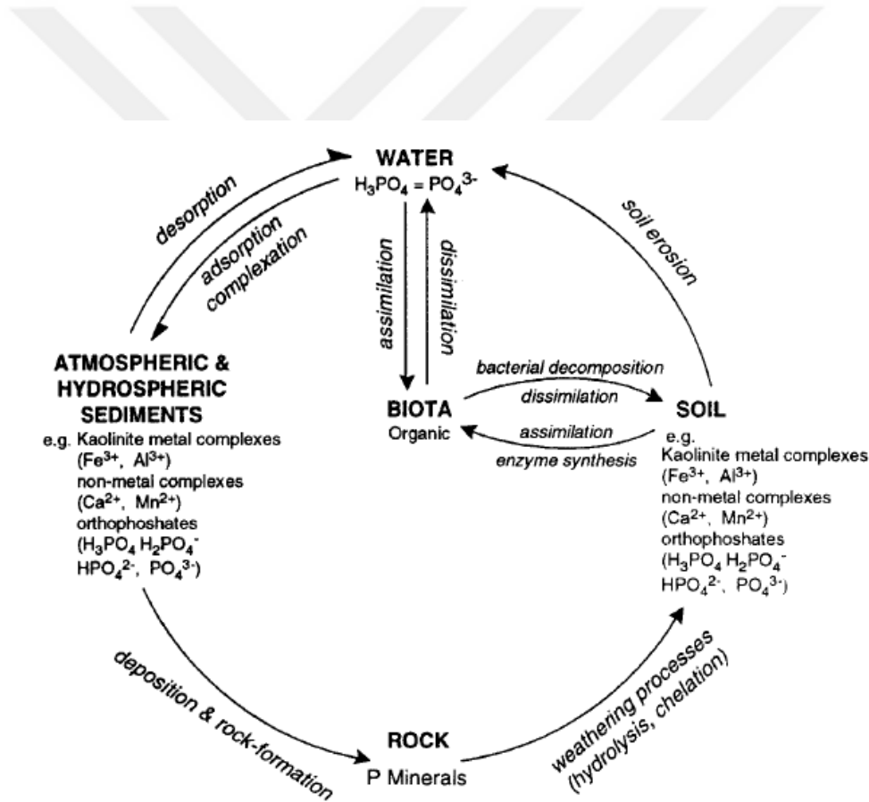
Figure 1.1: Phosphorus cycle (taken from Heathwaite et al., 1996).
