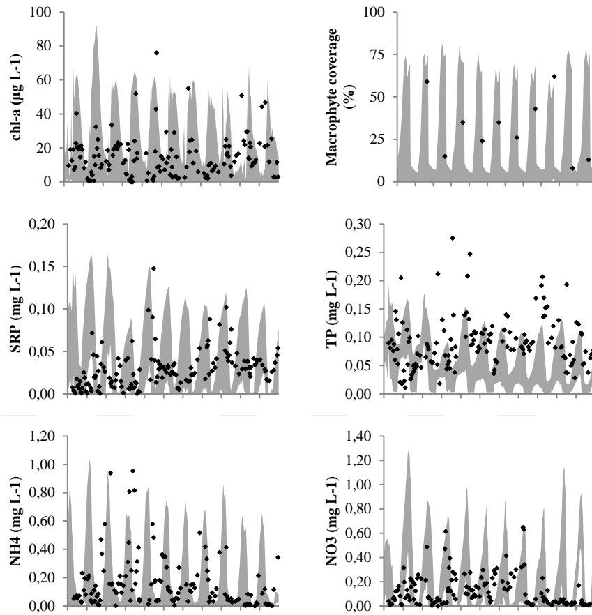
Figure 4.4: Performance of the PCLake model for Lake Mogán against observed values. Grey bands represent the range between the 2.5 th percentile and the 97.5 th percentile on a daily basis based on 250 iterations of the model with parameter values inside the calibration ranges.
