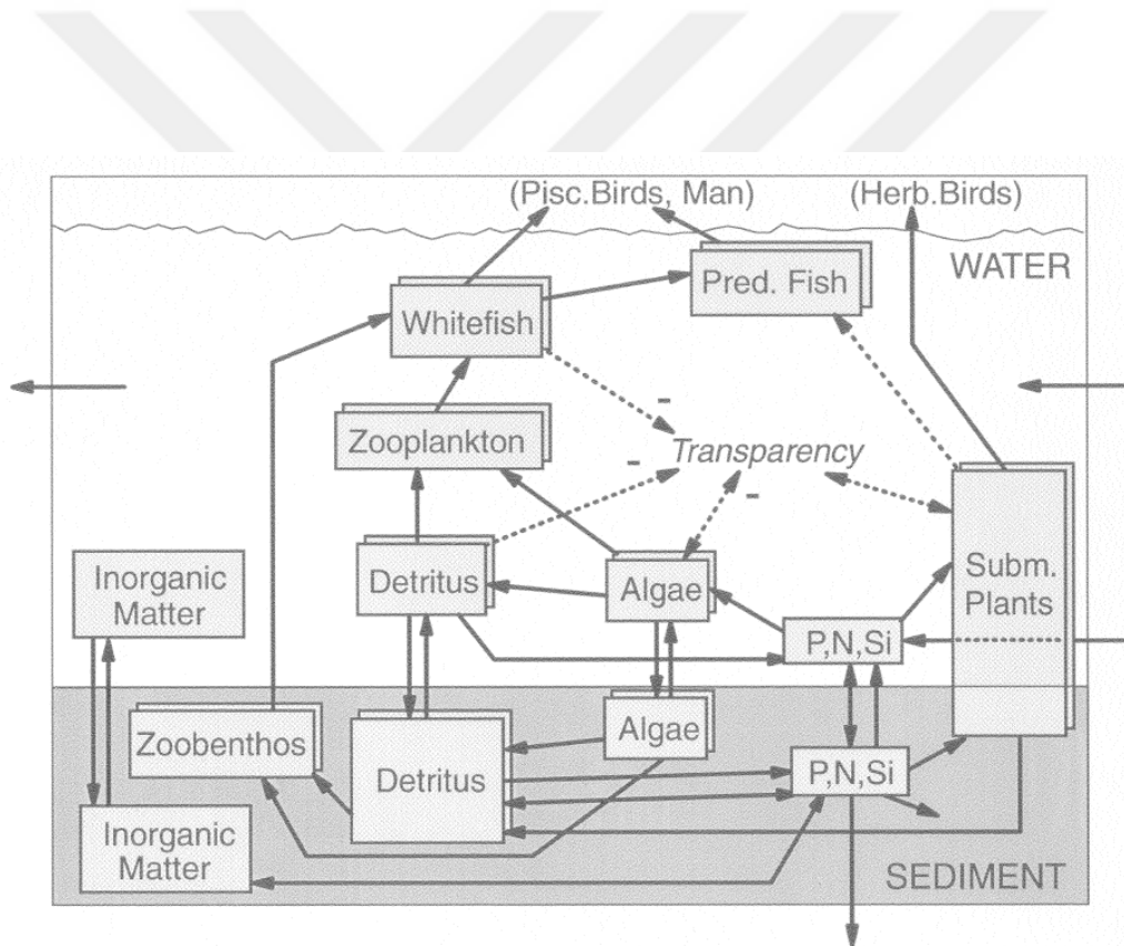
Figure 1.5: PCLake model structure (Janse, 1997): Arrows with solid lines represent mass fluxes; arrows with dotted lines represent empirical relations
