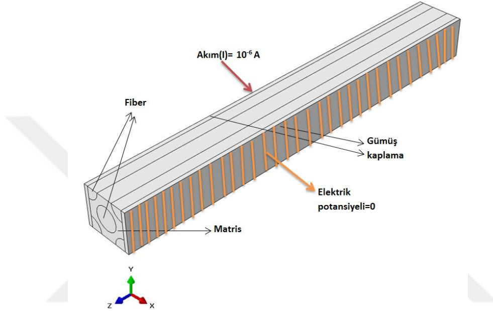
Şekil 5.23 3D Hexagonal model.
