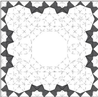
Geometry of first layer
