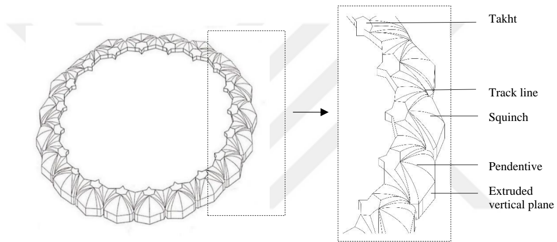
Figure 50. Track elements of Muqarnas
