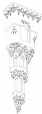
Figure 164. The design for the projecting muqarnas by windows (Web 58)
