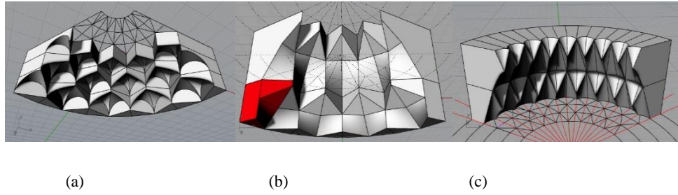
Figure 71. Muqarnas modeling in Design Computing courses (Web 40) Modeled by Seda Öznal (a), modeled by Elif Özüçağlıyan (b), modeled by Ekin Arslan (c)
