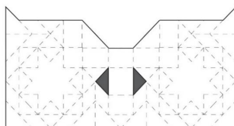
Geometry of third layer
