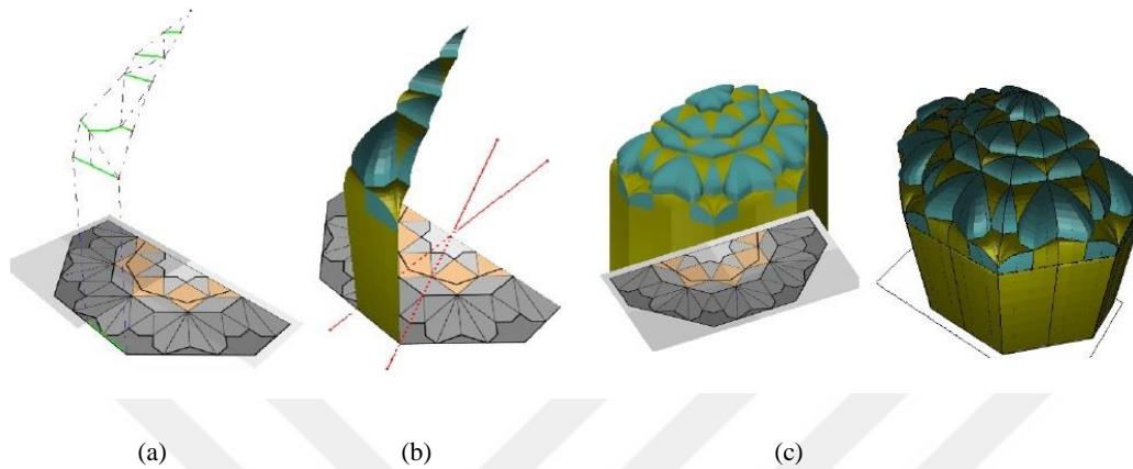
Figure 72. The process of constructing a Muqarnas vault
