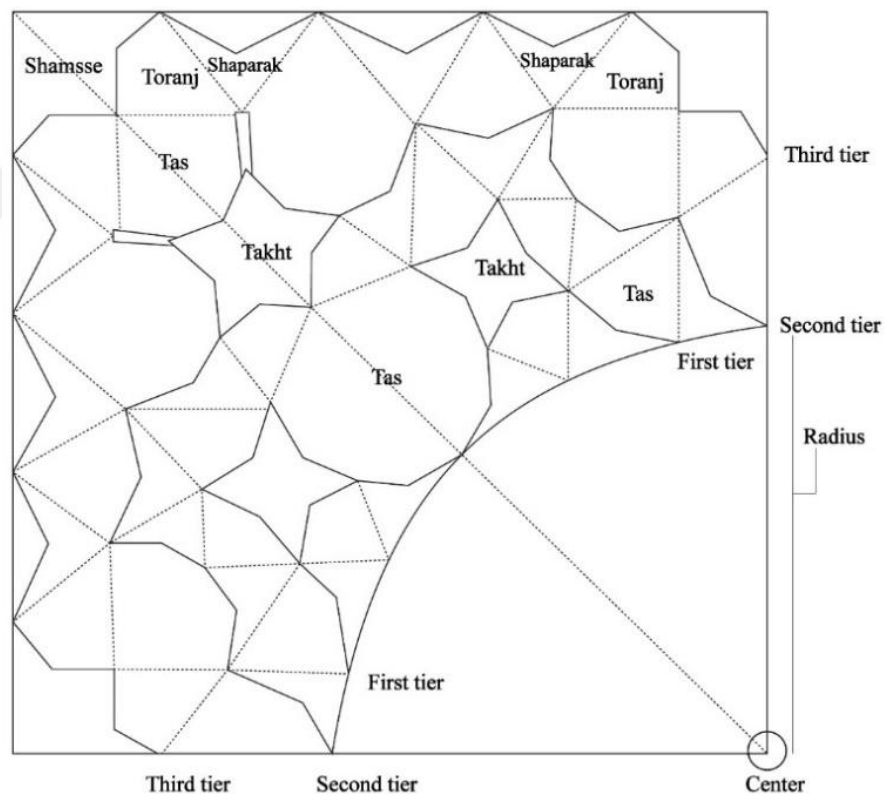
Figure 44. Two-dimensional plane projection of a Muqarnas composition (Web 36)
