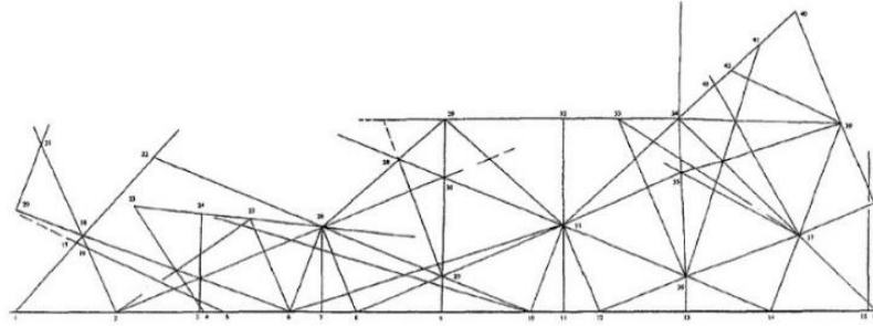
Figure 60. Construction of the Central Muqarnas vault
