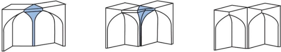
Figure 43. Three ways of joining intermediate element/elements and cells
