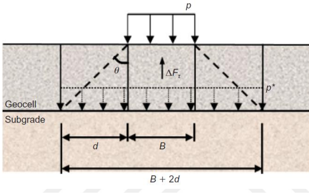
Figure 2.12 Illustration of the stress dispersion effect adopted for the presented method (Neto et al., 2013)
