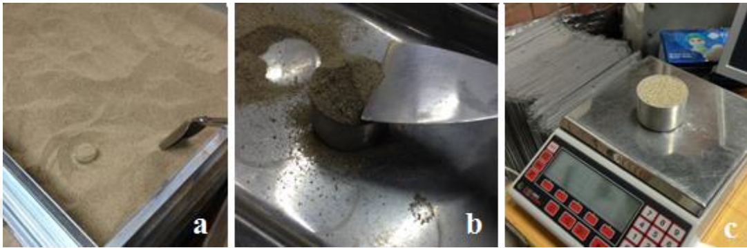
Figure 4.3 Steps of relative density tests
