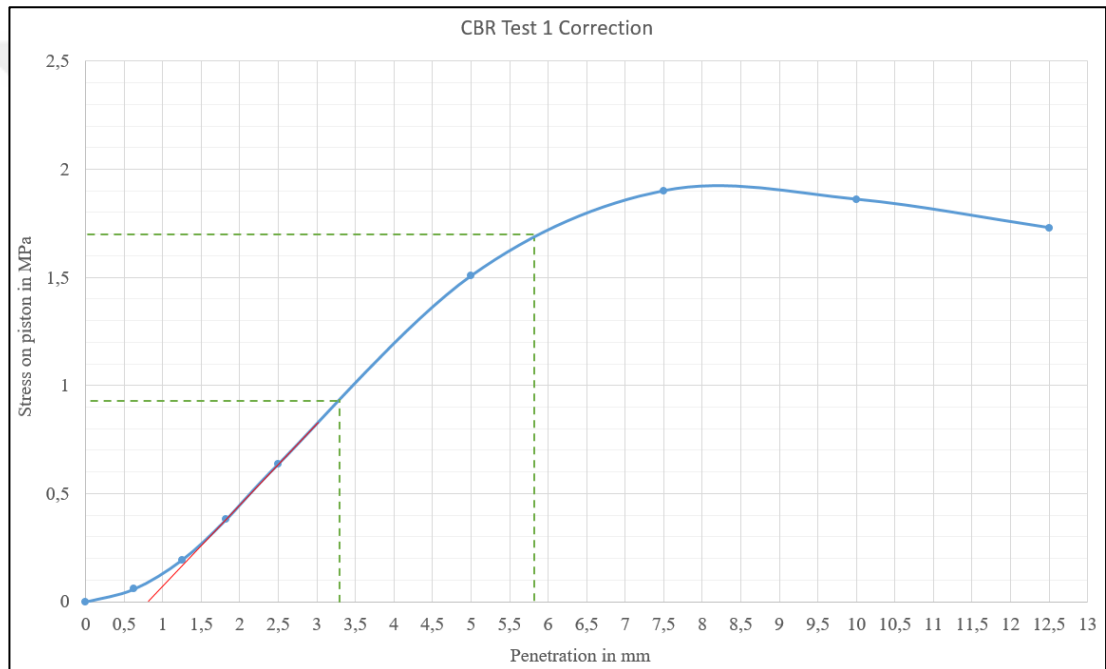
Figure B.1 Correction of CBR Test 1
