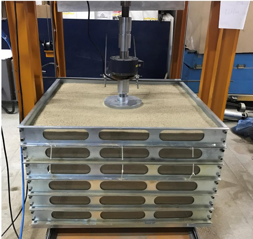
Figure 4.13 Filling of the tank to desired height, placement of loading plate and load cell
