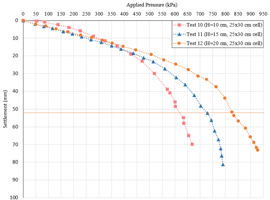
Figure 4.20 Results of test series 3
