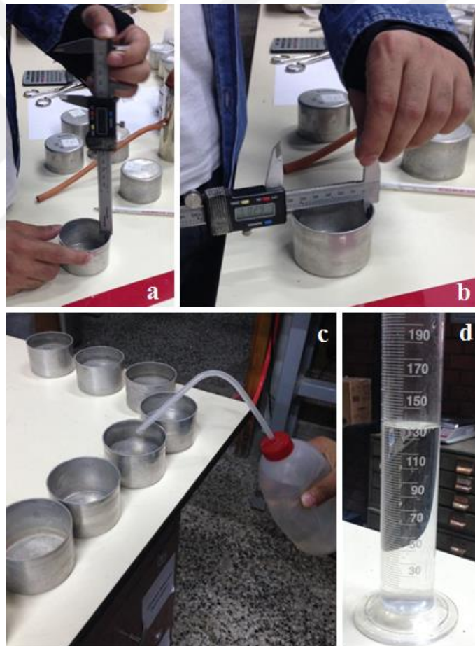
Figure 4.2 Volume determination of relative density boxes
