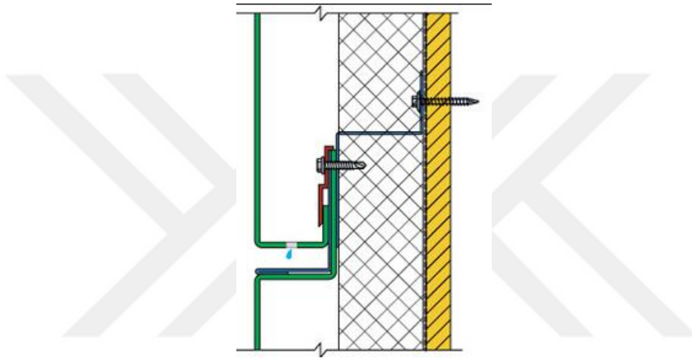
Figure C.38. Condensation guttering details for overlap panel joints (Ceruti, 2012).
