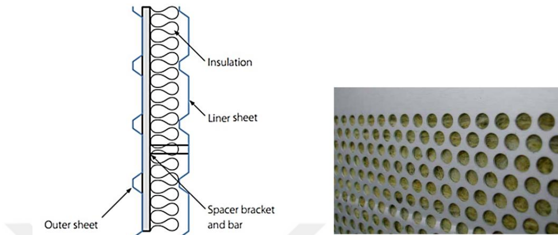
Figure C.64. Left: cross section of the position of non-reflective liner sheet layer. Right: example of a perforated liner sheets (Tata Steel, 2012).
