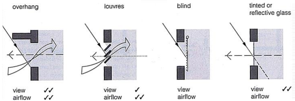
Figure C.50. Light-directing louvers; Okasolar system (IEA, 2000a).
