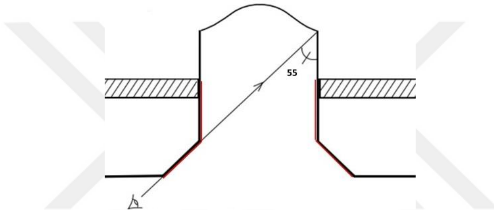
Figure C.59. Optimum cut-off angle of skylights for office buildings along with combination of straight and splayed walls in ceiling part (Skylighting Design Guidelines, 2014).
