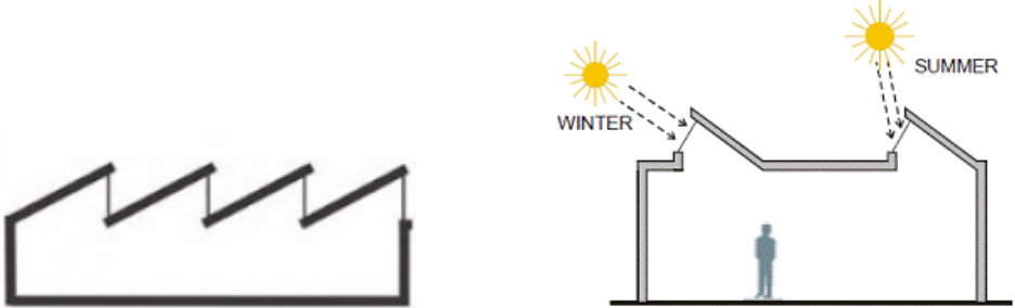
Figure C.41. Saw tooth clerestories with sun-catcher baffles ( elad.su-per-b.org ).
