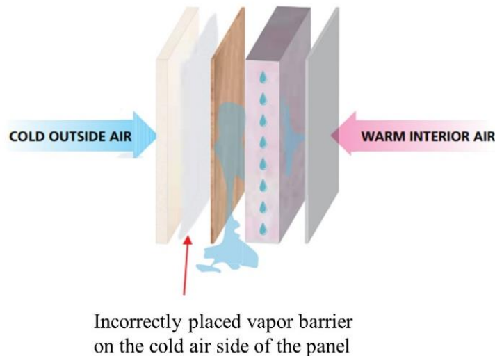
Figure C.29. Position of vapor barriers (WaterTech, 2011).
