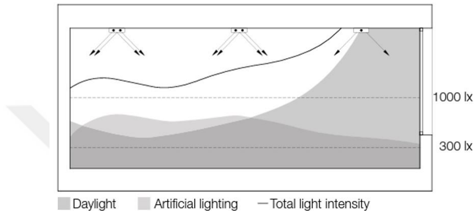
Figure B.4. Cross-section of a combined lighting scenario (Schittich, 2011, p.50).
