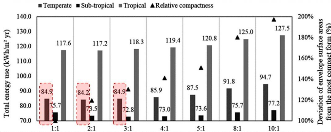
Figure 4.4. Total energy consumption for seven plan aspect ratios (Raji, et al., 2017).
