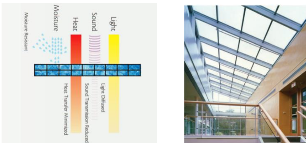
Figure C.45. Translucent aerogel skylights schematically (Wasco Products, waskoskylights.com).
