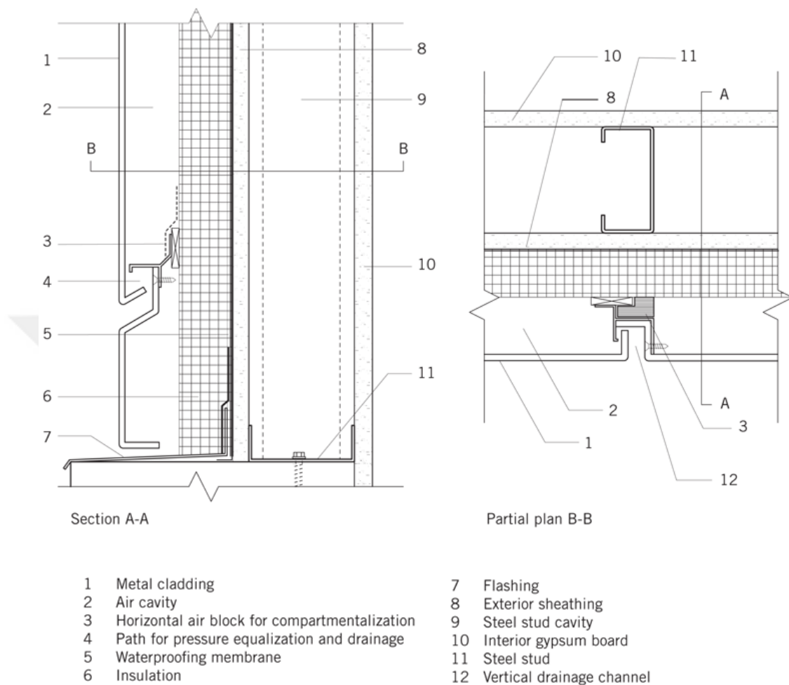
Figure C.27. Schematic concept of pressure-equalized rain screen (Aksamija, 2013, p.25).
