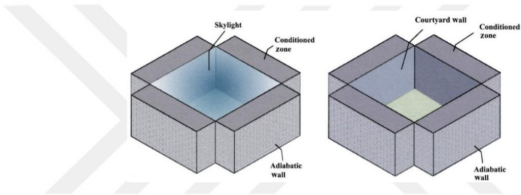
Figure 4.8. The models of atrium and courtyard (Aldawoud and Clark, 2008).
