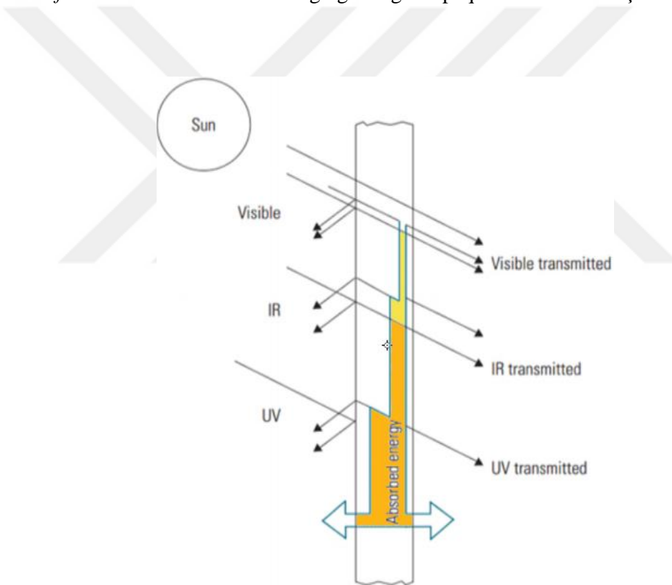
Figure 4.22. Light and heat transmission through glass (by the author).
