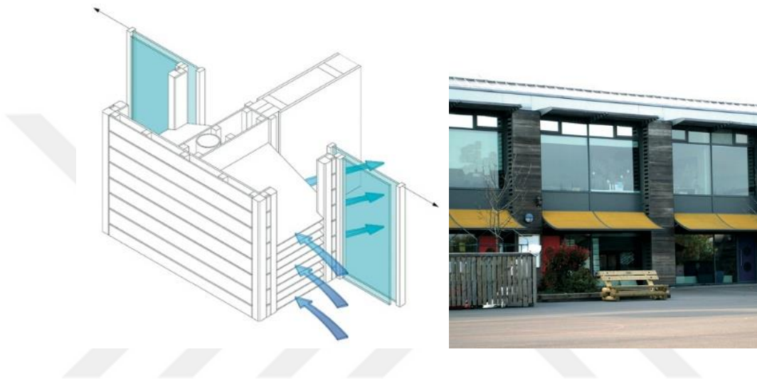
Figure A.5. External Vent Box and the incorporated façade (machacoustics.com).
