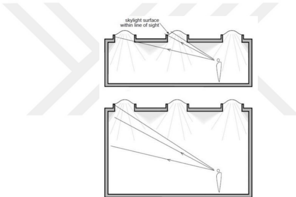
Figure C.58. Visual discomfort in high and low ceilings (SkylightingDesignGuidelines, 2014).
