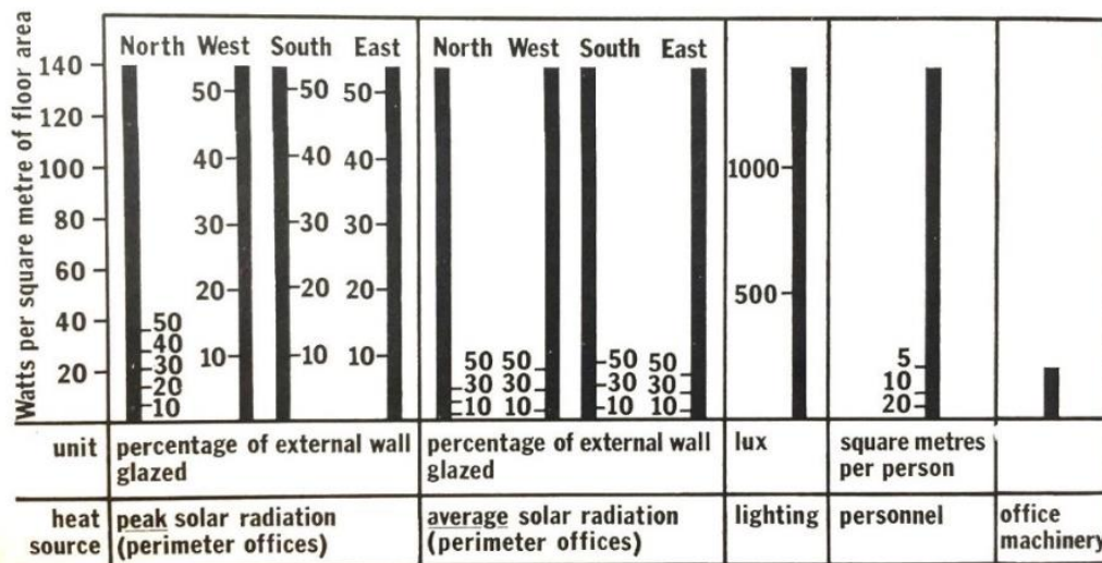
Figure A.4. Heat gains in peripheral offices with peak and average solar radiation and glazing percentage (Duffy et.al, 1976, p.144).
