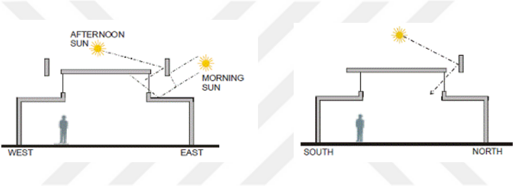
Figure C.40. Left: east-west vertical clerestories with sun-catcher baffles. Right: north-south vertical clerestories with sun-catcher baffles ( elad.su-per-b.org ).
