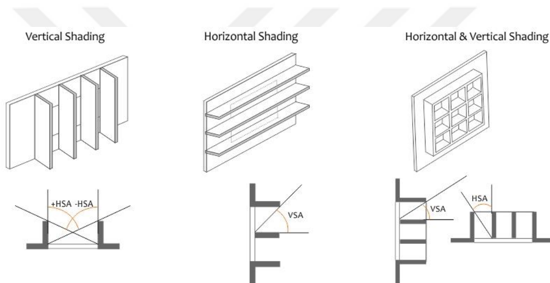
Figure C.21. Three main shading strategies ( http://www.nzeb.in ).
