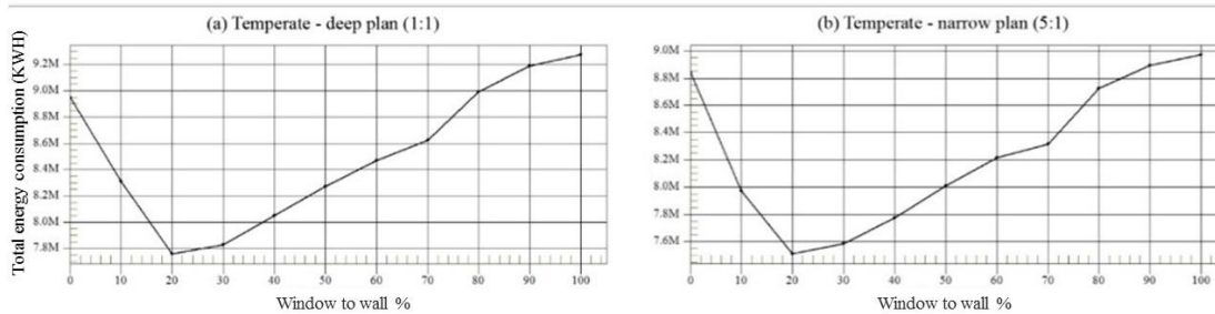
Figure 4.6. The optimal percentage of window-to-wall ratio for two plan types (1:1 and 5:1) in temperate climate (Raji, Tenpierik, and van den Dobbelen, 2017).
