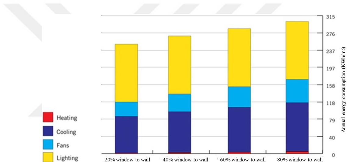
Figure 4.5. Effects of window-to-wall ratio for mixed, dry 4B climatic zones (Aksamija, 2013, p.22).
