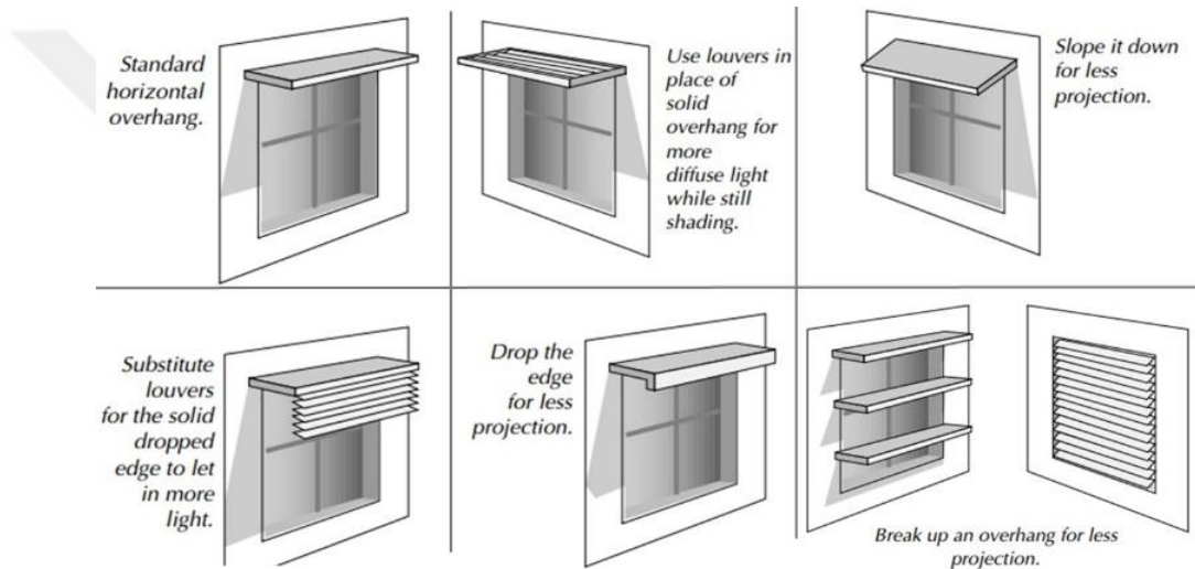
Figure C.19. Positions for horizontal shadings on south façades (US. Department of Energy).
