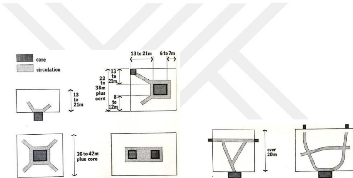
Figure 3.8. Left: deep space, right: very deep space (Duffy et al., 1976, pp.43-44).
