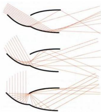
Figure C.47. Anidolic ceiling examples (Baker and Steemers, 2002).
