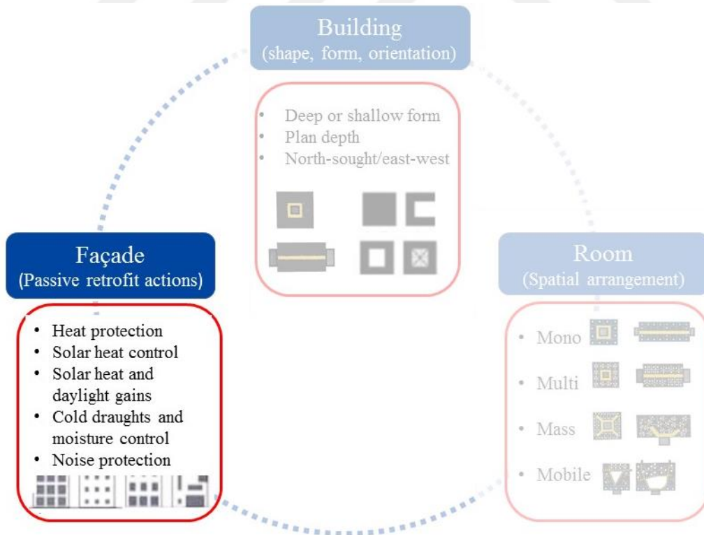
Figure 4.21. Passive retrofitting criteria applicable on existing façade system (author).
