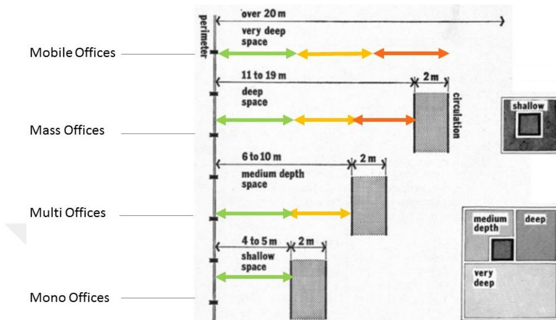
Figure 4.20. Passive zones in deep (above) and very deep spaces (below).
