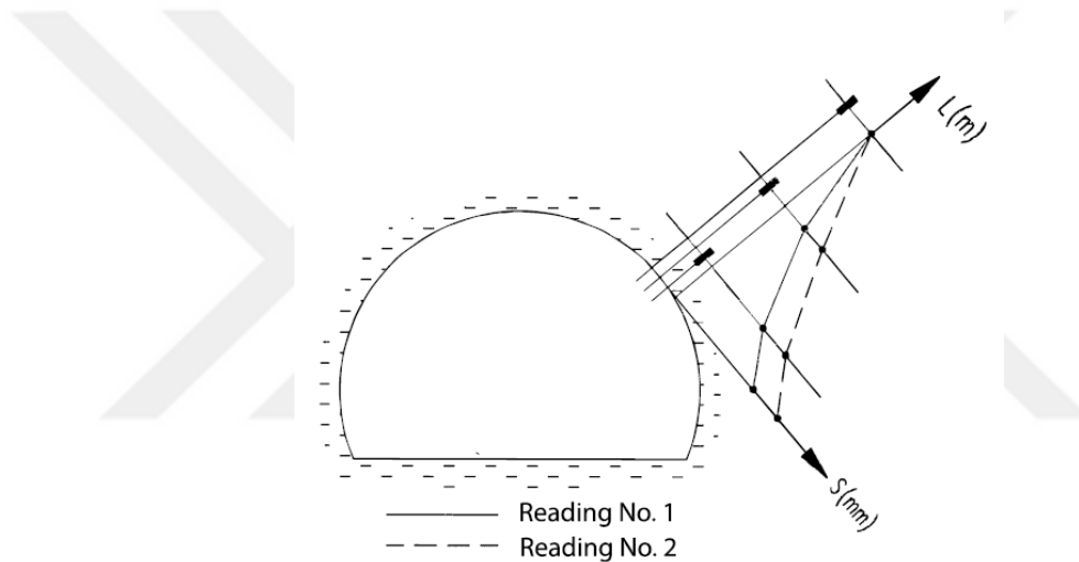
Figure 5 Extensometer Reading (Lunardi, 2008)
