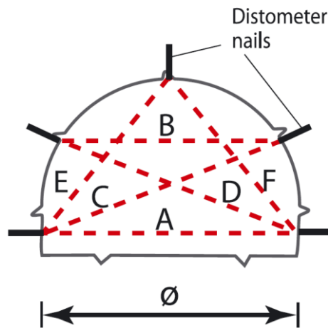
Figure 3 Convergence Measurement with Distometer (Lunardi, 2008)
