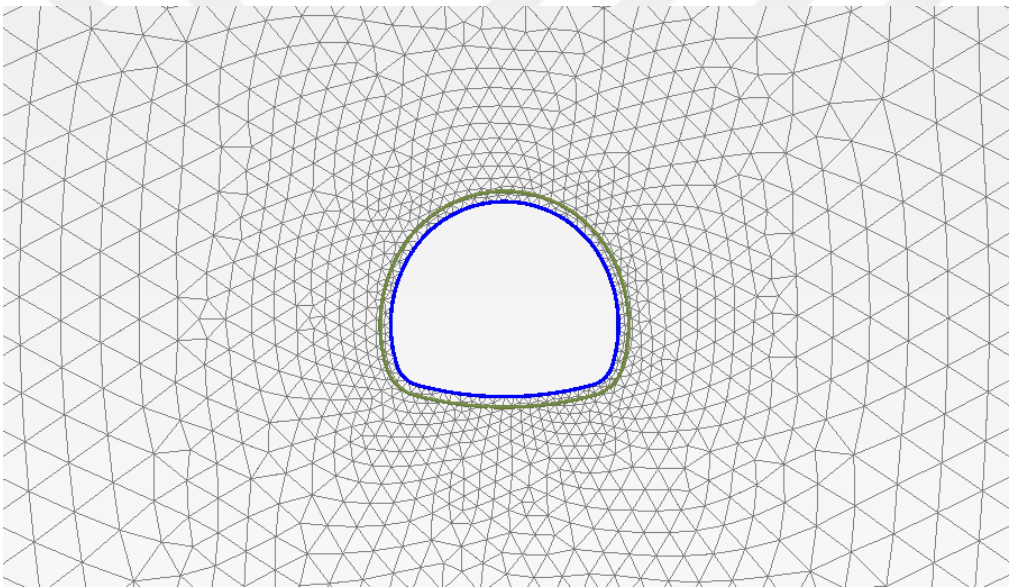
Figure 8 Tunnel Model Geometry and Generated Mesh
