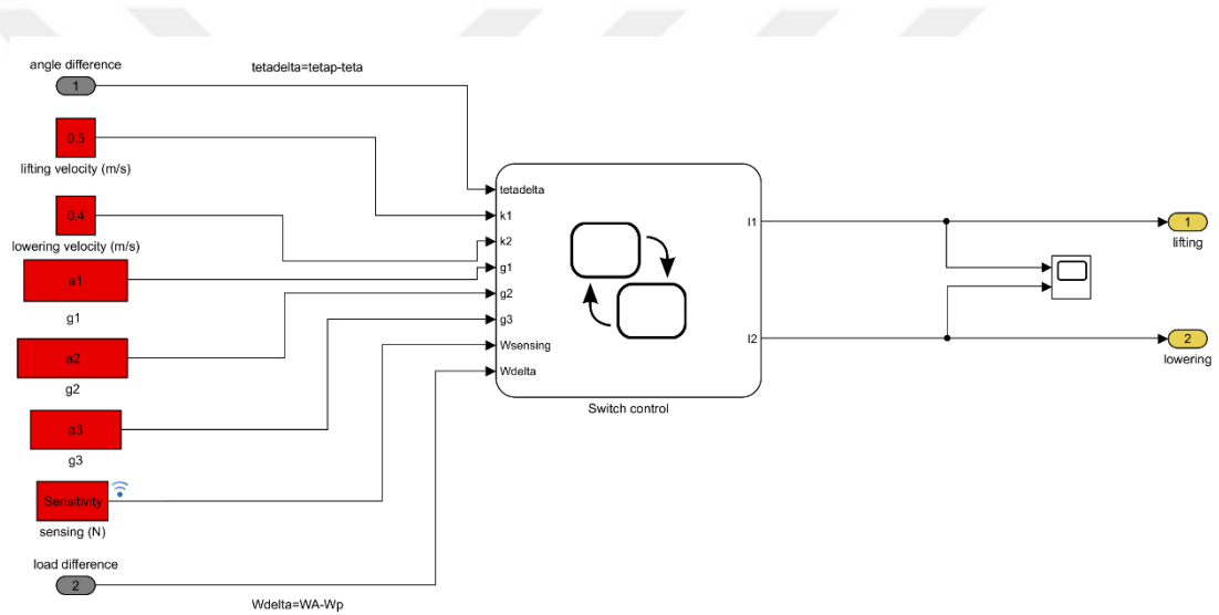
Figure 3.32. Detail view of the controller
