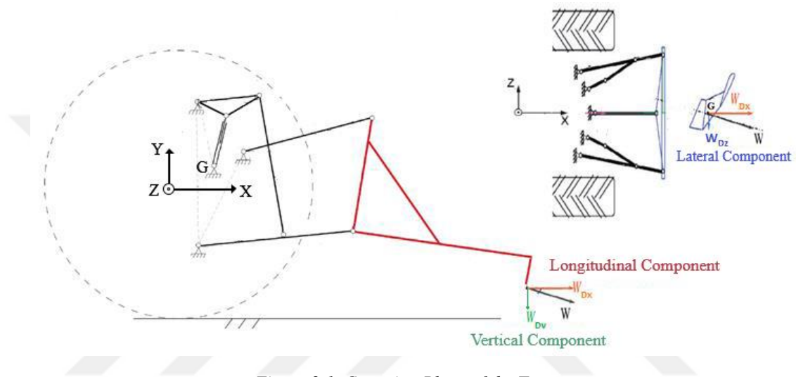
Figure 2.1. Cartesian Plane of the Tractor
