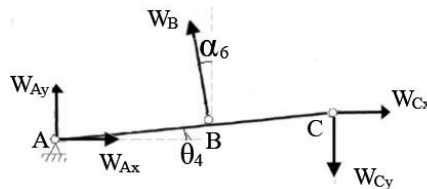
Figure 3.10. Force body diagram of the lower link
