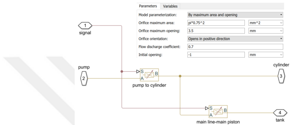
Figure 3.29. Simulink model of lifting module
