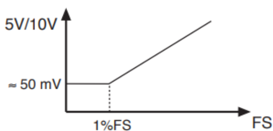
Figure 4.5. Characteristic of the pressure sensor [39]
