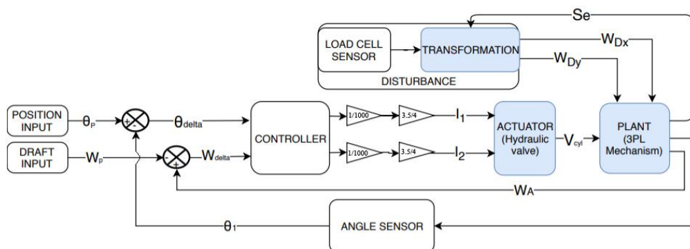
Figure 5.9. Current model block diagram
