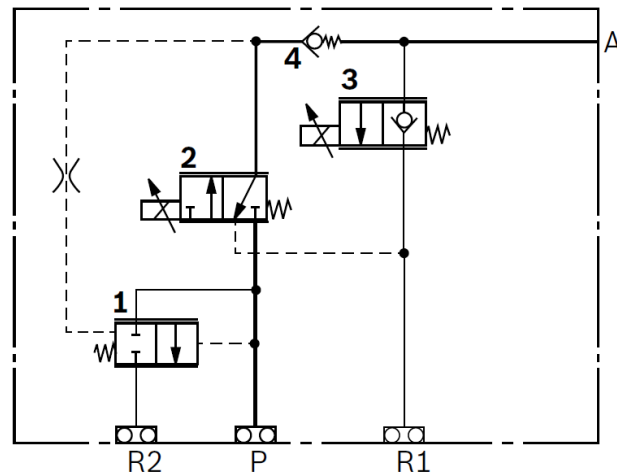
Figure 3.24. Hydraulic schema of the BOSCH EHR 5 valve [35]
