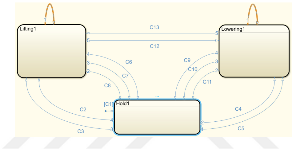
Figure 3.36. State flow conditions
