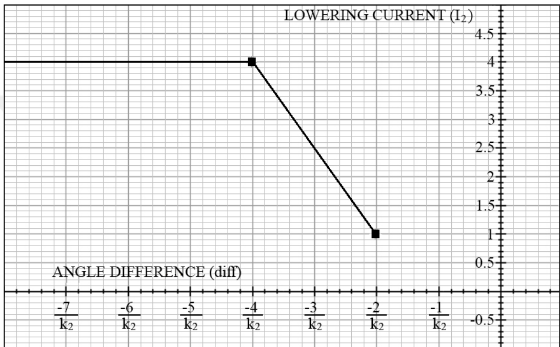
Figure 3.39. Position control characteristic of lowering module current wrt. angle difference
