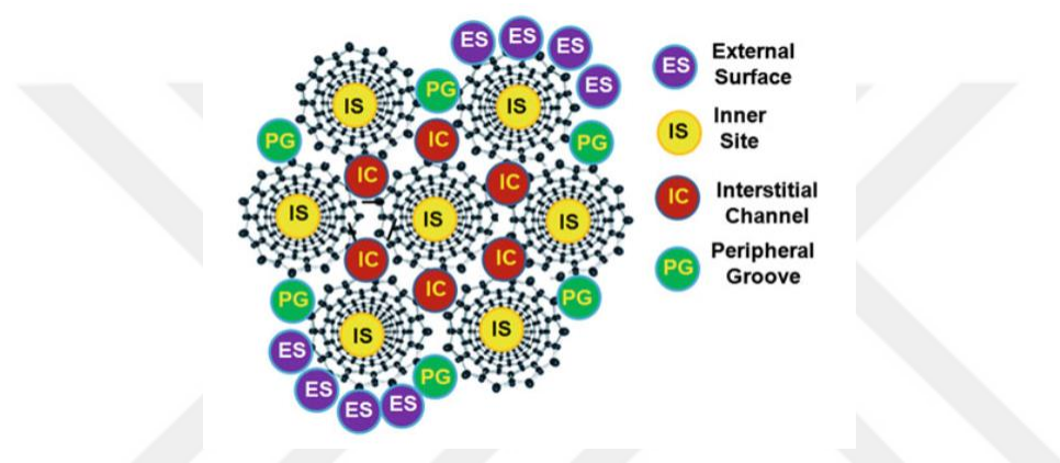
Figure 5. Structural Representation of Four Possible Major Adsorption Sites of CNT Bundle (Das, 2017)
