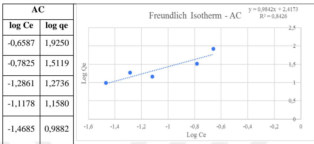
Figure 37. Freundlich Isotherm Graph of PAC
