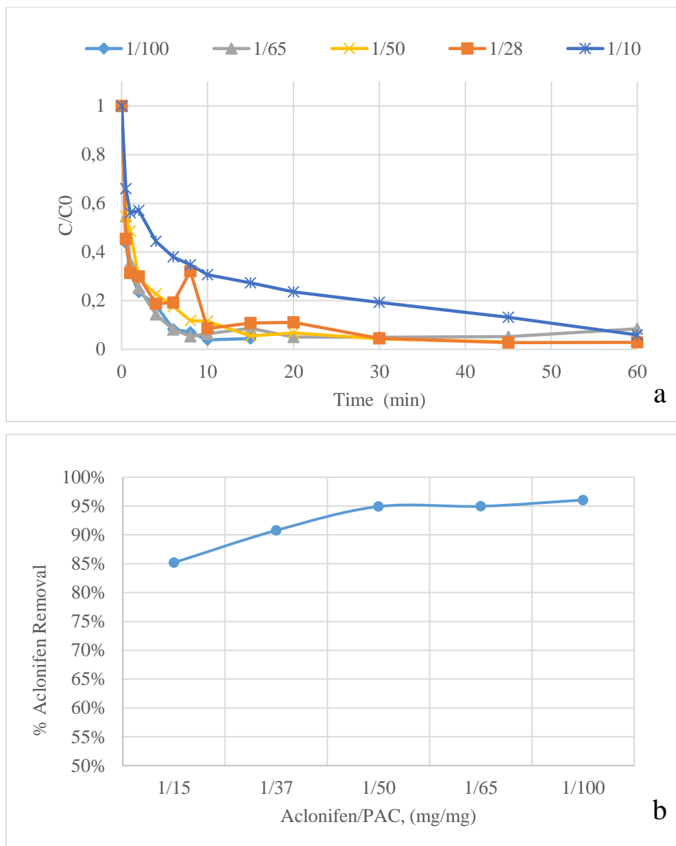
Figure 9. Removal of Aclonifen from Aqueous Solutions by PAC: (a) Time Course Variation of Aclonifen at Different Aclonifen/PAC Ratios; (b) % Aclonifen Removal vs Aclonifen/PAC Ratio
