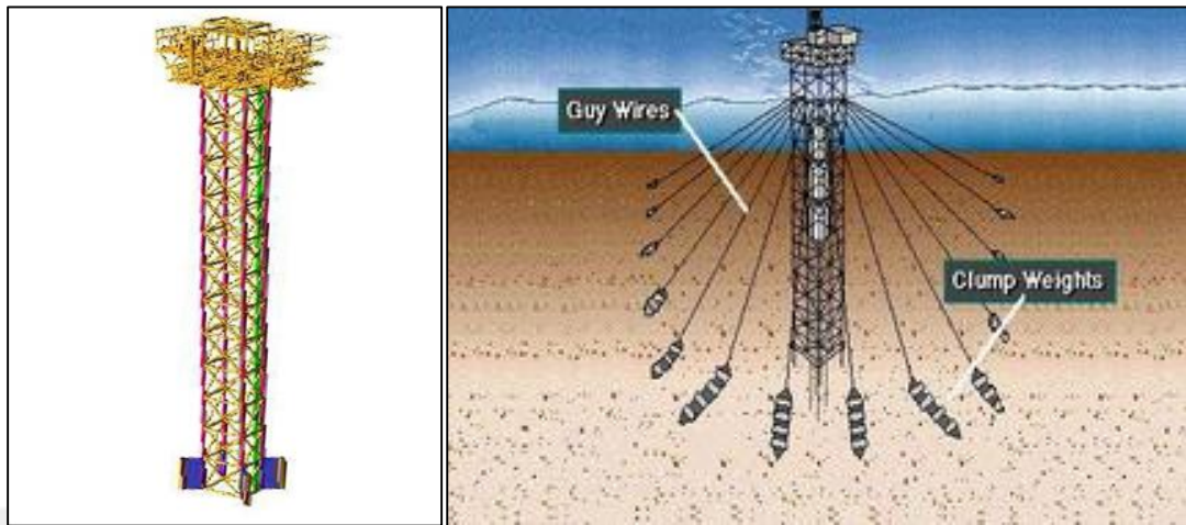
Figure 1.3. Examples of Compliant Tower and Guyed Tower
